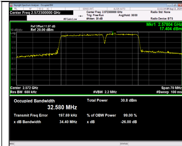
41-41-20MHz-15MHz-QPSK-QPSK-40340-40511-100RB #0-75RB#0-PASS
