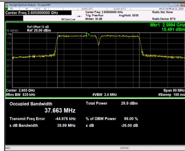
41-41-20MHz-20MHz-64QAM-64QAM-40641-40839-100RB #0-100RB#0-PASS
