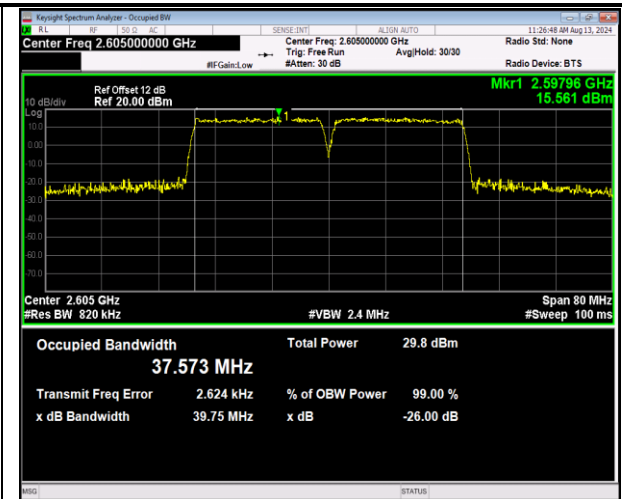
41-41-20MHz-20MHz-16QAM-16QAM-40641-40839-100RB #0-100RB#0-PASS
