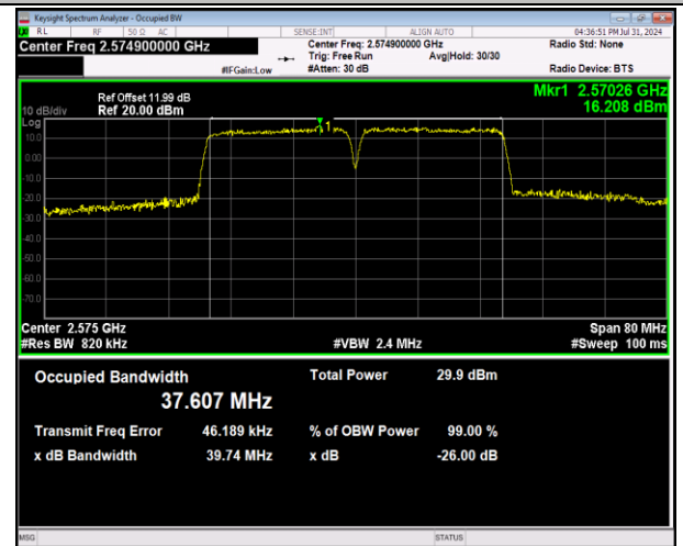
41-41-20MHz-20MHz-64QAM-64QAM-40340-40538-100RB #0-100RB#0-PASS
