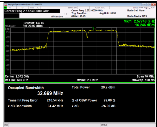
41-41-20MHz-15MHz-16QAM-16QAM-40340-40511-100RB #0-75RB#0-PASS
