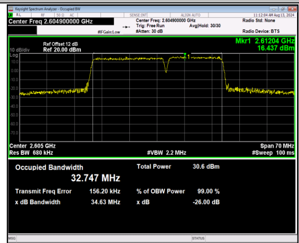
41-41-20MHz-15MHz-QPSK-QPSK-40666-40837-100RB #0-75RB#0-PASS
