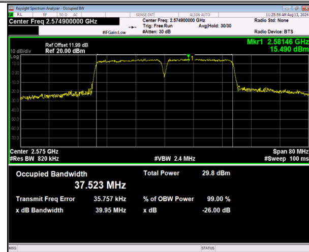
41-41-20MHz-20MHz-16QAM-16QAM-40340-40538-100RB #0-100RB#0-PASS
