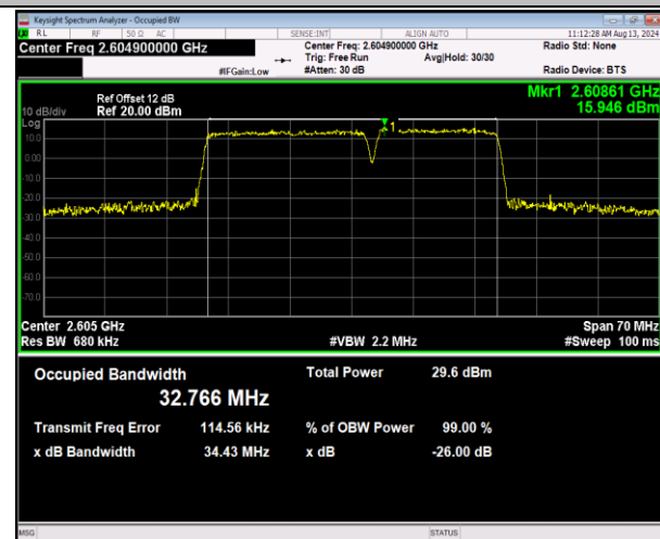
41-41-20MHz-15MHz-16QAM-16QAM-40666-40837-100RB #0-75RB#0-PASS
