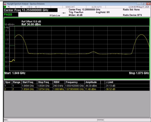
2-2-5MHz-20MHz-QPSK@QPSK-QPSK@QPSK-18633-1 8750-1RB#0@25RB#0-1RB#99@100RB#0-PASS
