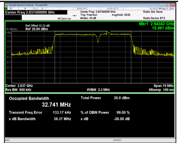
41-41-20MHz-15MHz-16QAM-16QAM-40991-41162-100RB #0-75RB#0-PASS
