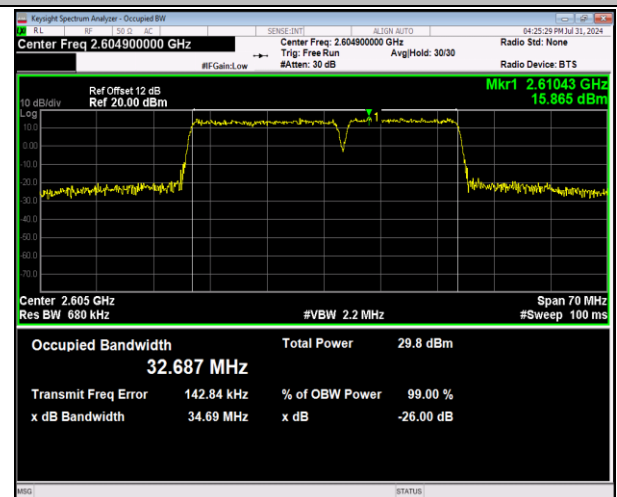
41-41-20MHz-15MHz-64QAM-64QAM-40666-40837-100RB #0-75RB#0-PASS
