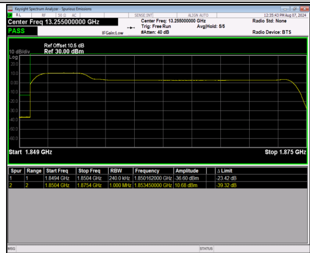
2-2-5MHz-20MHz-QPSK@QPSK-QPSK@QPSK-18633-1 8750-25RB#0@25RB#0-100RB#0@100RB#0-PASS
