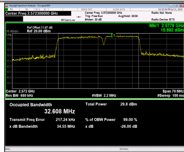
41-41-20MHz-15MHz-64QAM-64QAM-40340-40511-100RB #0-75RB#0-PASS
