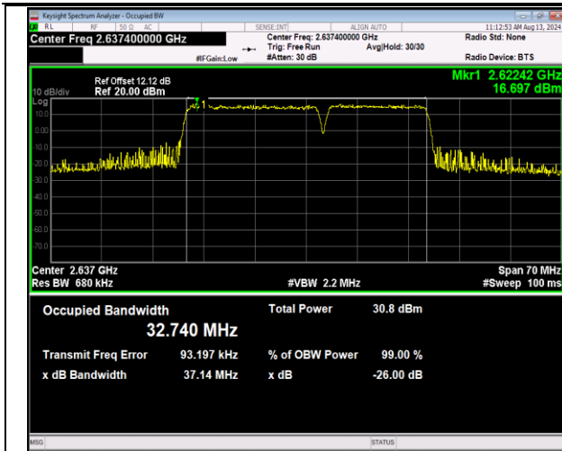
41-41-20MHz-15MHz-QPSK-QPSK-40991-41162-100RB #0-75RB#0-PASS
