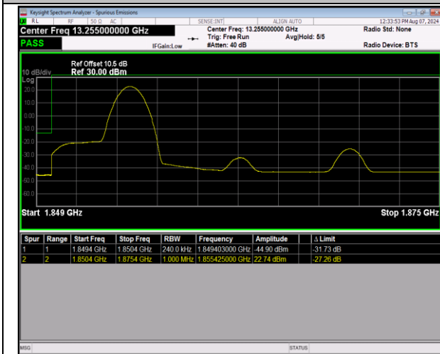
2-2-5MHz-20MHz-QPSK@QPSK-QPSK@QPSK-18633-1 8750-1RB#24@25RB#0-0RB#0@100RB#0-PASS
