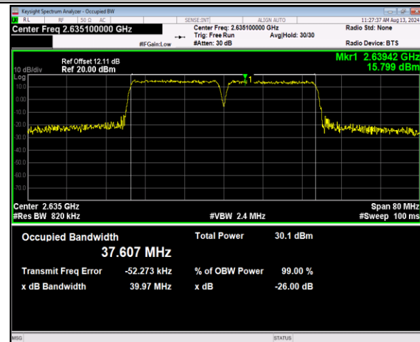
41-41-20MHz-20MHz-16QAM-16QAM-40942-41140-100RB #0-100RB#0-PASS
