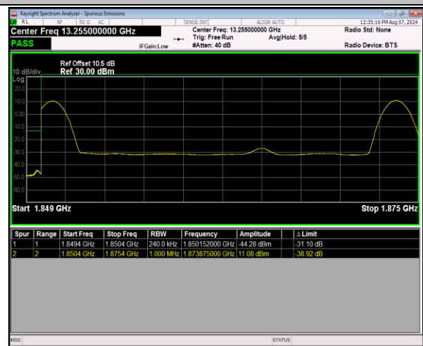
2-2-5MHz-20MHz-16QAM@16QAM-16QAM@16QAM-18
