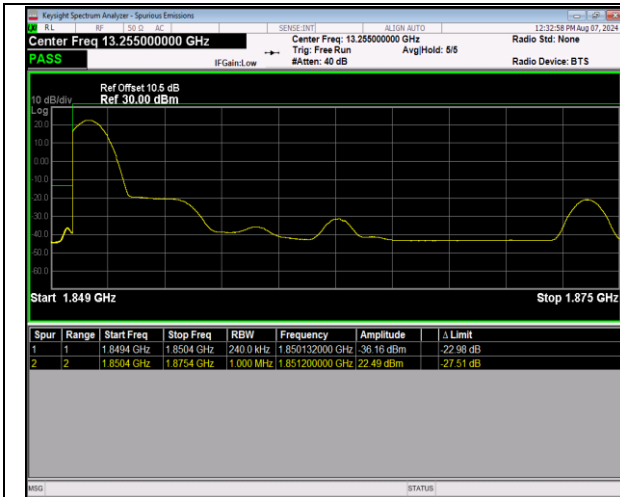
2-2-5MHz-20MHz-QPSK@QPSK-QPSK@QPSK-18633-1 8750-1RB#0@25RB#0-0RB#0@100RB#0-PASS
