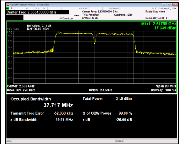
41-41-20MHz-20MHz-QPSK-QPSK-40942-41140-100RB #0-100RB#0-PASS
