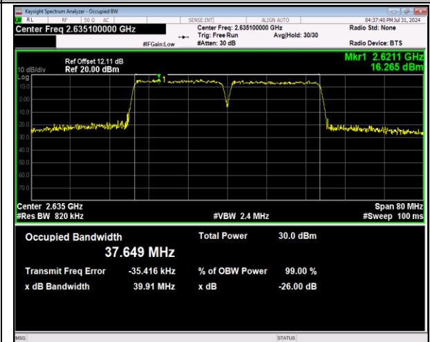
41-41-20MHz-20MHz-64QAM-64QAM-40942-41140-100RB #0-100RB#0-PASS
