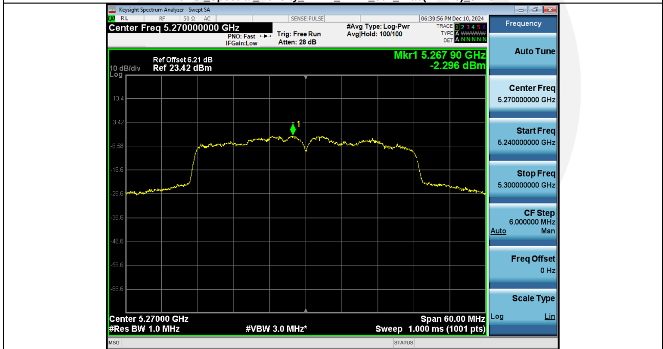
Power_Spectral_Density_NVNT_ANT2_802_11ac(VHT40)_5270
