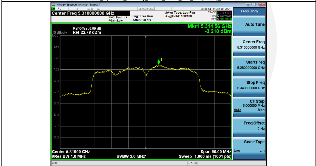
Power_Spectral_Density_NVNT_ANT2_802_11n(HT40)_5310
