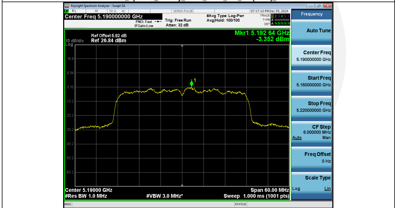
Power_Spectral_Density_NVNT_ANT2_802_11n(HT40)_5190
