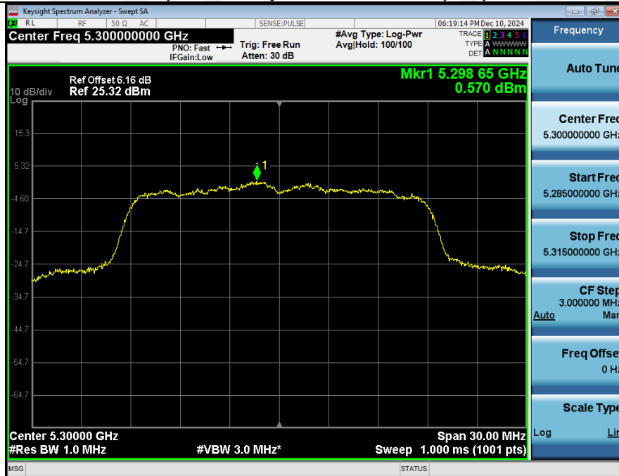
Power_Spectral_Density_NVNT_ANT2_802_11n(HT20)_5300
