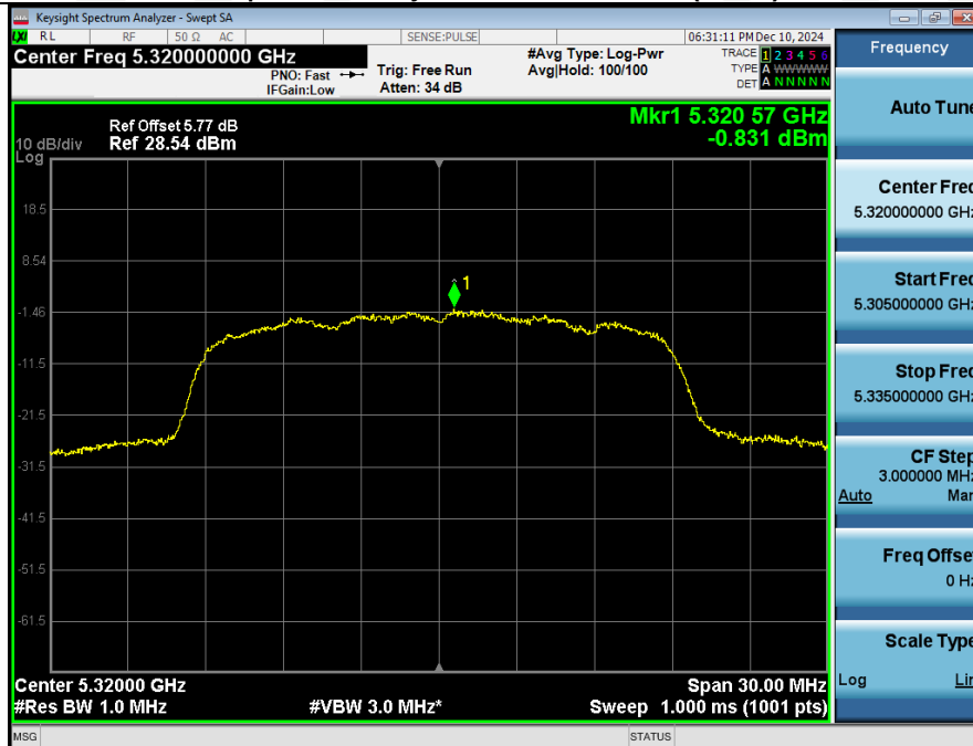
Power_Spectral_Density_NVNT_ANT2_802_11ac(VHT20)_5320
