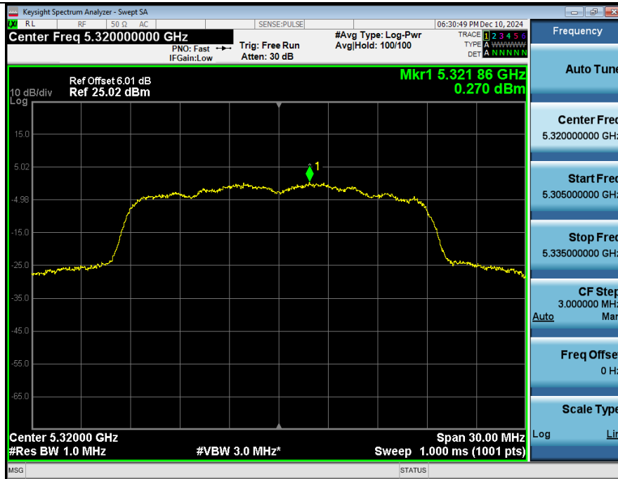
Power_Spectral_Density_NVNT_ANT2_802_11ac(VHT20)_5320
