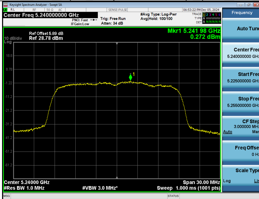
Power_Spectral_Density_NVNT_ANT2_802_11n(HT20)_5240
