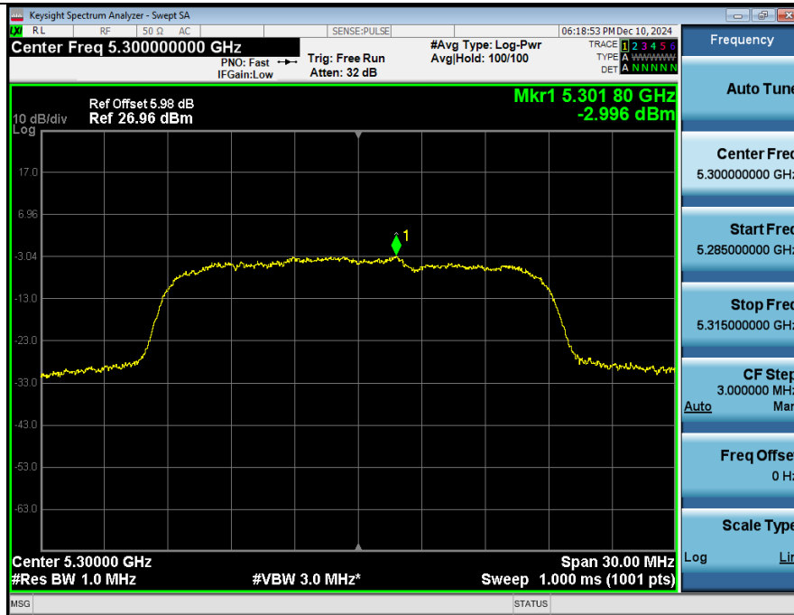
Power_Spectral_Density_NVNT_ANT2_802_11n(HT20)_5300
