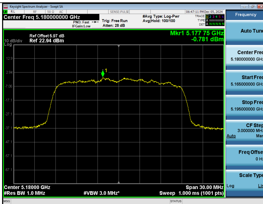
Power_Spectral_Density_NVNT_ANT2_802_11n(HT20)_5180
