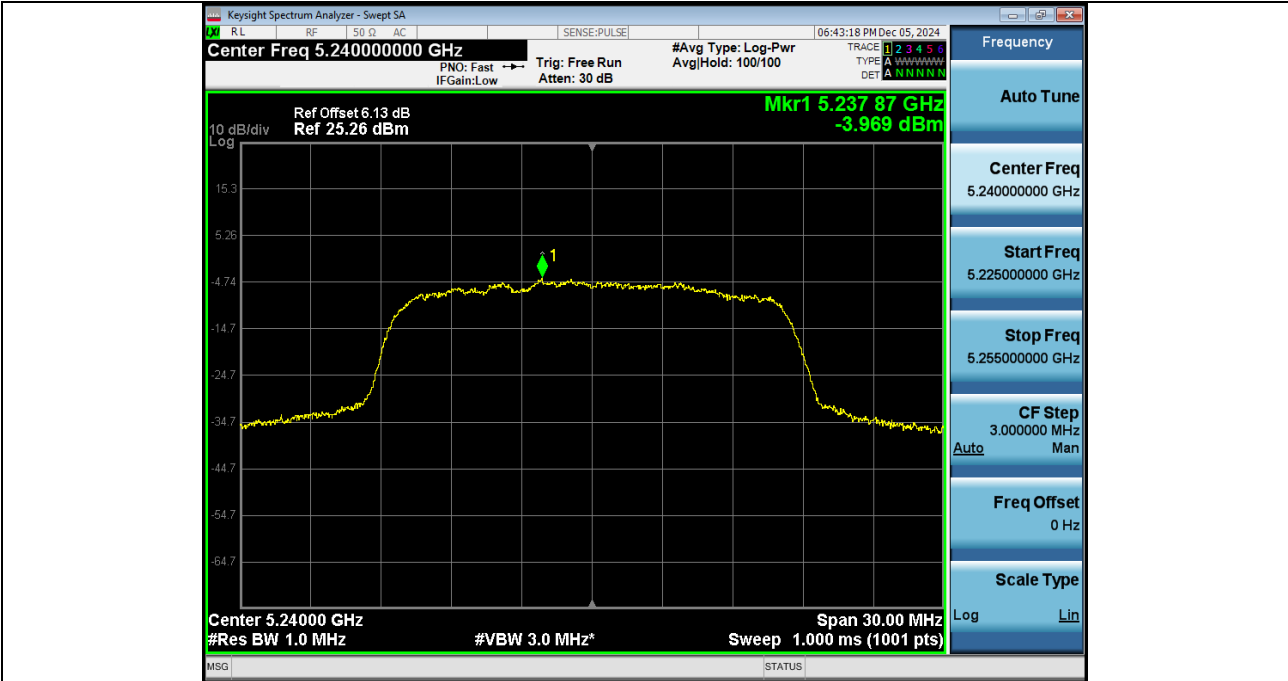
Power_Spectral_Density_NVNT_ANT2_802_11a_5240
