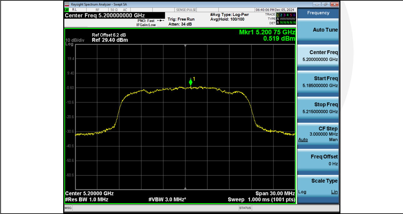
Power_Spectral_Density_NVNT_ANT2_802_11a_5200
