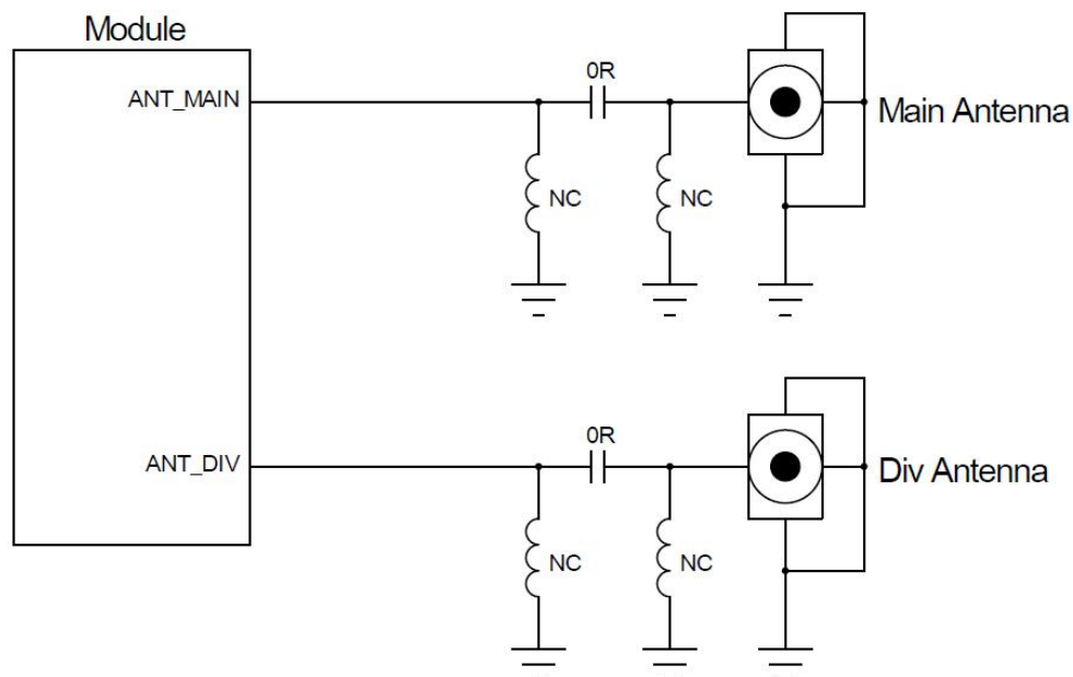
Figure 4-1 L816-AM Antenna \pi Circuit
