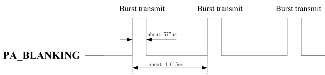
Figure 3-15 PA_Blanking Timing
