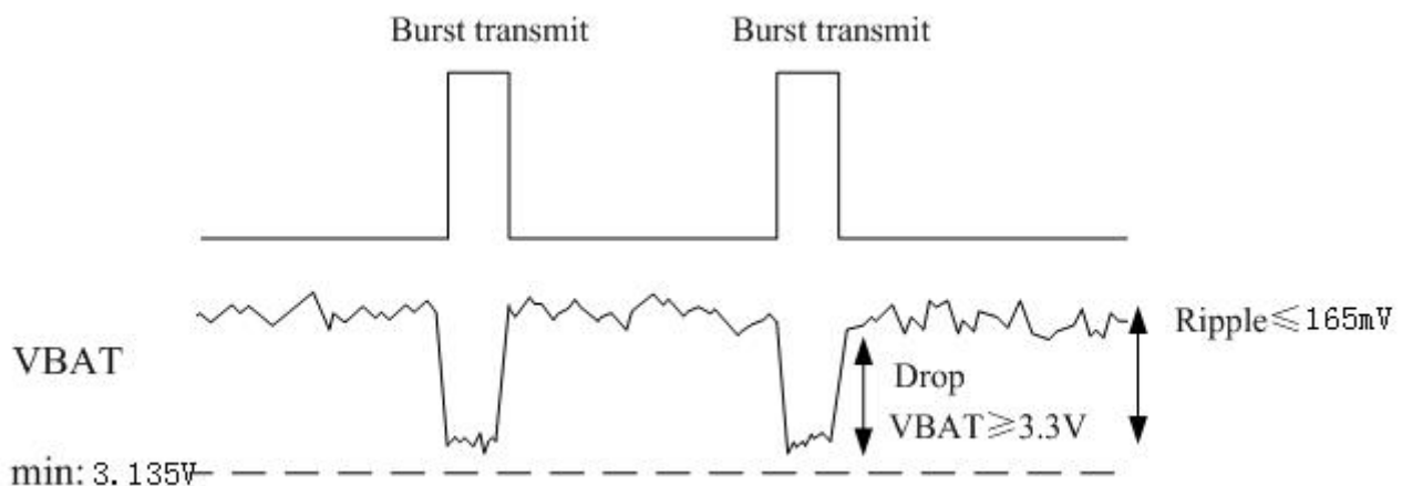
Figure 3-3 Power Supply Limit
