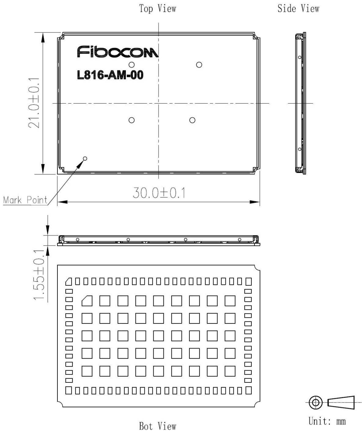
Figure 5-2 Dimension of Structure
