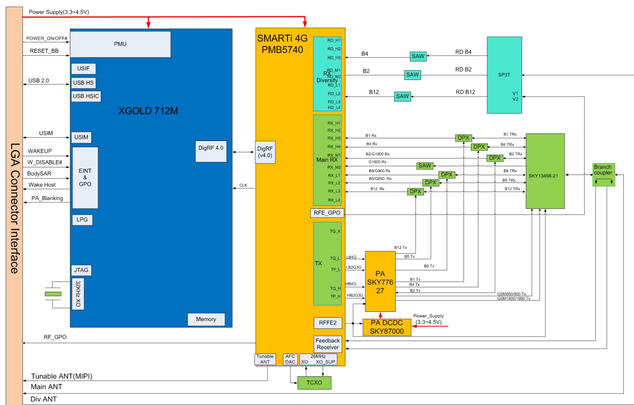
Figure 2-2 Hardware Framework
