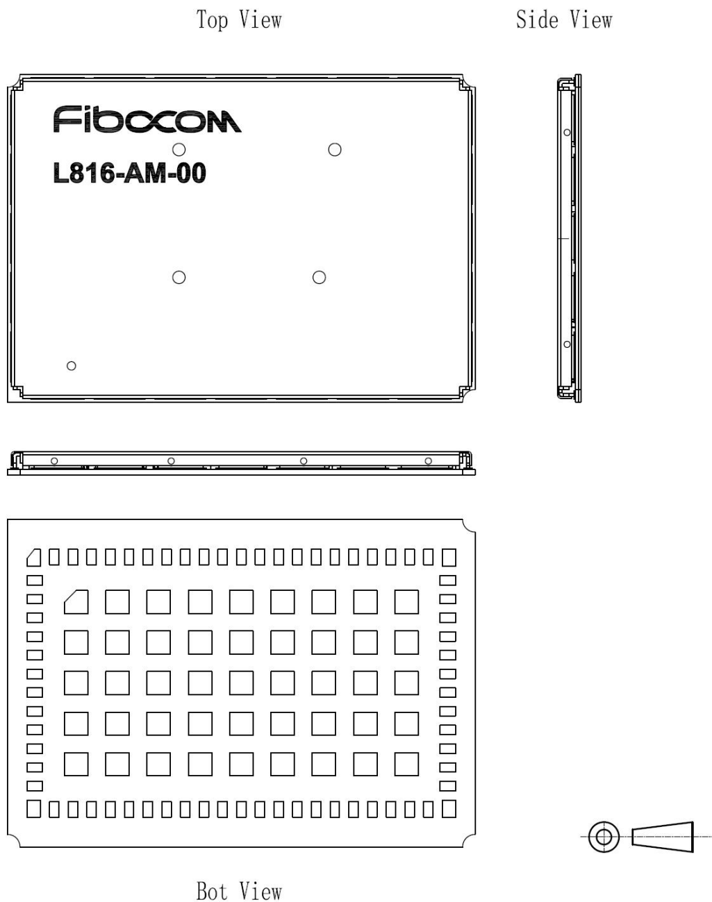
Figure 5-1 Module Appearance
