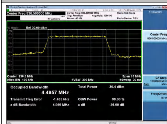
Band26(824-849)-5MHz-QPSK-26915-25RB#0-P
