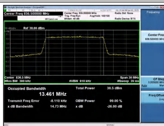
Band26(824-849)-15MHz-16QAM-26915-75RB#0- PASS
