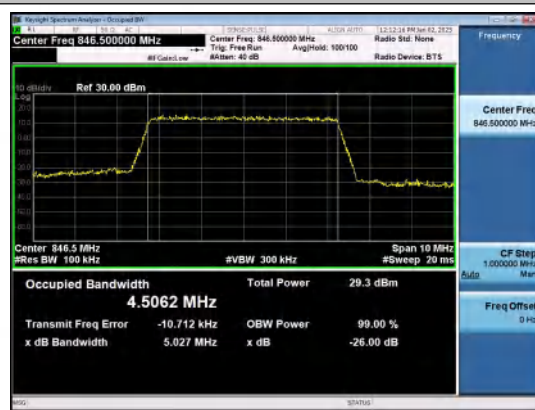
Band26(824-849)-5MHz-16QAM-27015-25RB#0-P
