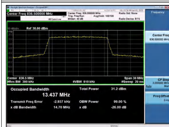
Band26(824-849)-15MHz-QPSK-26915-75RB#0- PASS
