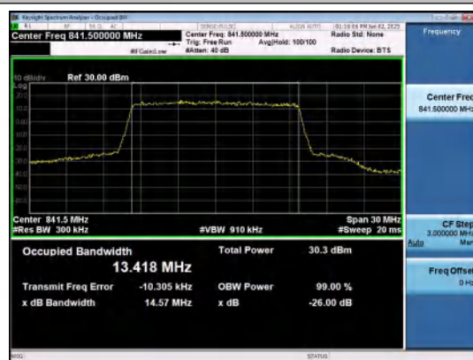
Band26(824-849)-15MHz-16QAM-26965-75RB#0- PASS
