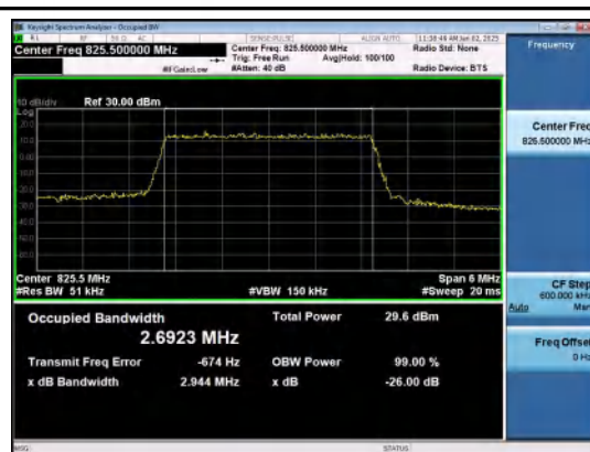
Band26(824-849)-3MHz-16QAM-26805-15RB#0-P ASS
