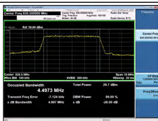
Band26(824-849)-5MHz-16QAM-26815-25RB#0-P
