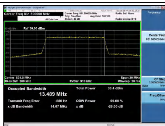
Band26(824-849)-15MHz-16QAM-26865-75RB#0- PASS
