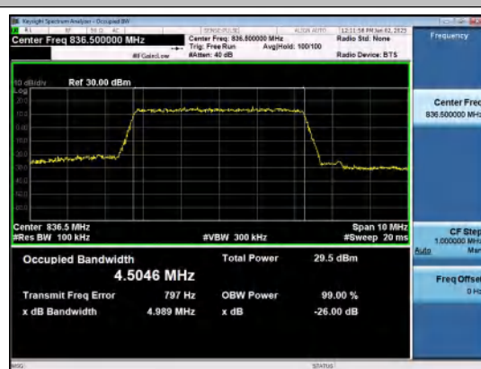
Band26(824-849)-5MHz-16QAM-26915-25RB#0-P
