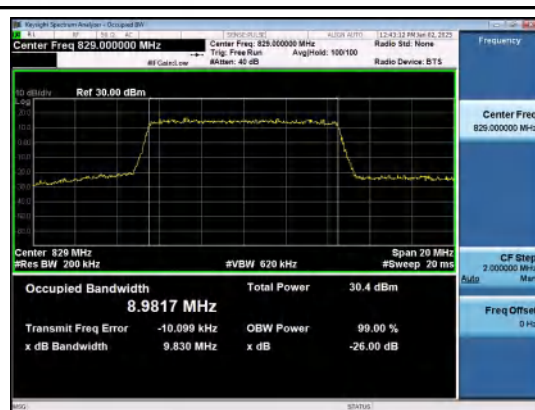
Band26(824-849)-10MHz-16QAM-26840-50RB#0-PASS
