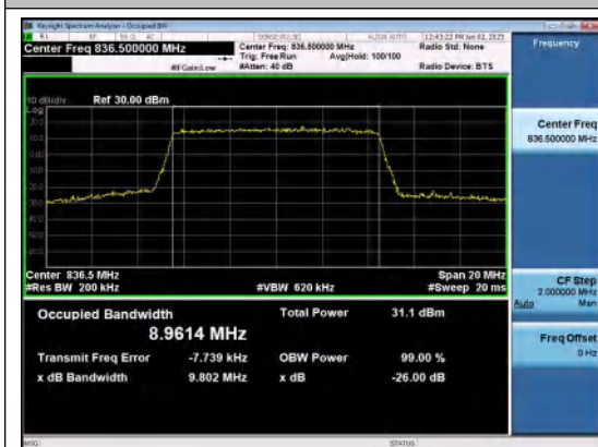
Band26(824-849)-10MHz-QPSK-26915-50RB#0-PASS
