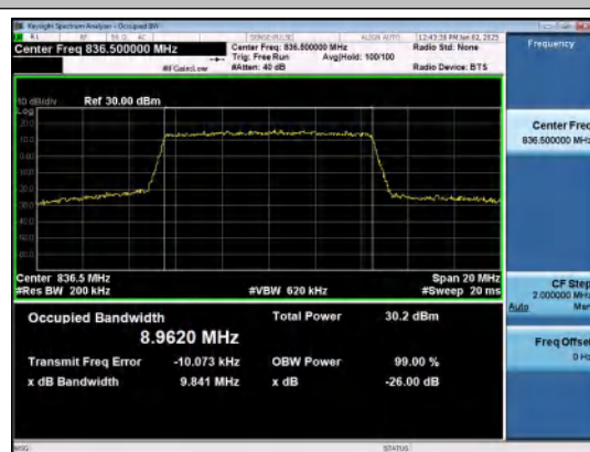
Band26(824-849)-10MHz-16QAM-26915-50RB#0-PASS
