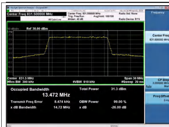
Band26(824-849)-15MHz-QPSK-26865-75RB#0- PASS
