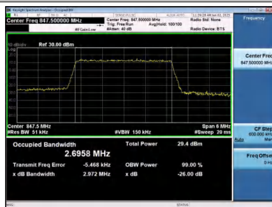
Band26(824-849)-3MHz-16QAM-27025-15RB#0-P ASS
