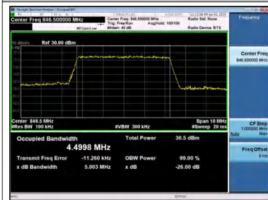
Band26(824-849)-5MHz-QPSK-27015-25RB#0-P
