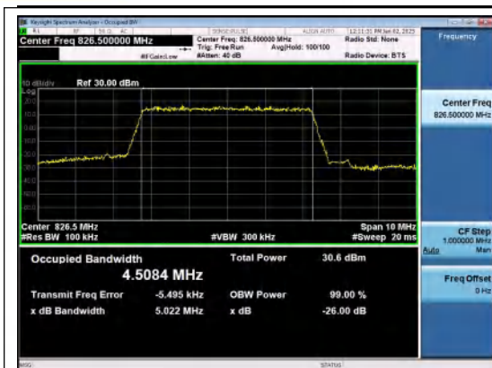
Band26(824-849)-5MHz-QPSK-26815-25RB#0-P
