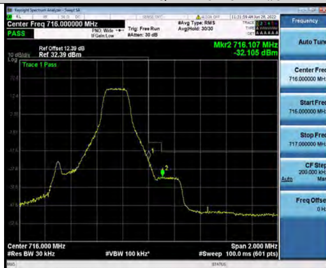
Band12-1.4MHz-QPSK-23173-1RB#5
