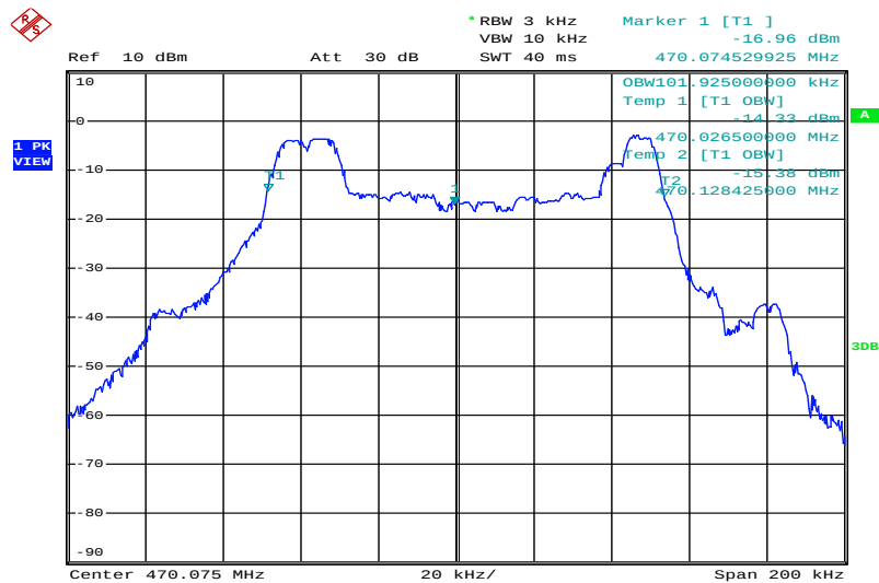
Plot 1: lowest channel, 1 kHz tone
