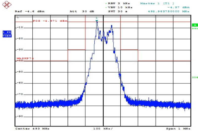
Plot 6: middle channel, spectrum mask
