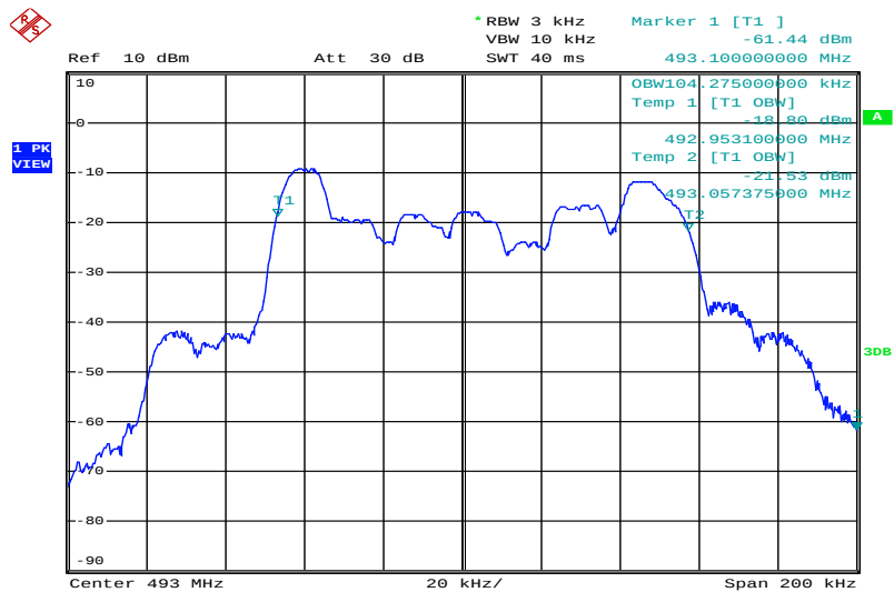
Plot 5: middle channel, 2.5 kHz tone
