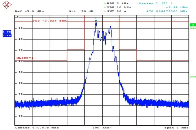
Plot 3: lowest channel, spectrum mask
