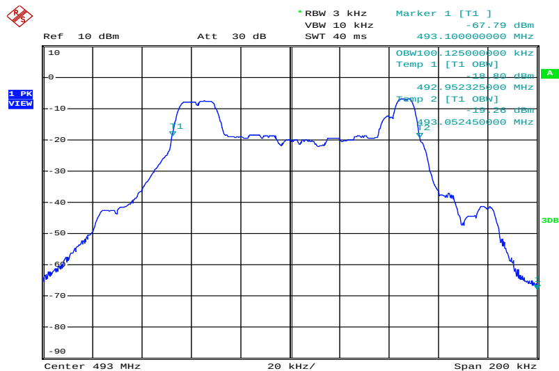
Plot 2: middle channel, 1 kHz tone
