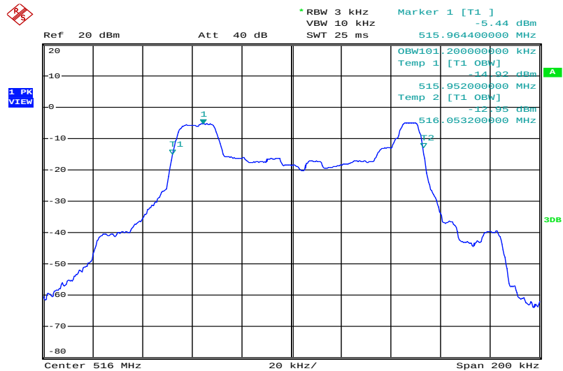
Plot 3: highest channel, 1 kHz tone
