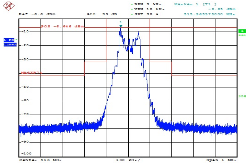
Plot 9: highest channel, spectrum mask
