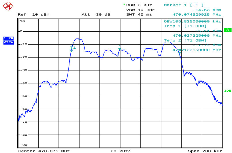
Plot 4: lowest channel, 2.5 kHz tone
