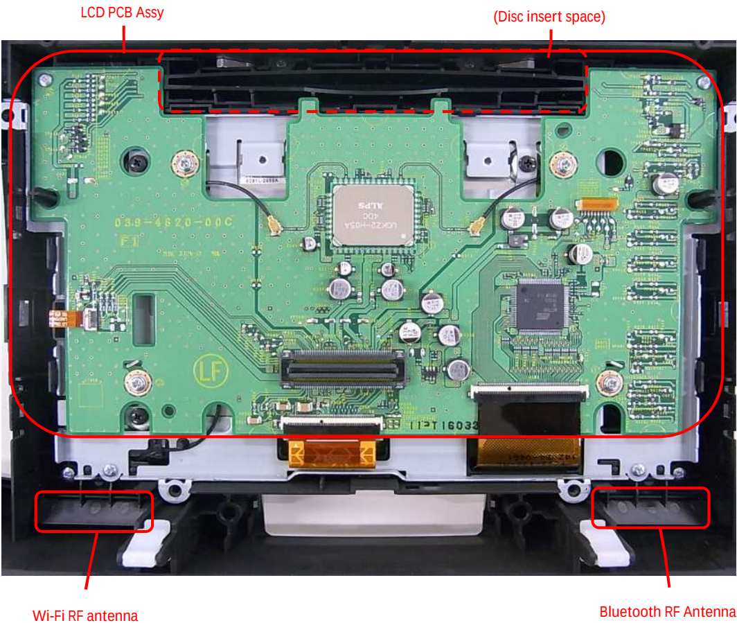
1-2. LCD PCB ASSY - F1 View (more detail)
