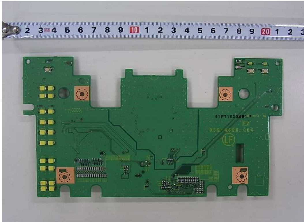
1-3. LCD PCB ASSY - F2 View
