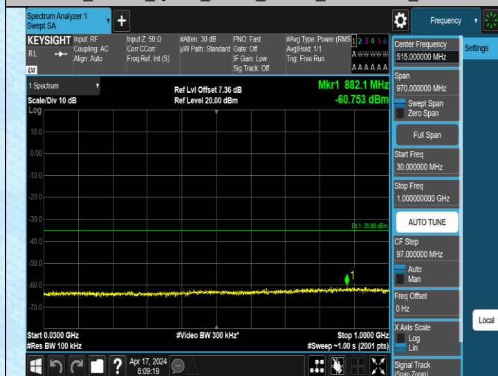
Band38_15MHz_QPSK_37825_1RB#0_30~1000_30~1000
