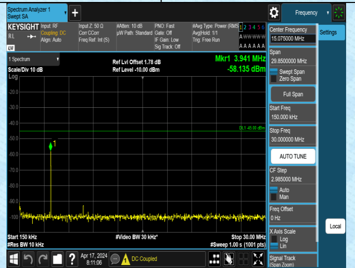
Band38_15MHz_QPSK_38000_1RB#0_0.15~30_0.15~30
