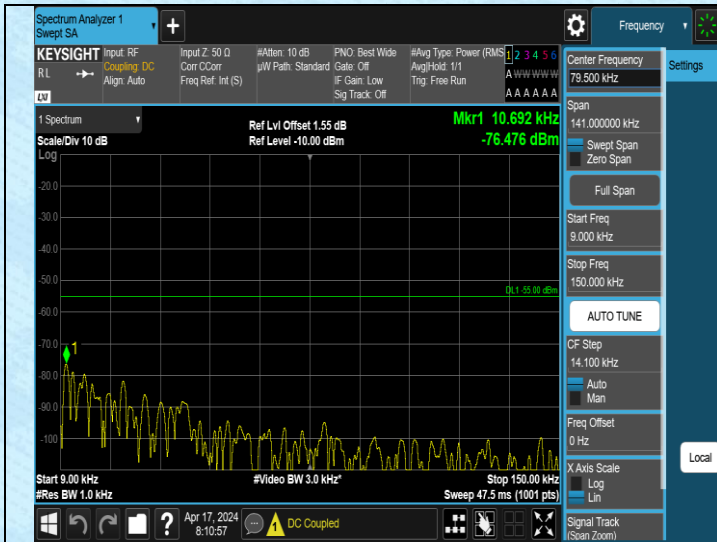
Band38_15MHz_QPSK_38000_1RB#0_0.009~0.15_0.009~0.15
