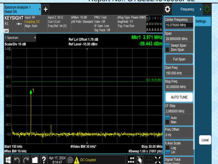
Band38_20MHz_QPSK_37850_1RB#0_0.15~30_0.15~30
