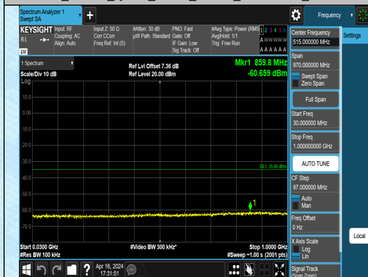
Band38_10MHz_QPSK_37800_1RB#0_30~1000_30~1000
