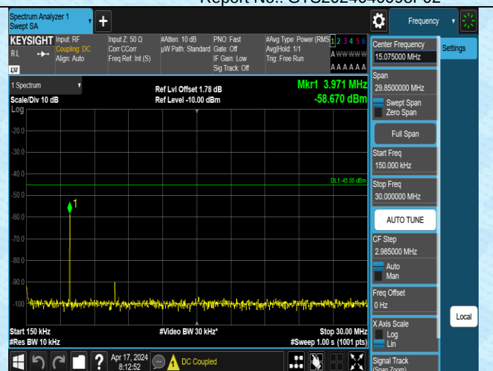
Band38_15MHz_QPSK_38175_1RB#0_0.15~30_0.15~30
