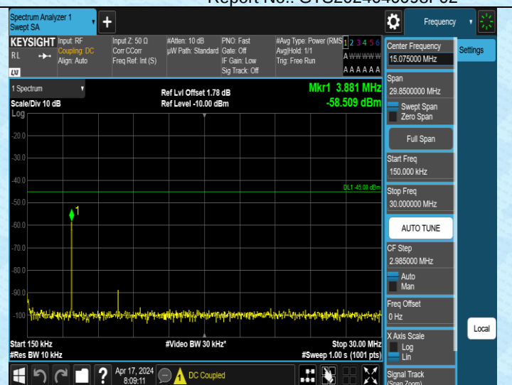
Band38_15MHz_QPSK_37825_1RB#0_0.15~30_0.15~30
