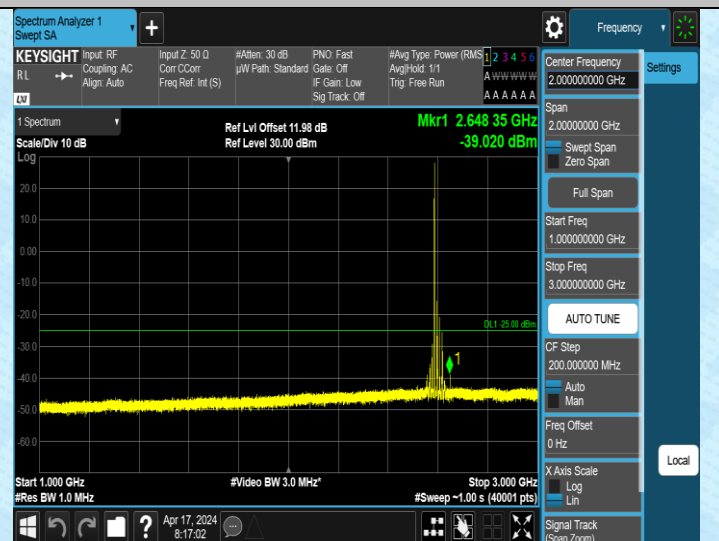
Band38_20MHz_QPSK_38000_1RB#0_1000~3000_1000~3000
