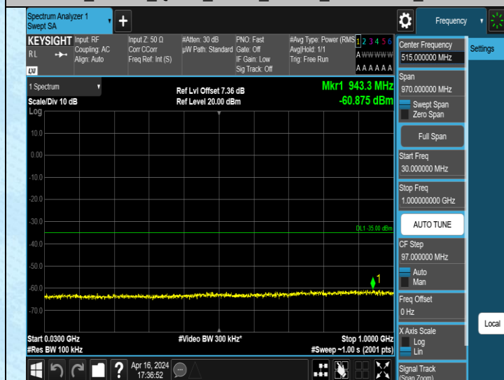
Band38_10MHz_QPSK_38200_1RB#0_30~1000_30~1000
