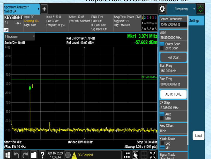
Band38_10MHz_QPSK_38200_1RB#0_0.15~30_0.15~30
