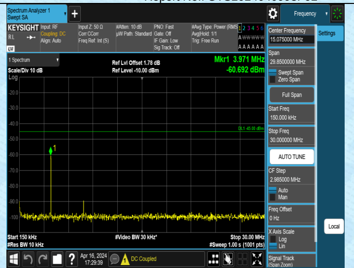
Band38_5MHz_QPSK_38225_1RB#0_0.15~30_0.15~30
