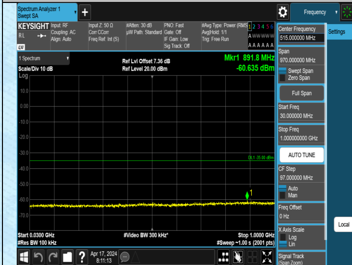
Band38_15MHz_QPSK_38000_1RB#0_30~1000_30~1000
