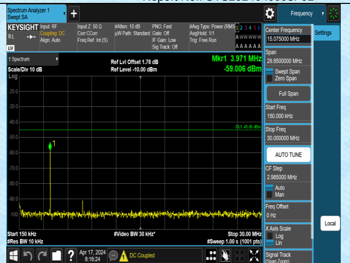
Band38_20MHz_QPSK_38000_1RB#0_0.15~30_0.15~30
