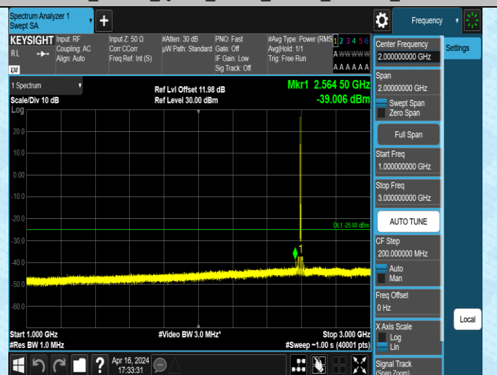
Band38_10MHz_QPSK_38000_1RB#0_1000~3000_1000~3000
