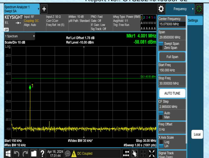
Band38_10MHz_QPSK_37800_1RB#0_0.15~30_0.15~30
