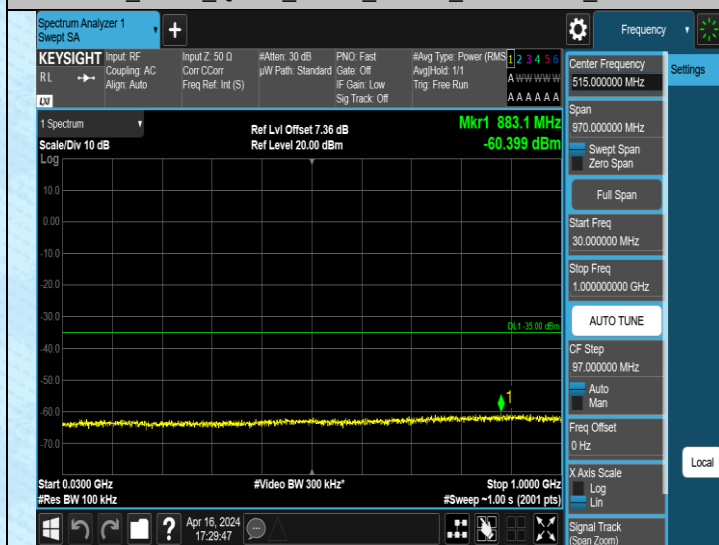
Band38_5MHz_QPSK_38225_1RB#0_30~1000_30~1000
