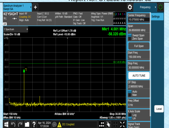
Band38_10MHz_QPSK_38000_1RB#0_0.15~30_0.15~30
