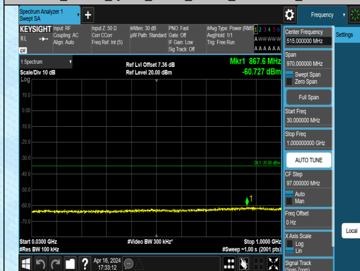
Band38_10MHz_QPSK_38000_1RB#0_30~1000_30~1000
