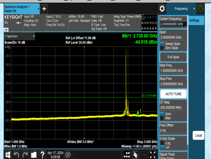
Band38_15MHz_QPSK_37825_1RB#0_1000~3000_1000~3000
