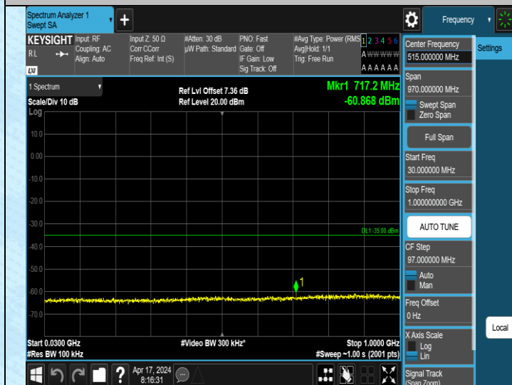
Band38_20MHz_QPSK_38000_1RB#0_30~1000_30~1000
