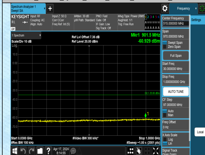
Band38_20MHz_QPSK_37850_1RB#0_30~1000_30~1000
