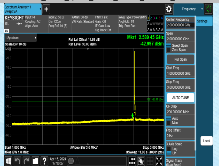
Band38_5MHz_QPSK_38225_1RB#0_1000~3000_1000~3000
