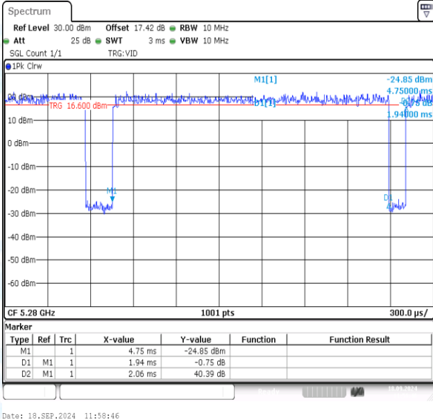
NTNV-11AC20MIMO-Ant1-5280
