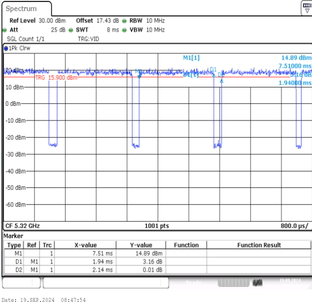
NTNV-11AC20MIMO-Ant1-5320
