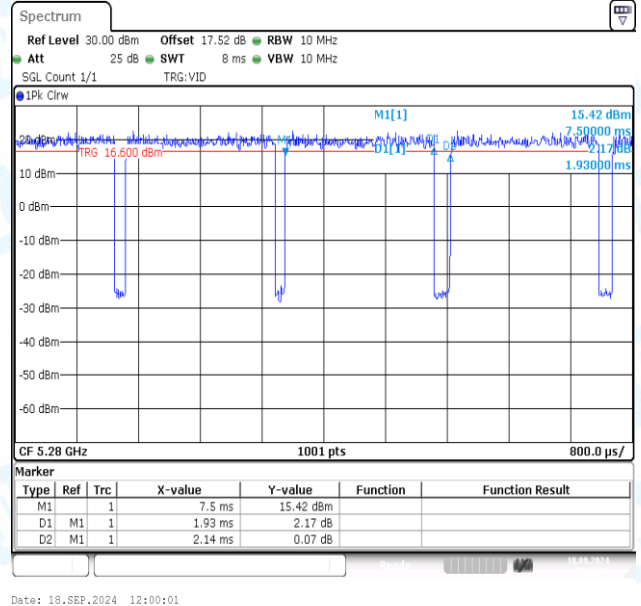
NTNV-11AC20MIMO-Ant2-5280
