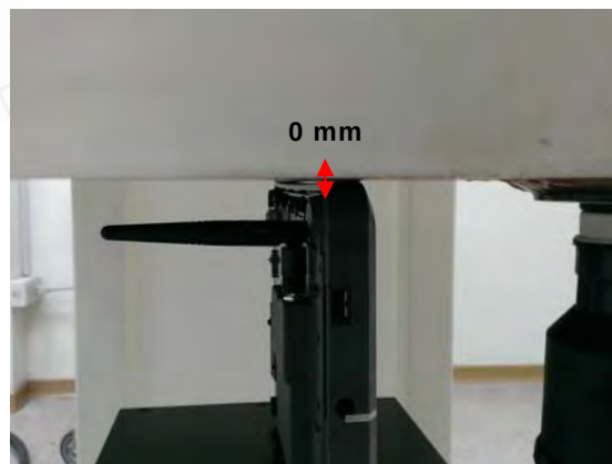
Fig.8 EUT Top side with transceiver to flat phantom
