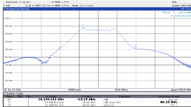
Figure 8.2-17: 26 dB OBW Middle channel: 16.15 GHz, shortest pulse (50 MHz BW)
