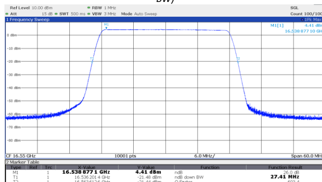
Figure 8.2-3: 26 dB OBW High channel: 16.55 GHz, longest pulse (25 MHz BW)
