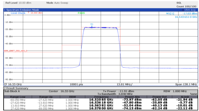
Figure 8.4-8: Emission mask, High channel: 16.55 GHz, longest pulse. (25 MHz BW)
