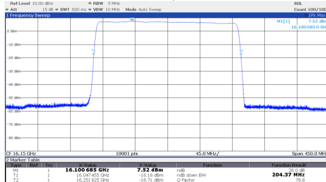
Figure 8.2-11: 26 dB OBW Middle channel: 16.15 GHz, longest pulse (200 MHz BW)
