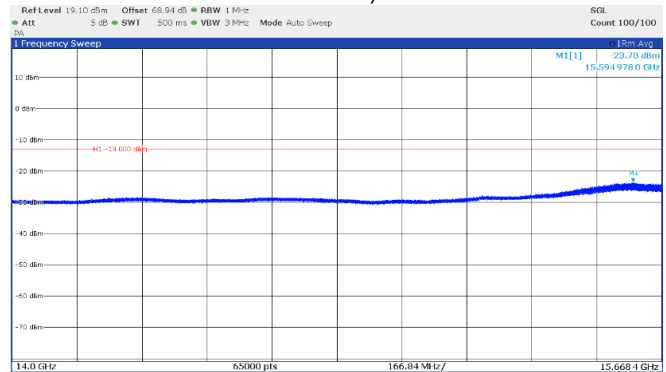
Figure 8.4-10: Emission mask, beyond \pm 250\% of BW (low frequency range), Low channel: 15.80 GHz, longest pulse. (50 MHz BW)
