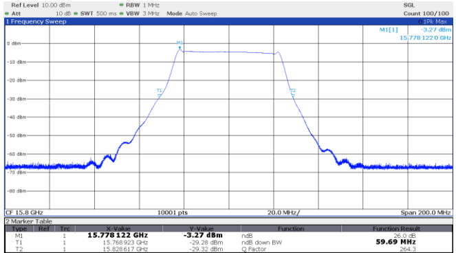
Figure 8.2-16: 26 dB OBW Low channel: 15.80 GHz, shortest pulse (50 MHz BW)
