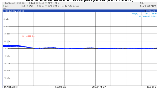
Figure 8.4-12: Emission mask, beyond \pm 250\% of BW (high frequency range), Low channel: 15.80 GHz, longest pulse. (50 MHz BW)
