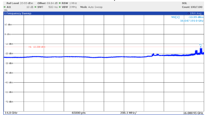
Figure 8.4-4: Emission mask, beyond \pm 250\% of BW (low frequency range), Middle channel: 16.15 GHz, longest pulse. (25 MHz BW)
