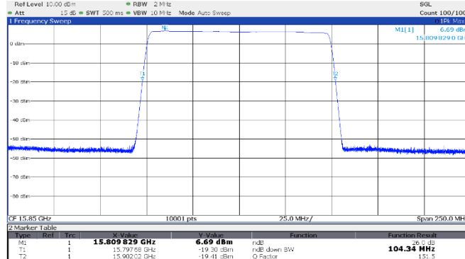
Figure 8.2-7: 26 dB OBW Low channel: 15.85 GHz, longest pulse (100 MHz BW)
