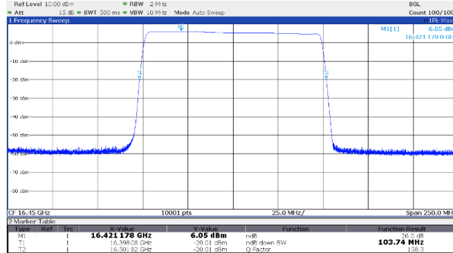
Figure 8.2-9: 26 dB OBW High channel: 16.45 GHz, longest pulse (100 MHz BW)
