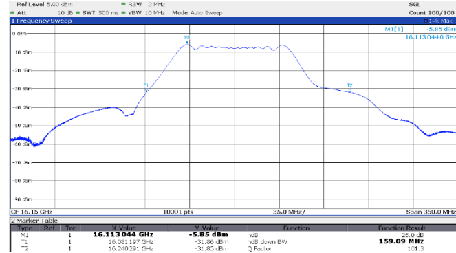
Figure 8.2-20: 26 dB OBW Middle channel: 16.15 GHz, shortest pulse (100 MHz BW)
