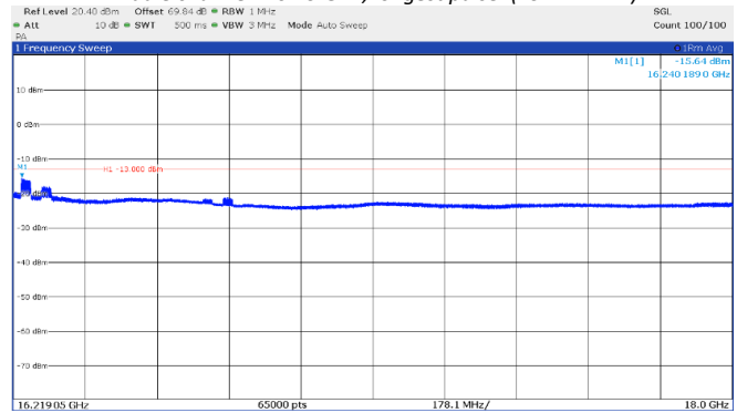
Figure 8.4-6: Emission mask, beyond \pm 250\% of BW (high frequency range), Middle channel: 16.15 GHz, longest pulse. (25 MHz BW)
