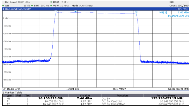
Figure 8.1-11: 99% OBW Middle channel: 16.15 GHz, longest pulse (200 MHz BW)
