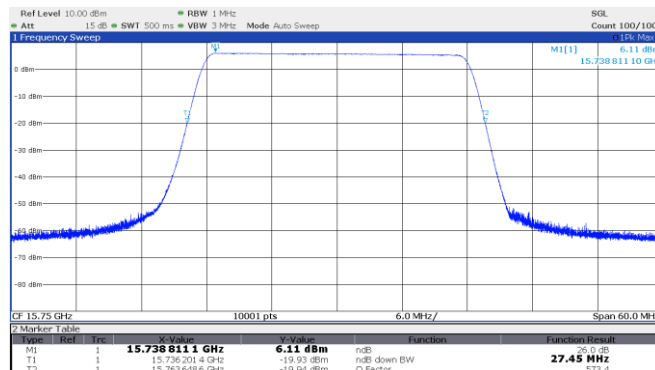
Figure 8.2-1: 26 dB OBW Low channel: 15.75 GHz, longest pulse (25 MHz BW)
