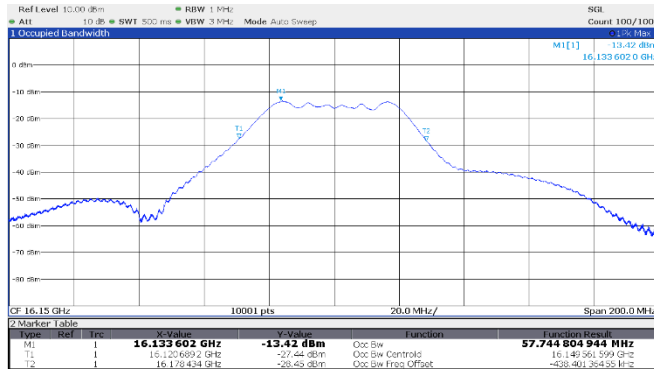
Figure 8.1-17: 99% OBW Middle channel: 16.15 GHz, shortest pulse (50 MHz BW)
