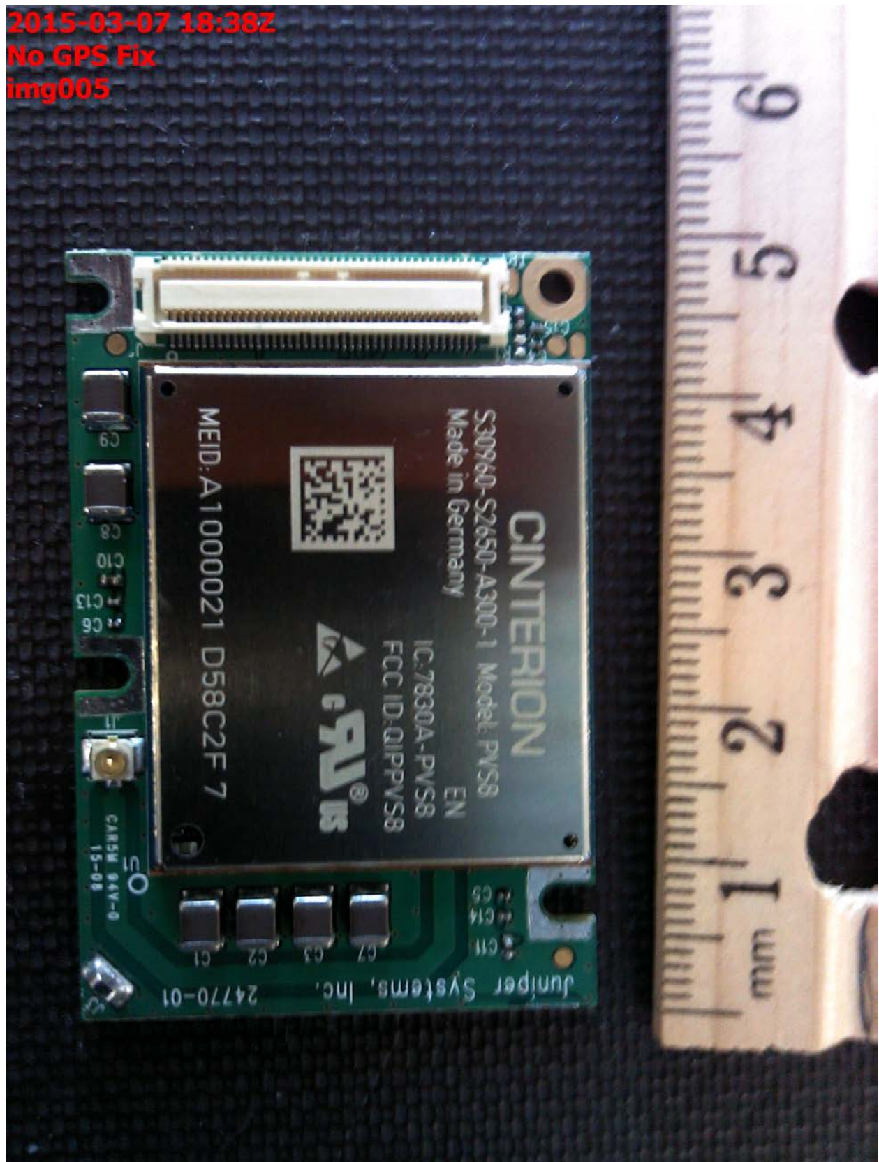
Figure 1: Module – Front View
