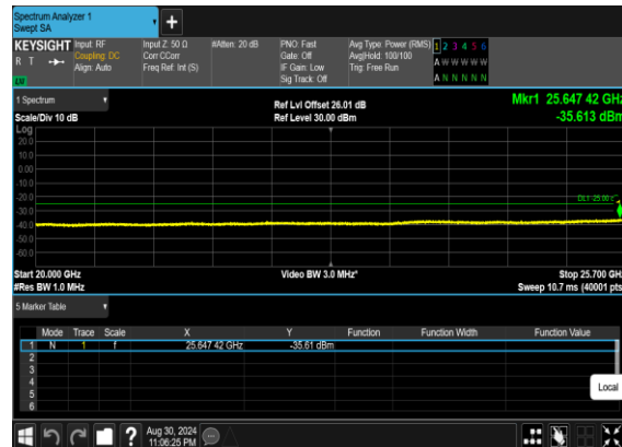
N7(25M)_DFT-s- OFDM_QPSK_Edge_1RB_Left_Low_CH
