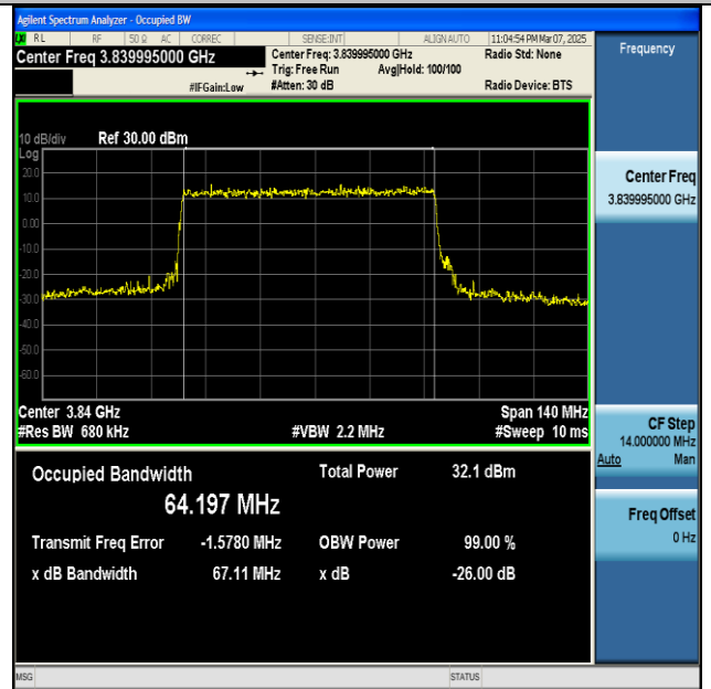
NTNV-n77(3700-3980)-PC2-30-70-M-DFT-256QAM- Outer_Full-Ant1-PASS
