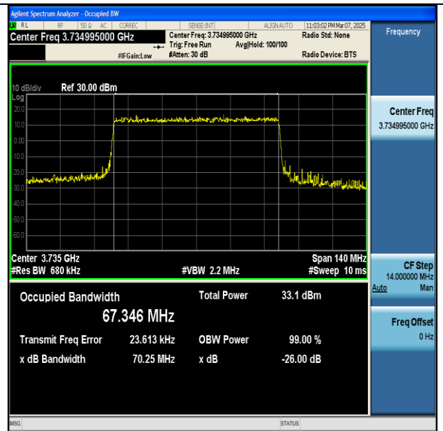
NTNV-n77(3700-3980)-PC2-30-70-L-CP-64QAM- Outer_Full-Ant1-PASS
