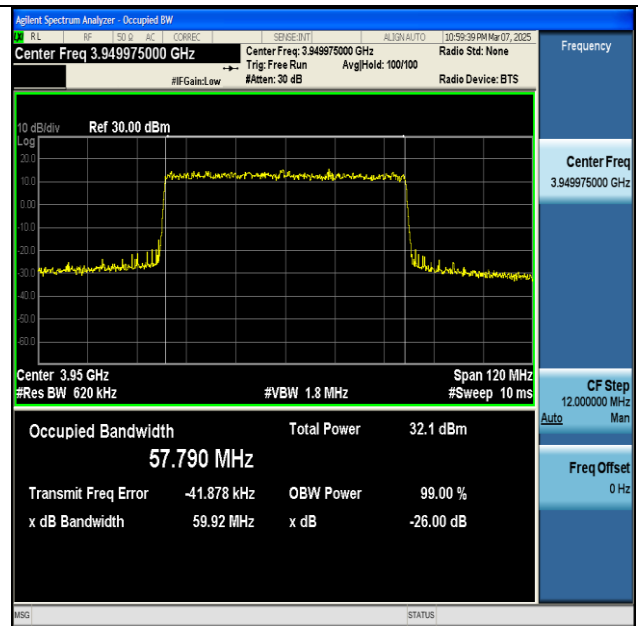
NTNV-n77(3700-3980)-PC2-30-60-H-DFT-256QAM- Outer_Full-Ant1-PASS
