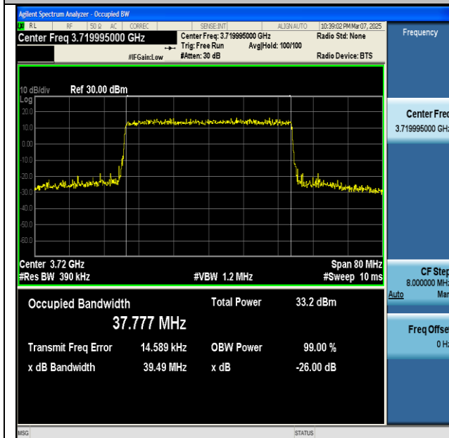
NTNV-n77(3700-3980)-PC2-30-40-L-CP-QPSK- Outer_Full-Ant1-PASS
