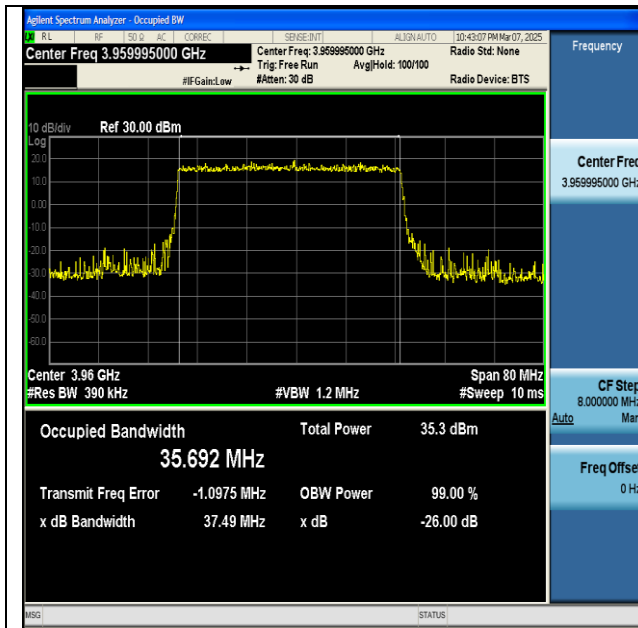
NTNV-n77(3700-3980)-PC2-30-40-H-DFT-QPSK- Outer_Full-Ant1-PASS
