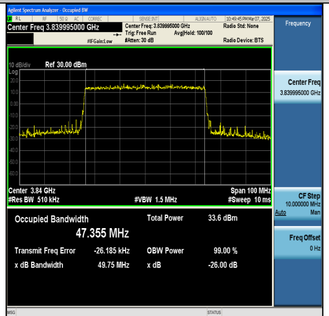
NTNV-n77(3700-3980)-PC2-30-50-M-CP-16QAM- Outer_Full-Ant1-PASS
