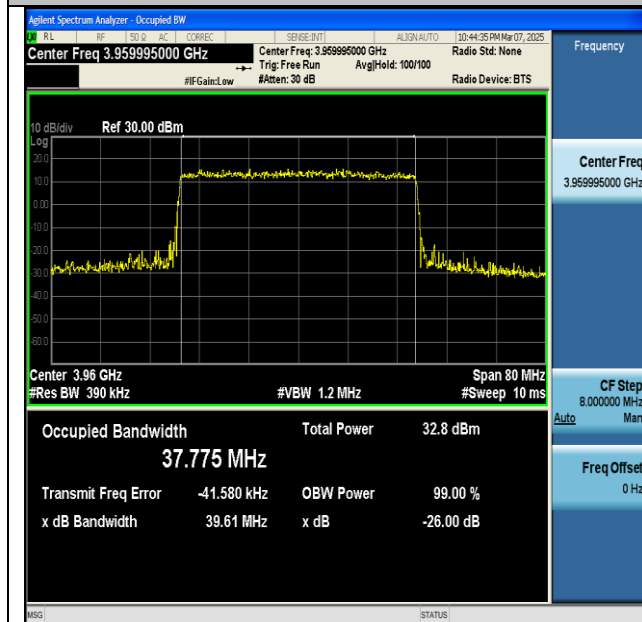
NTNV-n77(3700-3980)-PC2-30-40-H-CP-64QAM-Outer_Full-Ant1-PASS
