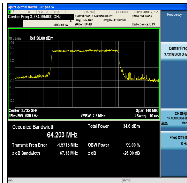
NTNV-n77(3700-3980)-PC2-30-70-L-DFT-16QAM- Outer_Full-Ant1-PASS
