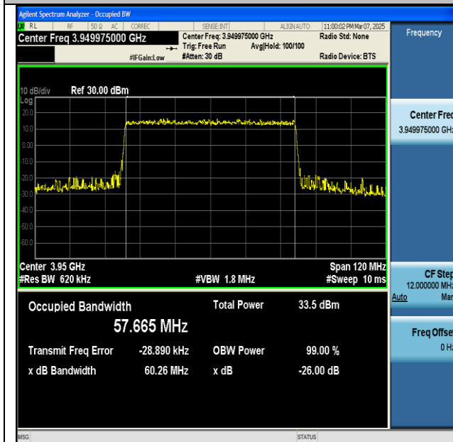
NTNV-n77(3700-3980)-PC2-30-60-H-CP-QPSK- Outer_Full-Ant1-PASS
