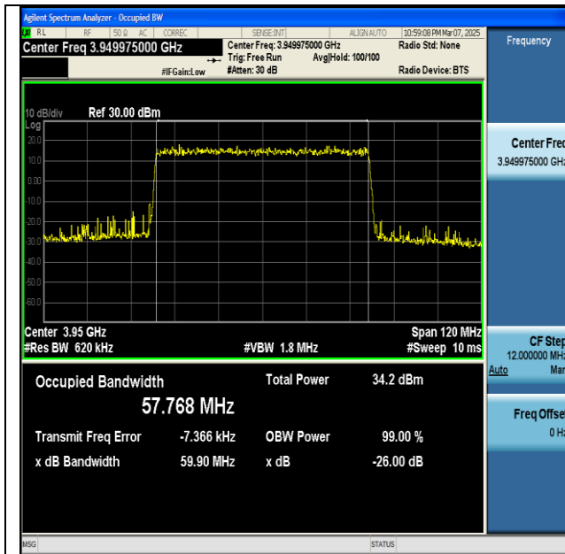
NTNV-n77(3700-3980)-PC2-30-60-H-DFT-64QAM- Outer_Full-Ant1-PASS
