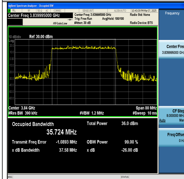
NTNV-n77(3700-3980)-PC2-30-40-M-DFT-BPSK- Outer_Full-Ant1-PASS
