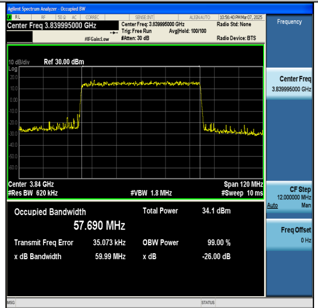
NTNV-n77(3700-3980)-PC2-30-60-M-DFT-64QAM- Outer_Full-Ant1-PASS
