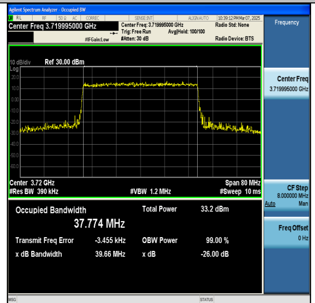
NTNV-n77(3700-3980)-PC2-30-40-L-CP-16QAM- Outer_Full-Ant1-PASS
