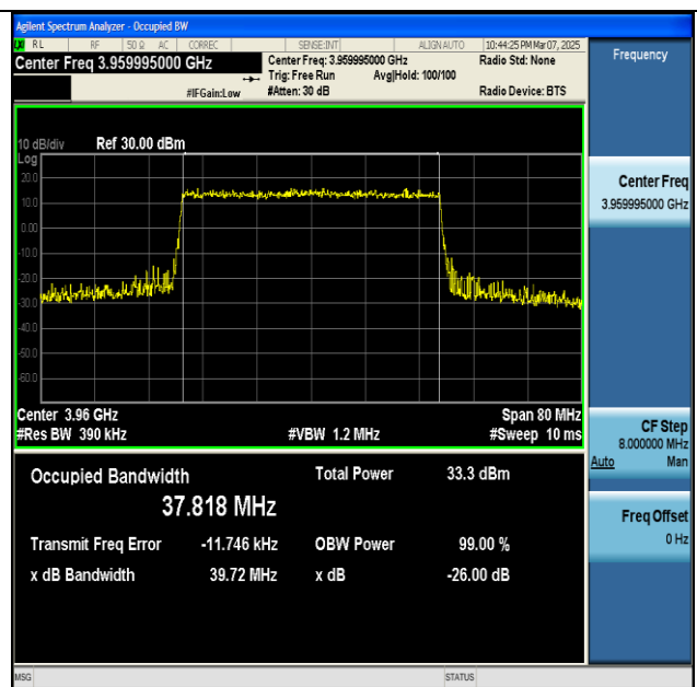
NTNV-n77(3700-3980)-PC2-30-40-H-CP-16QAM-Outer_Full-Ant1-PASS
