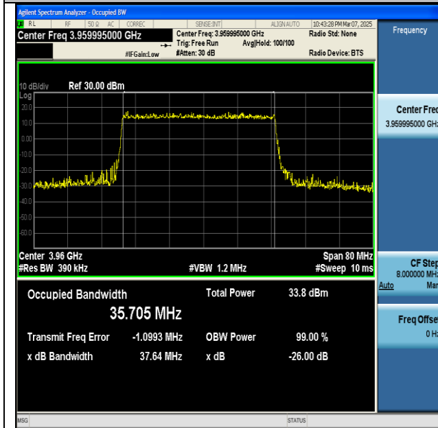
NTNV-n77(3700-3980)-PC2-30-40-H-DFT-64QAM- Outer_Full-Ant1-PASS
