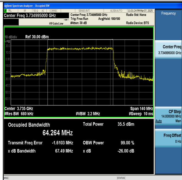
NTNV-n77(3700-3980)-PC2-30-70-L-DFT-QPSK-Outer_Full-Ant1-PASS
