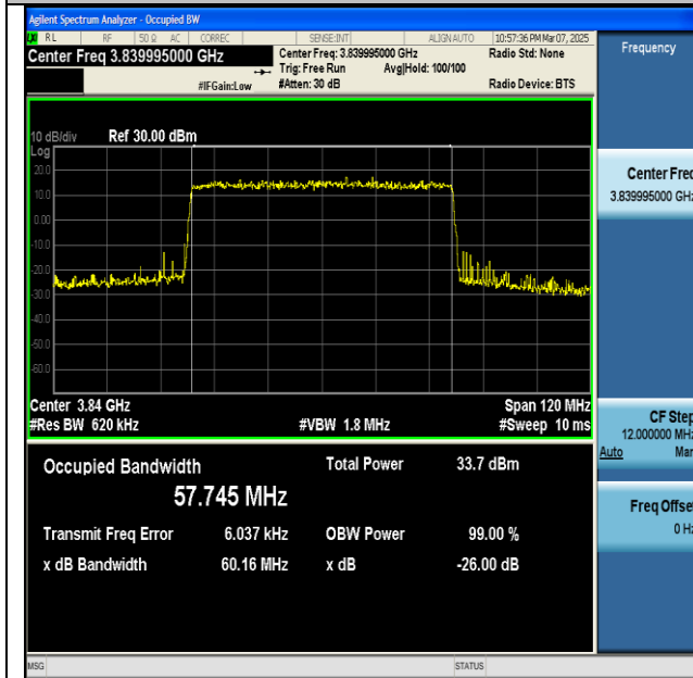
NTNV-n77(3700-3980)-PC2-30-60-M-CP-16QAM- Outer_Full-Ant1-PASS
