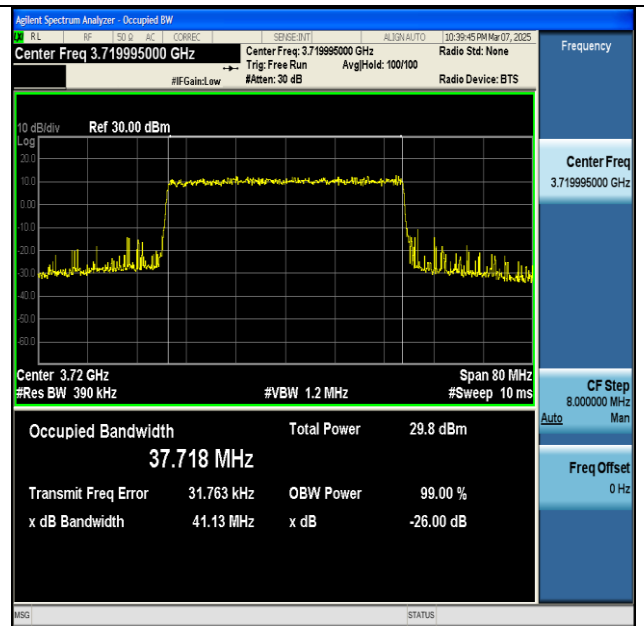
NTNV-n77(3700-3980)-PC2-30-40-L-CP-256QAM- Outer_Full-Ant1-PASS
