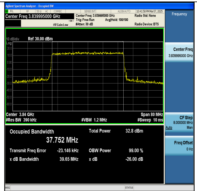
NTNV-n77(3700-3980)-PC2-30-40-M-CP-64QAM- Outer_Full-Ant1-PASS
