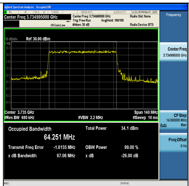
NTNV-n77(3700-3980)-PC2-30-70-L-DFT-64QAM- Outer_Full-Ant1-PASS
