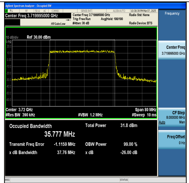
NTNV-n77(3700-3980)-PC2-30-40-L-DFT-256QAM- Outer_Full-Ant1-PASS
