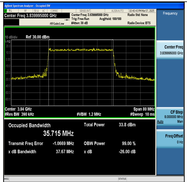
NTNV-n77(3700-3980)-PC2-30-40-M-DFT-64QAM- Outer_Full-Ant1-PASS
