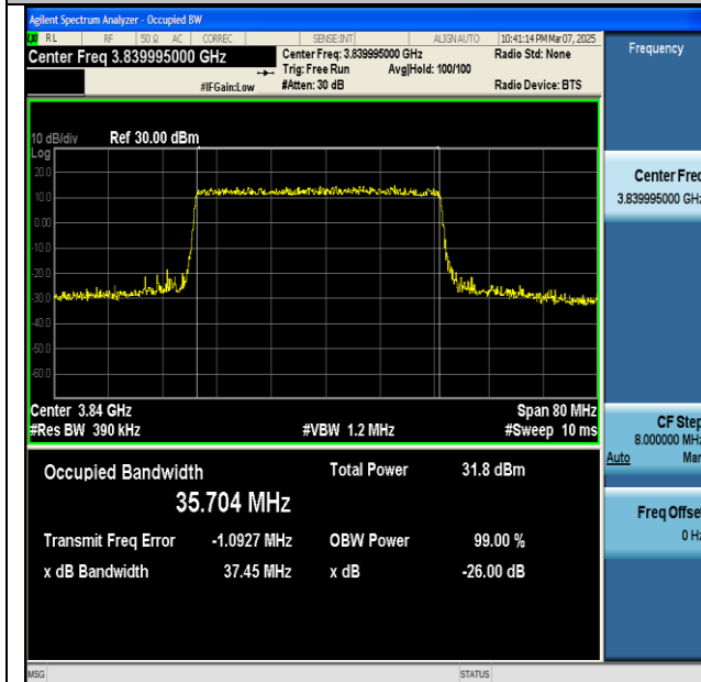
NTNV-n77(3700-3980)-PC2-30-40-M-DFT-256QAM- Outer_Full-Ant1-PASS
