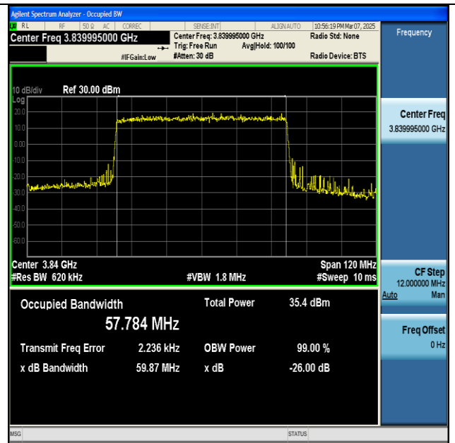
NTNV-n77(3700-3980)-PC2-30-60-M-DFT-QPSK- Outer_Full-Ant1-PASS
