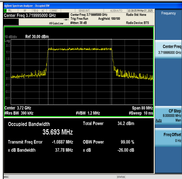
NTNV-n77(3700-3980)-PC2-30-40-L-DFT-16QAM-Outer_Full-Ant1-PASS
