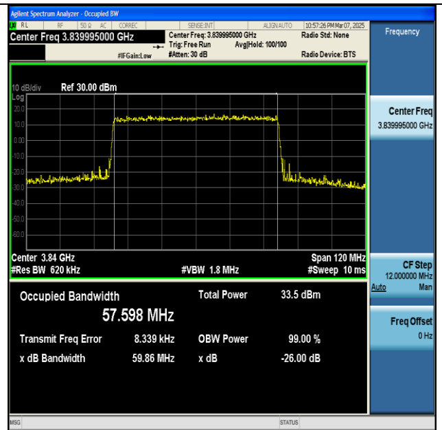
NTNV-n77(3700-3980)-PC2-30-60-M-CP-QPSK- Outer_Full-Ant1-PASS
