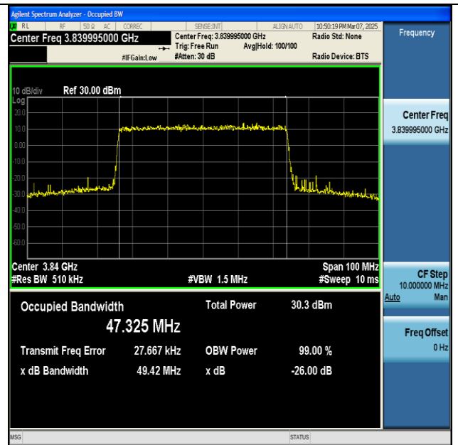
NTNV-n77(3700-3980)-PC2-30-50-M-CP-256QAM- Outer_Full-Ant1-PASS
