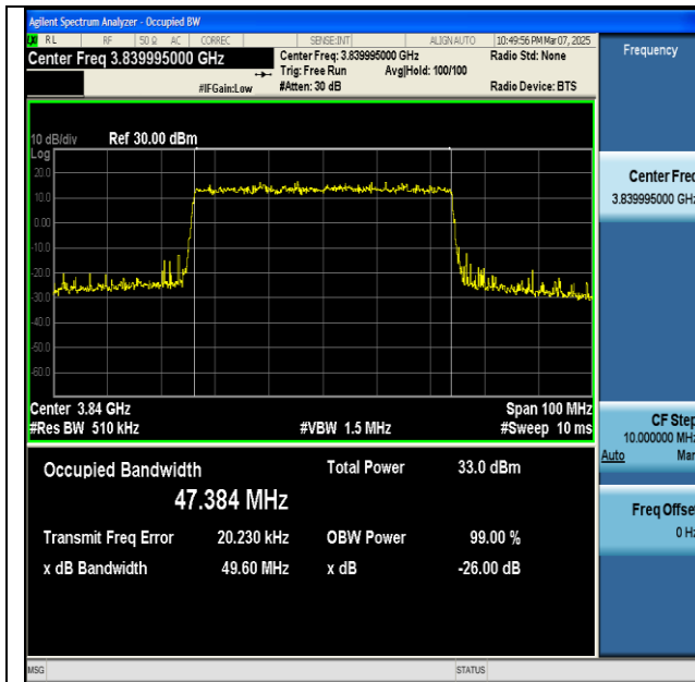
NTNV-n77(3700-3980)-PC2-30-50-M-CP-64QAM- Outer_Full-Ant1-PASS
