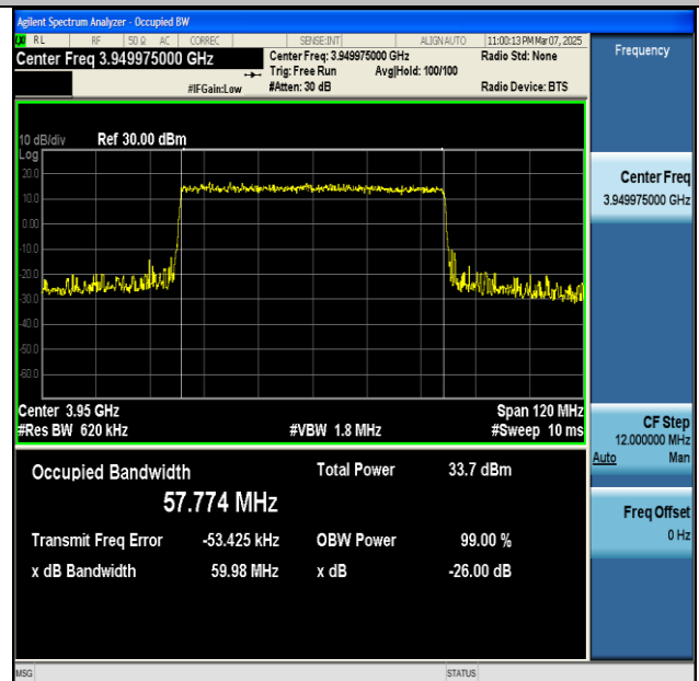
NTNV-n77(3700-3980)-PC2-30-60-H-CP-16QAM- Outer_Full-Ant1-PASS
