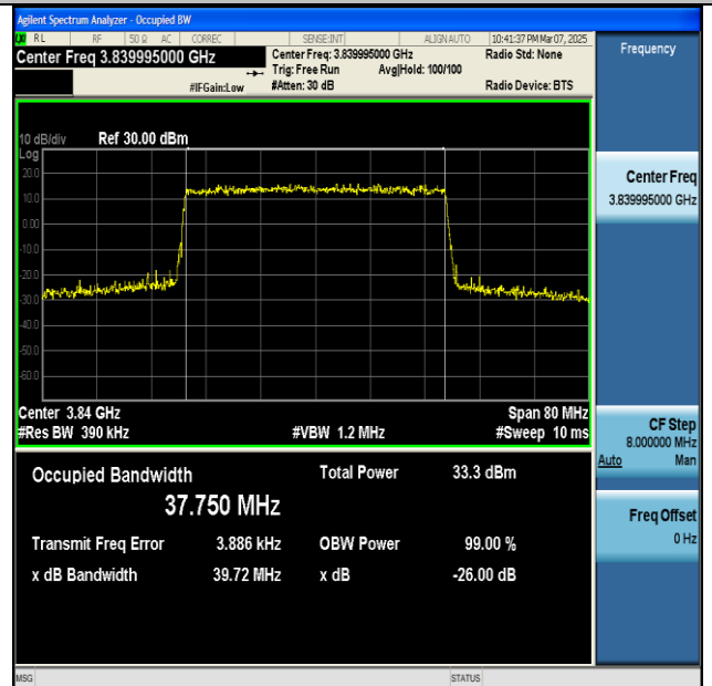
NTNV-n77(3700-3980)-PC2-30-40-M-CP-QPSK- Outer_Full-Ant1-PASS
