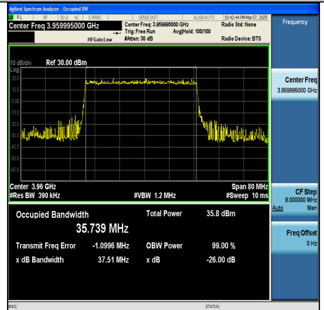
NTNV-n77(3700-3980)-PC2-30-40-H-DFT-BPSK- Outer_Full-Ant1-PASS
