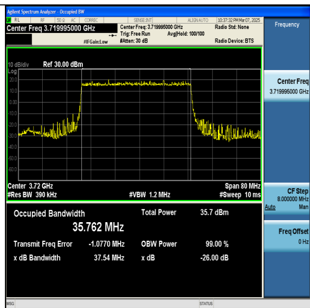
NTNV-n77(3700-3980)-PC2-30-40-L-DFT-BPSK-Outer_Full-Ant1-PASS
