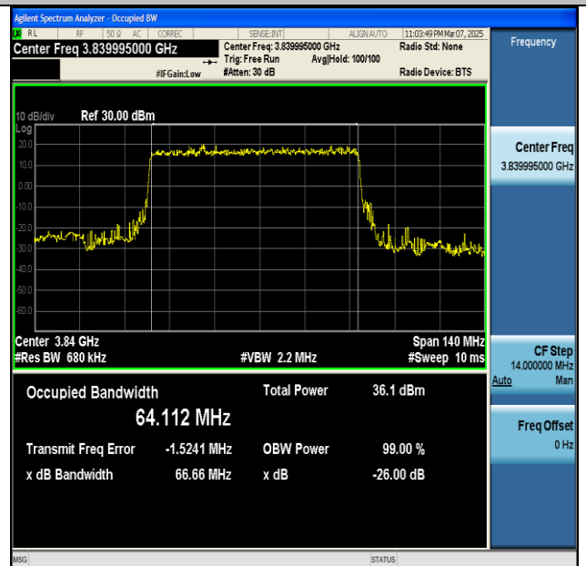
NTNV-n77(3700-3980)-PC2-30-70-M-DFT-BPSK- Outer_Full-Ant1-PASS
