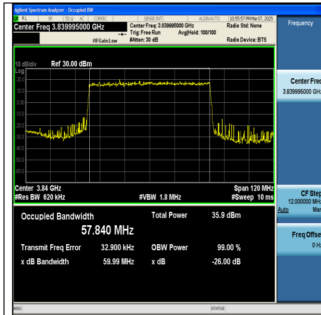
NTNV-n77(3700-3980)-PC2-30-60-M-DFT-BPSK- Outer_Full-Ant1-PASS
