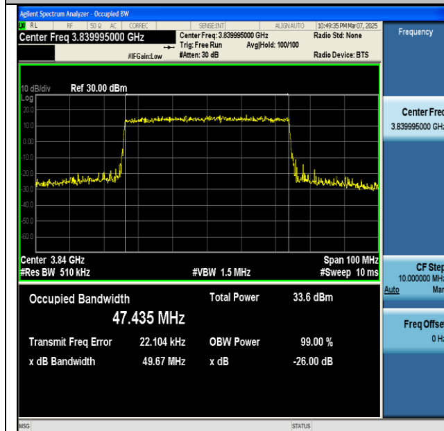
NTNV-n77(3700-3980)-PC2-30-50-M-CP-QPSK- Outer_Full-Ant1-PASS
