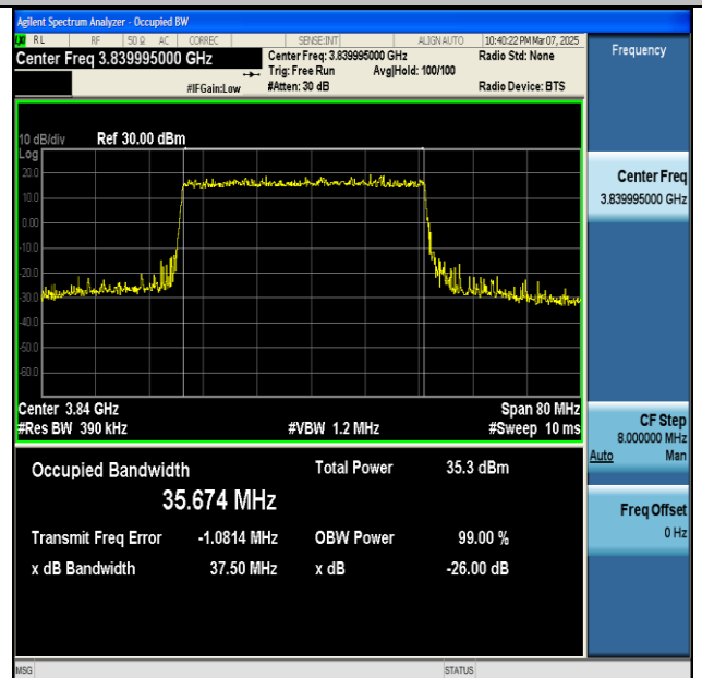
NTNV-n77(3700-3980)-PC2-30-40-M-DFT-QPSK- Outer_Full-Ant1-PASS
