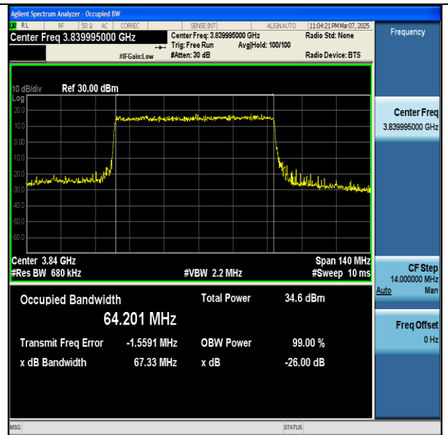
NTNV-n77(3700-3980)-PC2-30-70-M-DFT-16QAM- Outer_Full-Ant1-PASS
