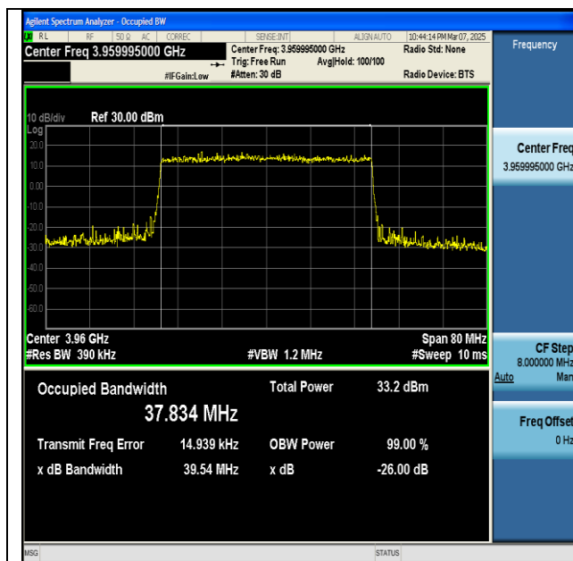
NTNV-n77(3700-3980)-PC2-30-40-H-CP-QPSK-Outer_Full-Ant1-PASS
