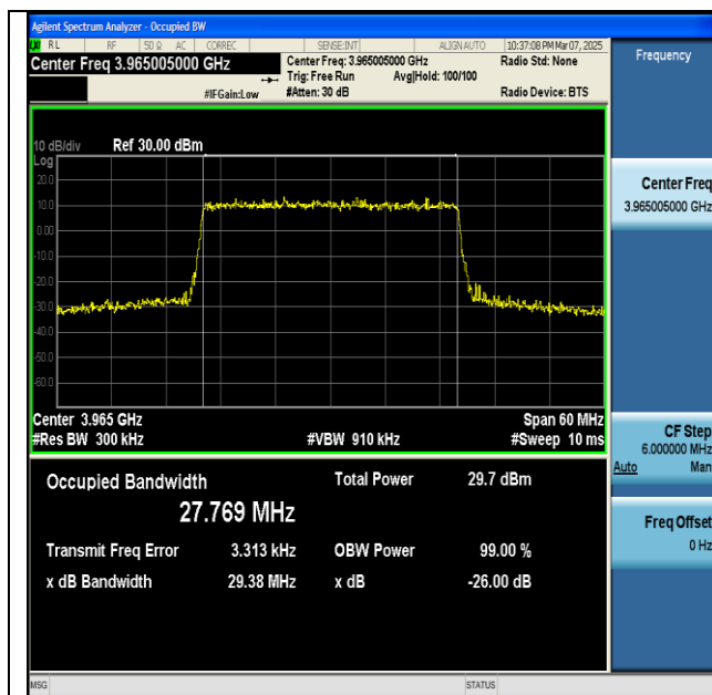
NTNV-n77(3700-3980)-PC2-30-30-H-CP-256QAM-Outer_Full-Ant1-PASS
