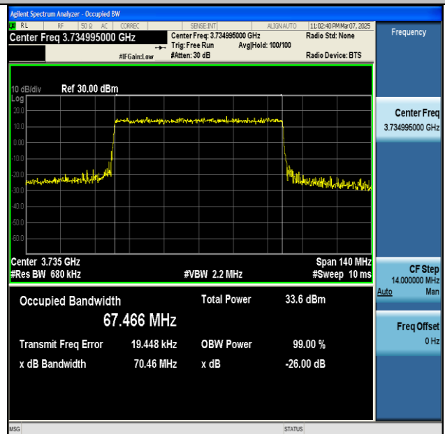
NTNV-n77(3700-3980)-PC2-30-70-L-CP-QPSK- Outer_Full-Ant1-PASS
