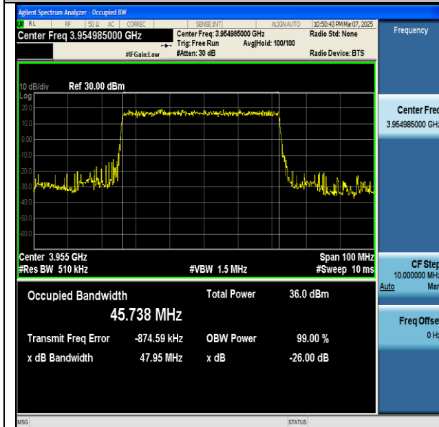
NTNV-n77(3700-3980)-PC2-30-50-H-DFT-BPSK- Outer_Full-Ant1-PASS
