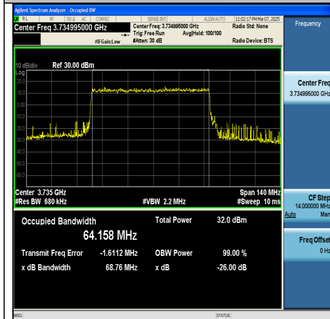
NTNV-n77(3700-3980)-PC2-30-70-L-DFT-256QAM- Outer_Full-Ant1-PASS
