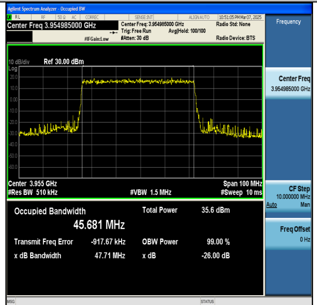
NTNV-n77(3700-3980)-PC2-30-50-H-DFT-QPSK- Outer_Full-Ant1-PASS
