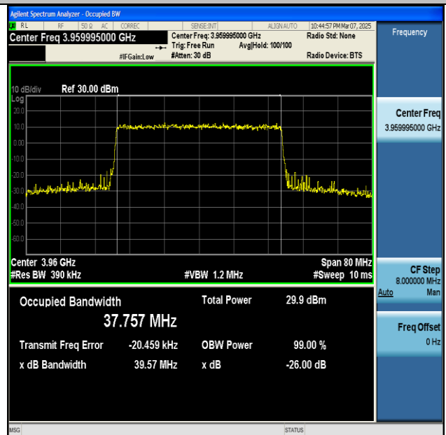
NTNV-n77(3700-3980)-PC2-30-40-H-CP-256QAM-Outer_Full-Ant1-PASS
