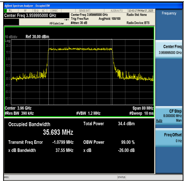
NTNV-n77(3700-3980)-PC2-30-40-H-DFT-16QAM- Outer_Full-Ant1-PASS
