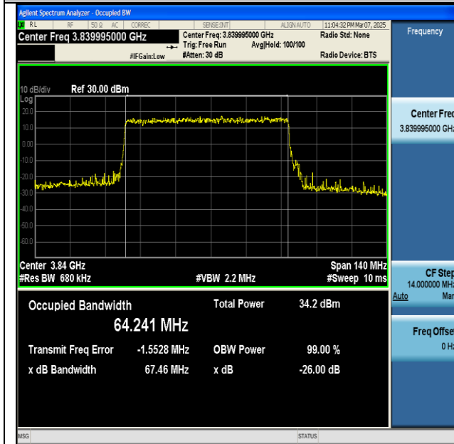
NTNV-n77(3700-3980)-PC2-30-70-M-DFT-64QAM- Outer_Full-Ant1-PASS
