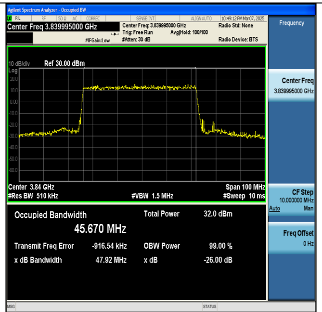
NTNV-n77(3700-3980)-PC2-30-50-M-DFT-256QAM- Outer_Full-Ant1-PASS
