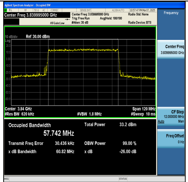
NTNV-n77(3700-3980)-PC2-30-60-M-CP-64QAM- Outer_Full-Ant1-PASS
