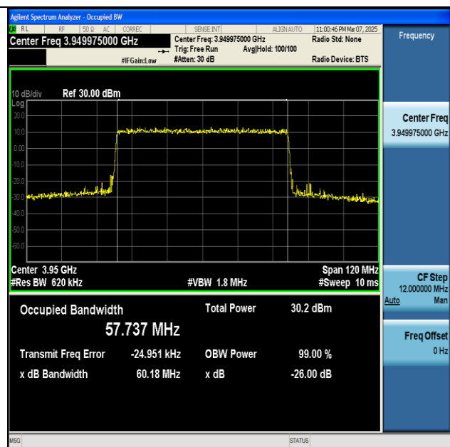
NTNV-n77(3700-3980)-PC2-30-60-H-CP-256QAM-Outer_Full-Ant1-PASS
