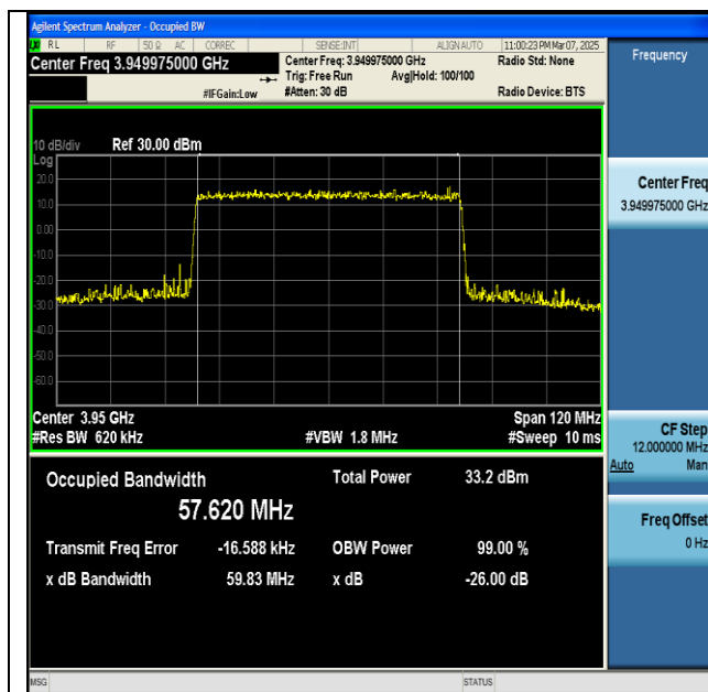
NTNV-n77(3700-3980)-PC2-30-60-H-CP-64QAM-Outer_Full-Ant1-PASS
