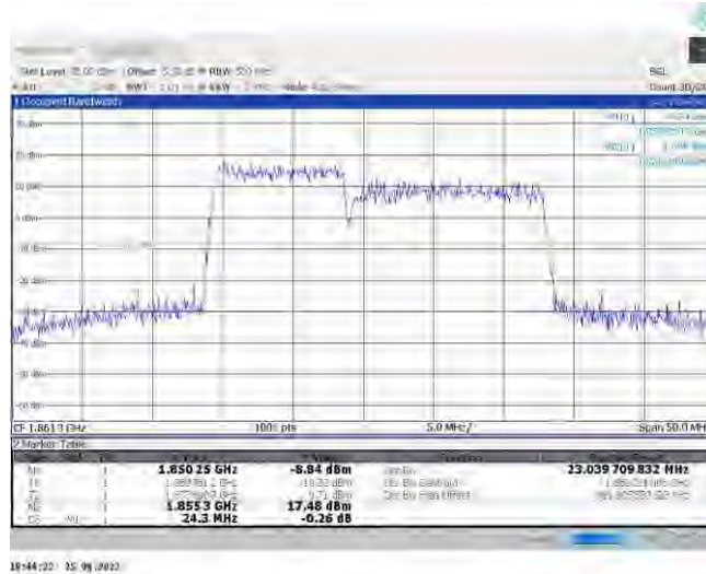
2-2-10MHz-15MHz-QPSK-QPSK-18829-18949-50RB#0-75RB#0
