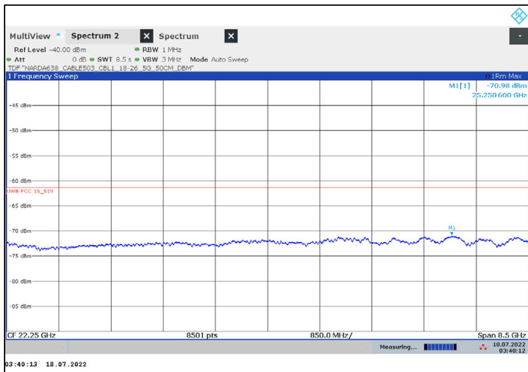
Plot 11: 18 GHz to 26.5 GHz, UWB test mode
