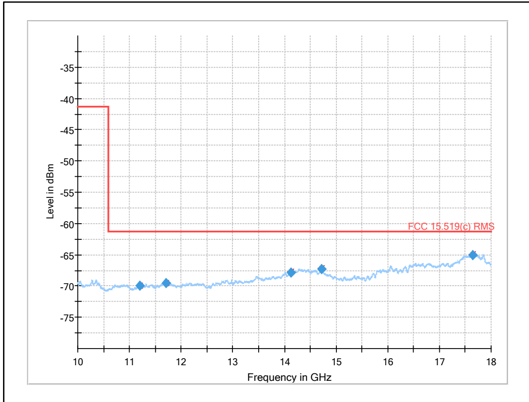
Plot 32: 10 GHz to 18 GHz, UWB test mode
