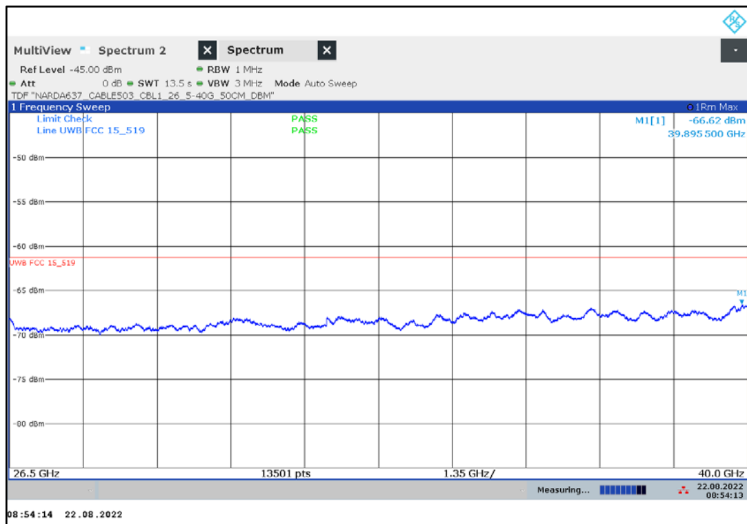
Plot 23: 26.5 GHz to 40.0 GHz, UWB test mode
