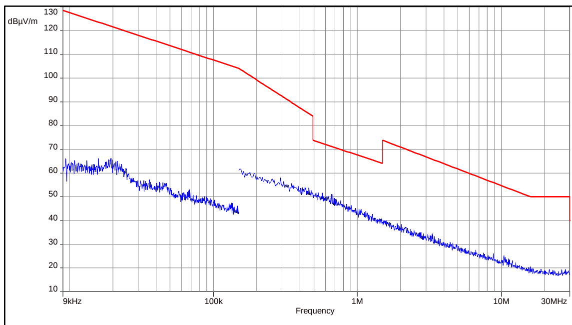
Plot 17: 9 kHz to 30 MHz, UWB test mode
