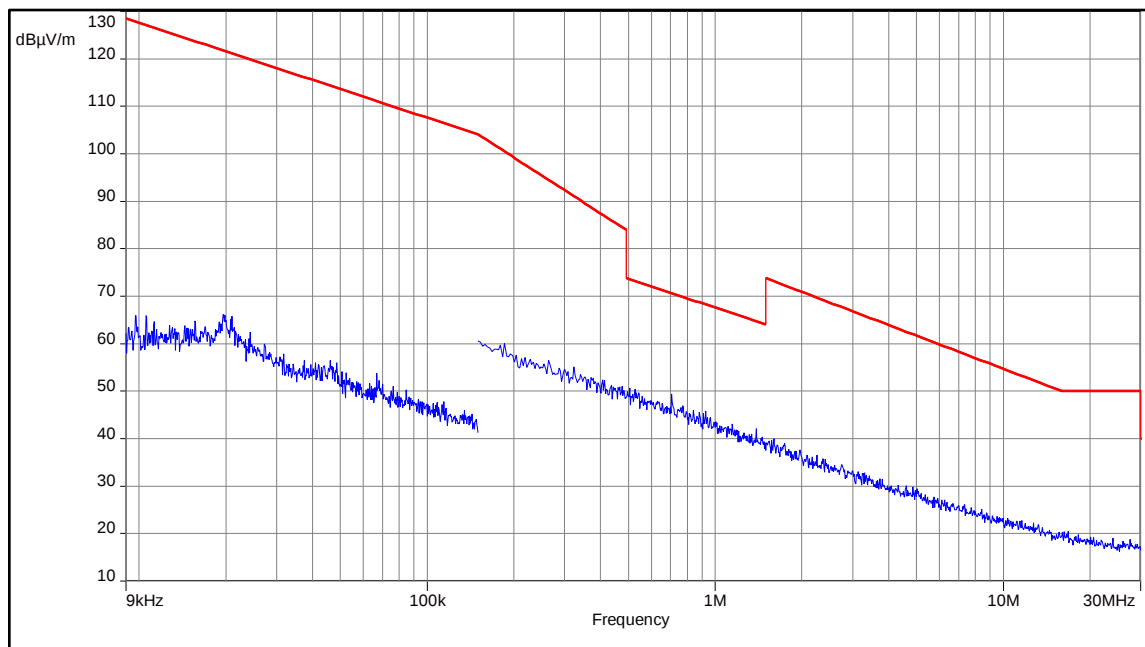
Plot 6: 9 kHz to 30 MHz, UWB test mode
