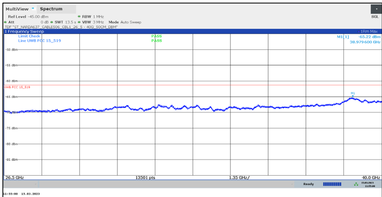
Plot 34: 26.5 GHz to 40.0 GHz, UWB test mode
