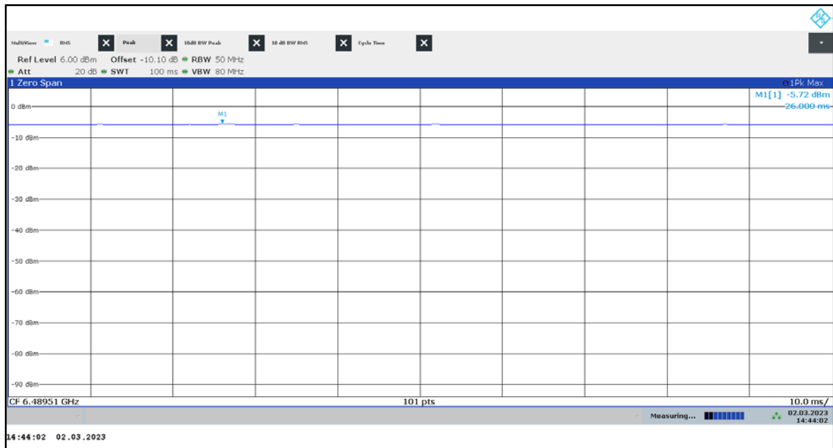
Plot 27: Fundamental emission (UWB test mode): Max Peak
