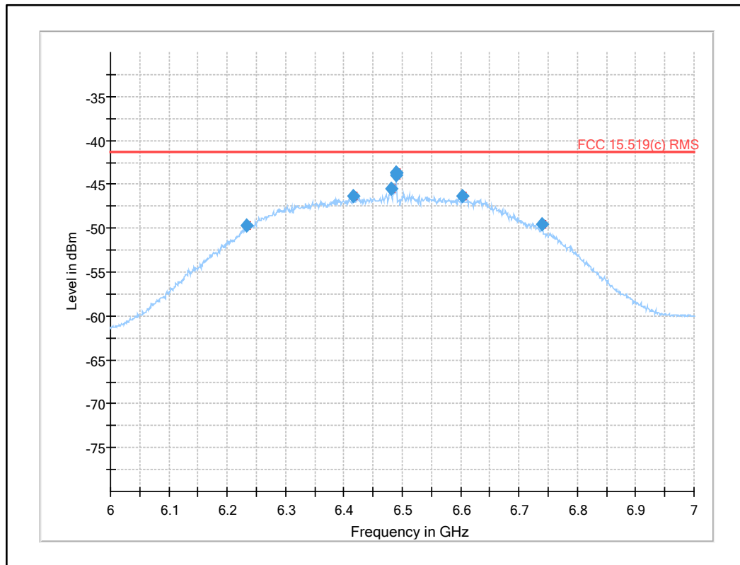
Plot 26: Fundamental emission (UWB test mode): RMS
