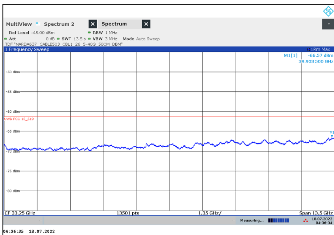
Plot 12: 26.5 GHz to 40.0 GHz, UWB test mode
