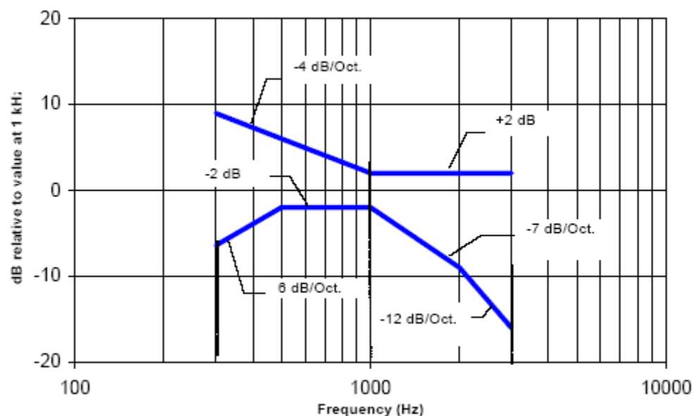
Figure 6.5-4 Magnetic field frequency response for WDs with a field strength of exceeding -15 dB(A/m) at 1 kHz
