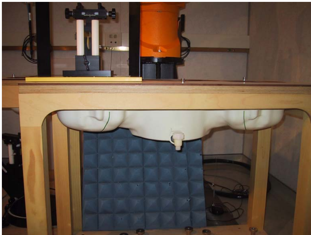
Figure 8.1-1 DASY5 system with absorbing material
