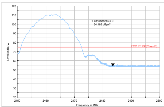
802.11b-Channel 11 Peak
