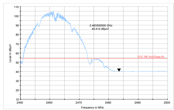
802.11b-Channel 11 Average
