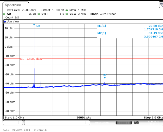
Band4-1.4MHz-QPSK-20393-1-5-Low-5000-12000--45.32-PASS
