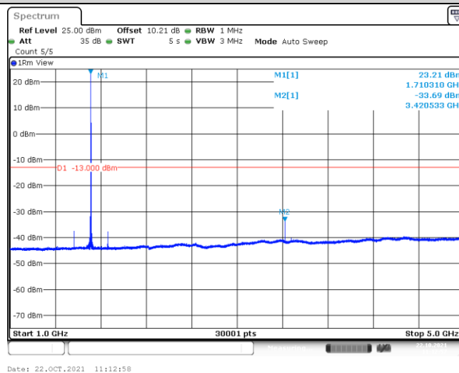
Band4-1.4MHz-16QAM-19957-1-0-Low-5000-12000--45.96-PASS
