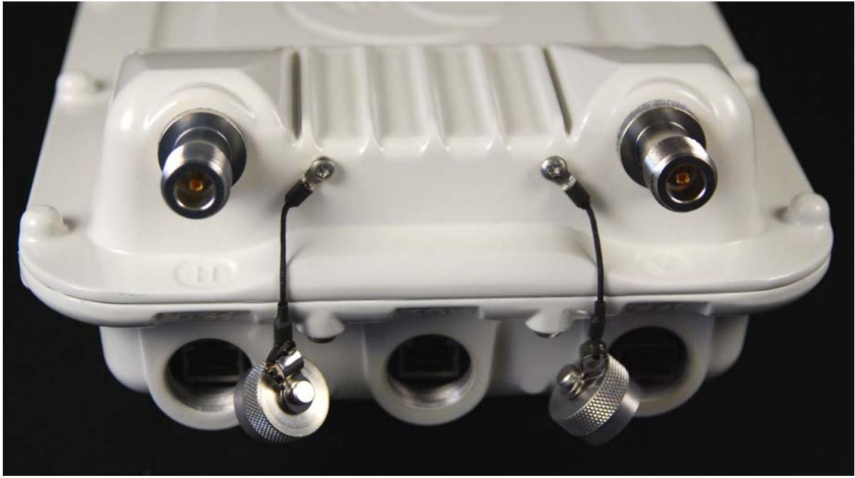
PTP 700 Connectorized ODU - Connectors with Covers Removed
