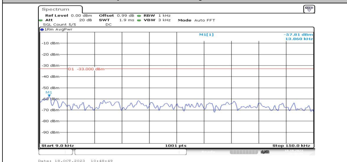
Band2-1.4MHz-16QAM-18607-1RB#0-Range1:0.009~0.15MHz-PASS
