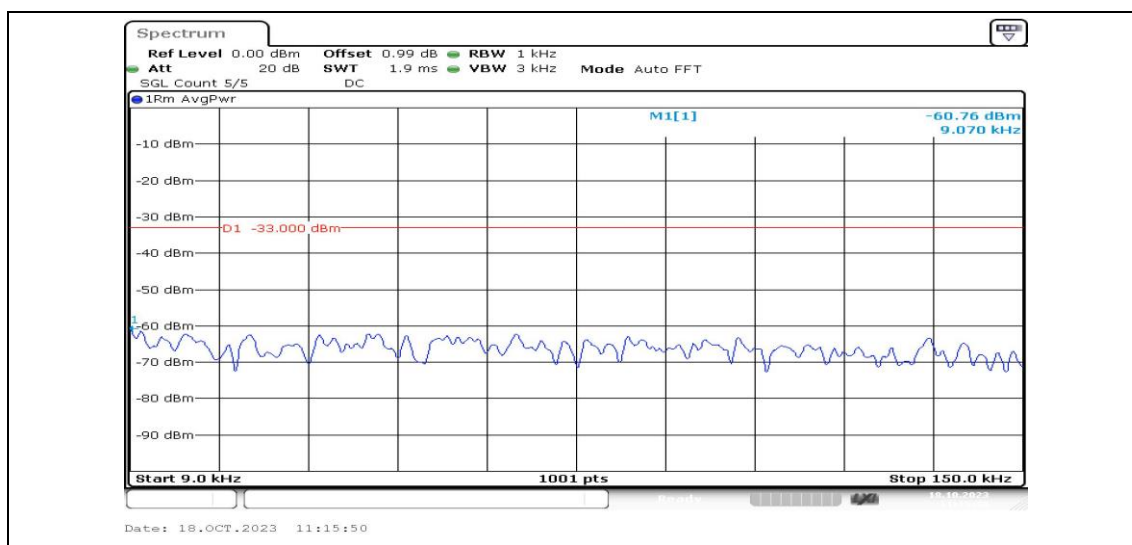
Band2-3MHz-16QAM-19185-1RB#0-Range1:0.009~0.15MHz-PASS
