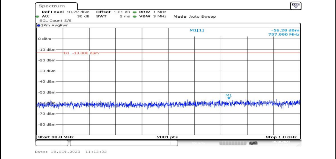
Band2-3MHz-16QAM-18615-1RB#0-Range3:30~1000MHz-PASS
