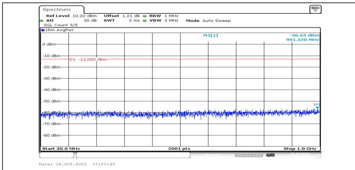
Band2-1.4MHz-16QAM-18900-1RB#0-Range3:30~1000MHz-PASS
