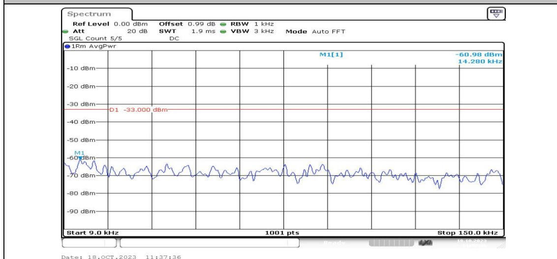
Band2-5MHz-16QAM-18625-1RB#0-Range1:0.009~0.15MHz-PASS
