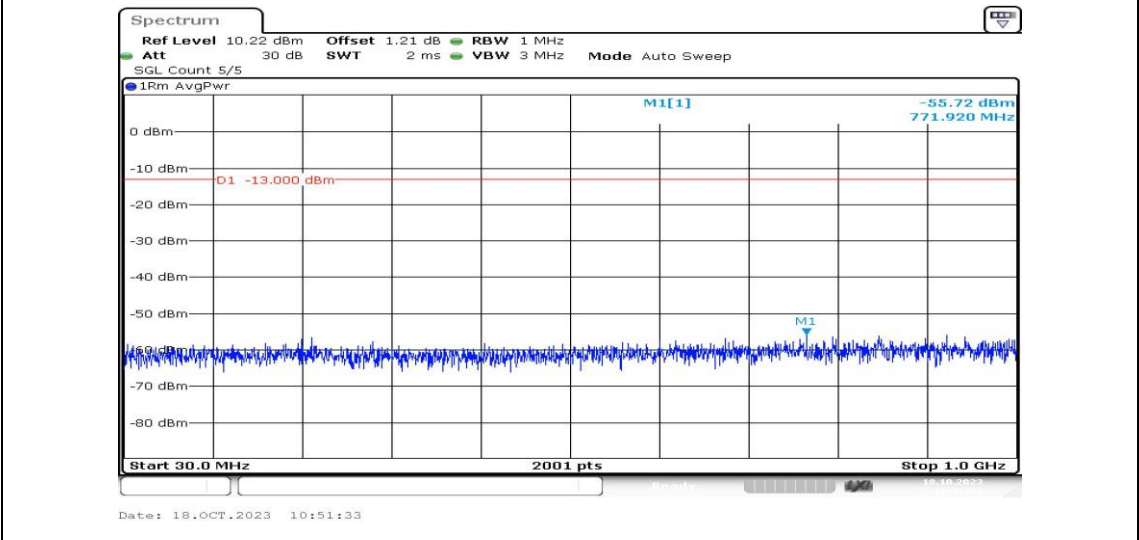
Band2-1.4MHz-QPSK-19193-1RB#0-Range3:30~1000MHz-PASS
