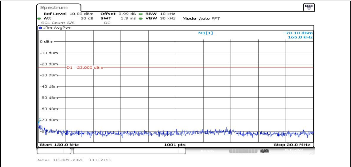
Band2-3MHz-16QAM-18615-1RB#0-Range2:0.15~30MHz-PASS
