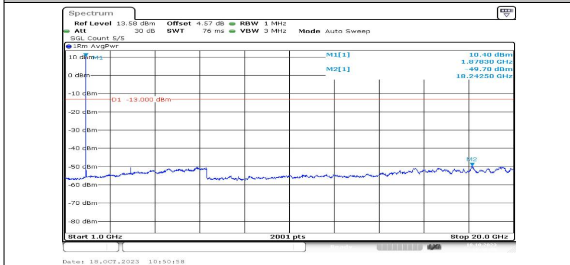
Band2-1.4MHz-16QAM-18900-1RB#0-Range4:1000~20000MHz-PASS
