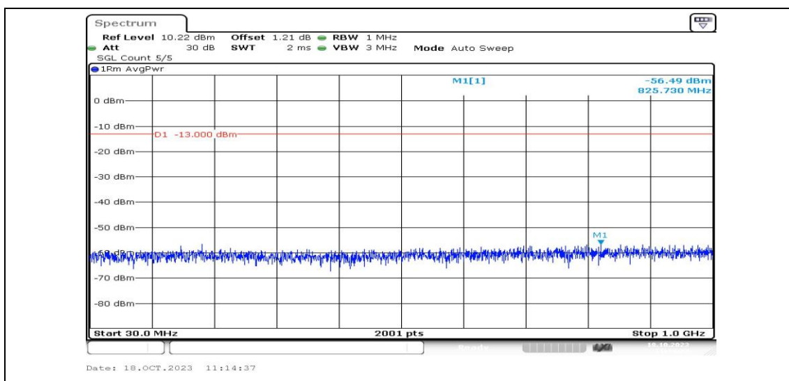
Band2-3MHz-16QAM-18900-1RB#0-Range3:30~1000MHz-PASS
