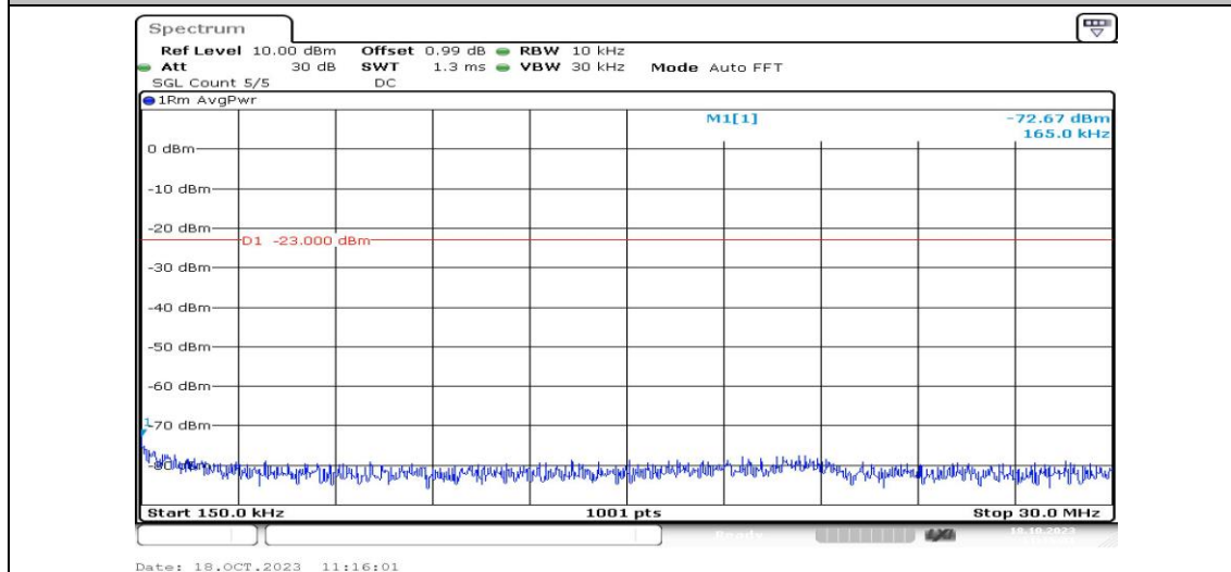
Band2-3MHz-16QAM-19185-1RB#0-Range2:0.15~30MHz-PASS
