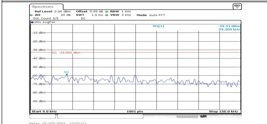
Band2-1.4MHz-QPSK-19193-1RB#0-Range1:0.009~0.15MHz-PASS
