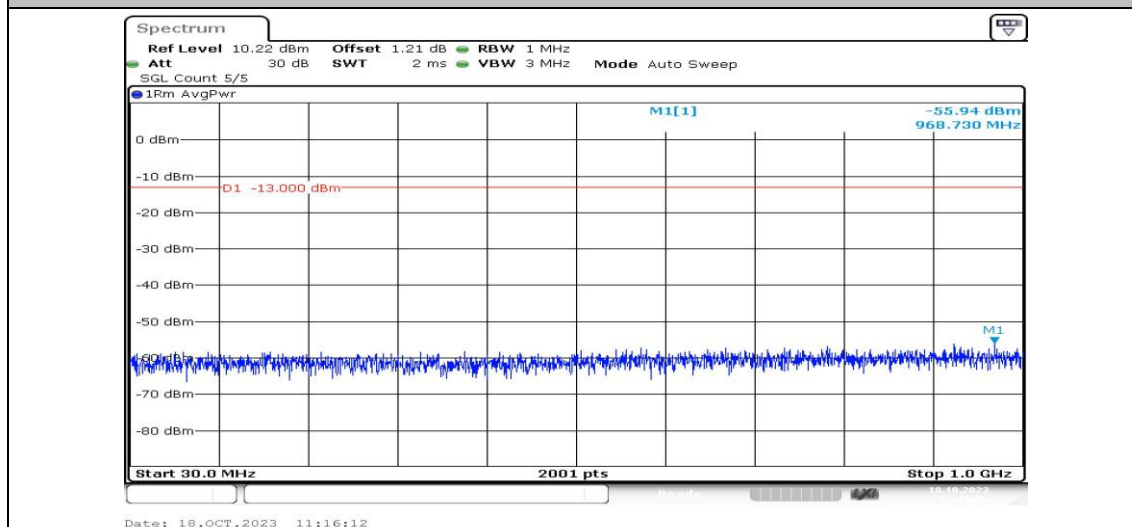
Band2-3MHz-16QAM-19185-1RB#0-Range3:30~1000MHz-PASS
