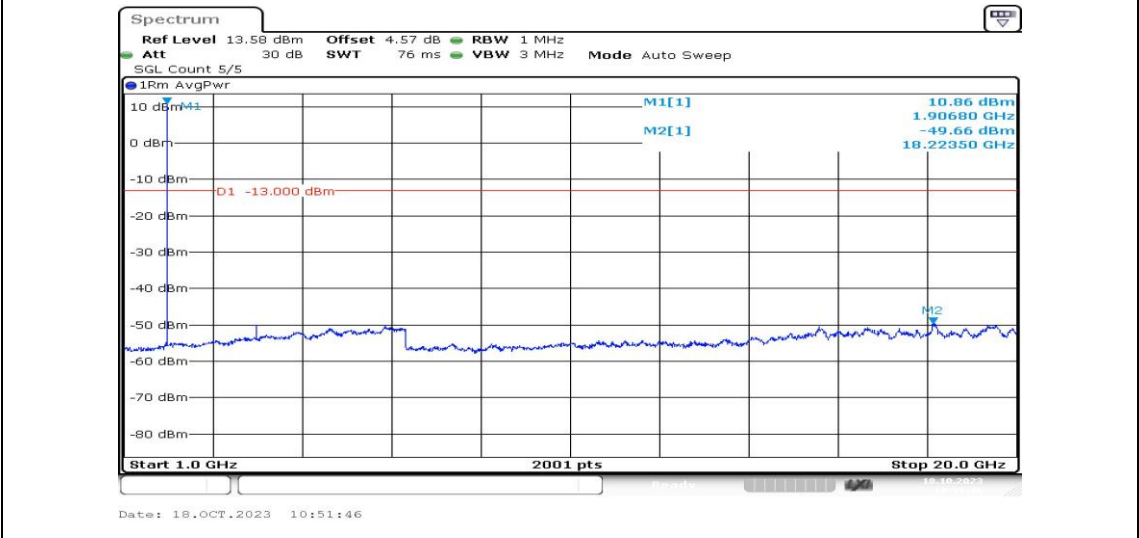
Band2-1.4MHz-QPSK-19193-1RB#0-Range4:1000~20000MHz-PASS
