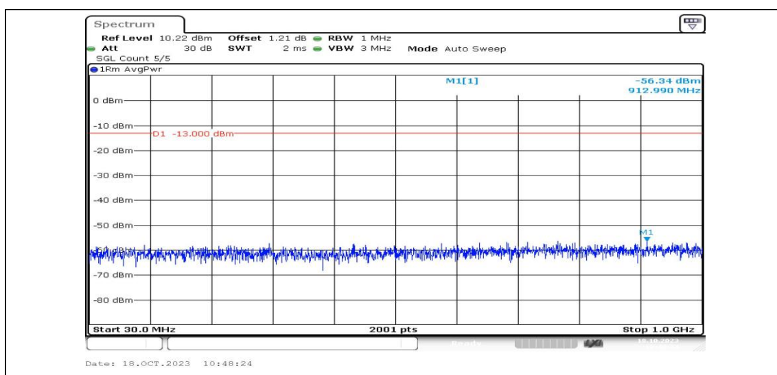
Band2-1.4MHz-QPSK-18607-1RB#0-Range3:30~1000MHz-PASS
