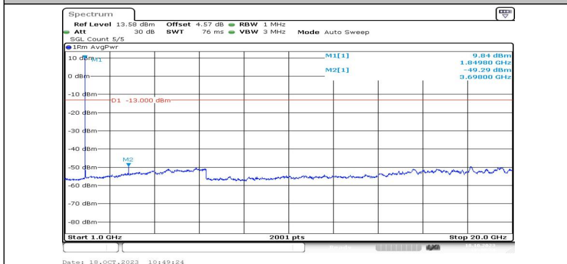
Band2-1.4MHz-16QAM-18607-1RB#0-Range4:1000~20000MHz-PASS
