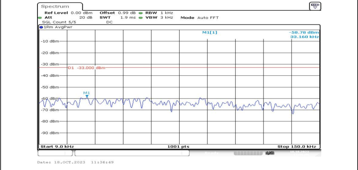
Band2-5MHz-QPSK-18625-1RB#0-Range1:0.009~0.15MHz-PASS
