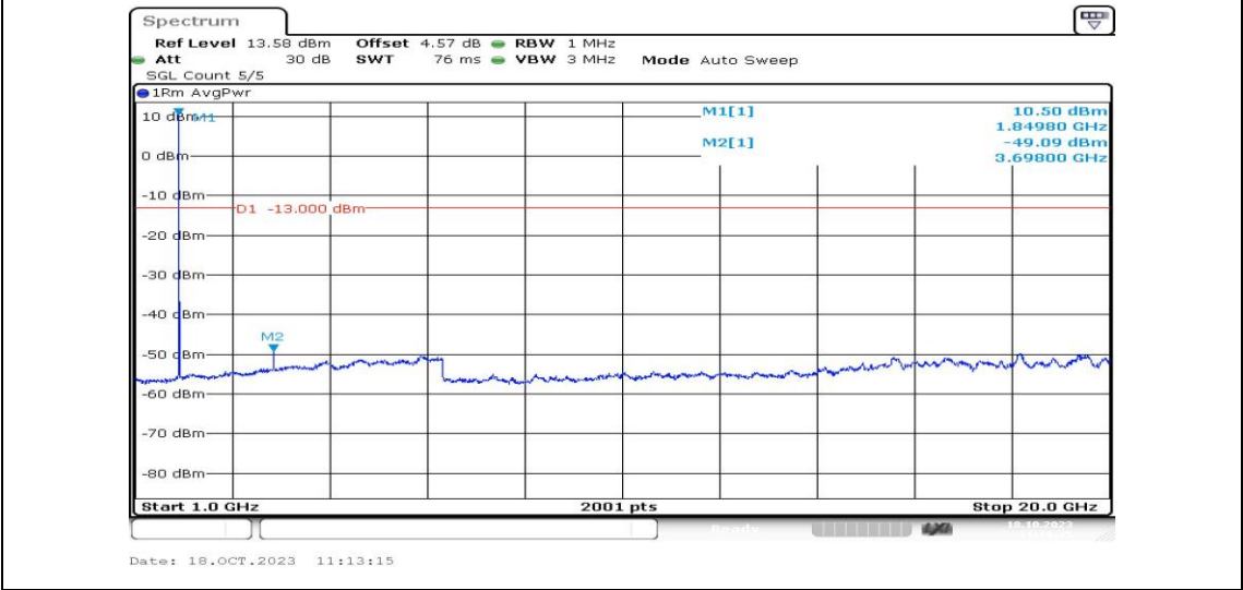
Band2-3MHz-16QAM-18615-1RB#0-Range4:1000~20000MHz-PASS
