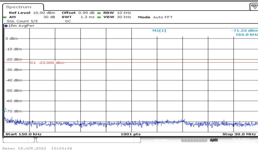
Band2-1.4MHz-16QAM-18900-1RB#0-Range2:0.15~30MHz-PASS
