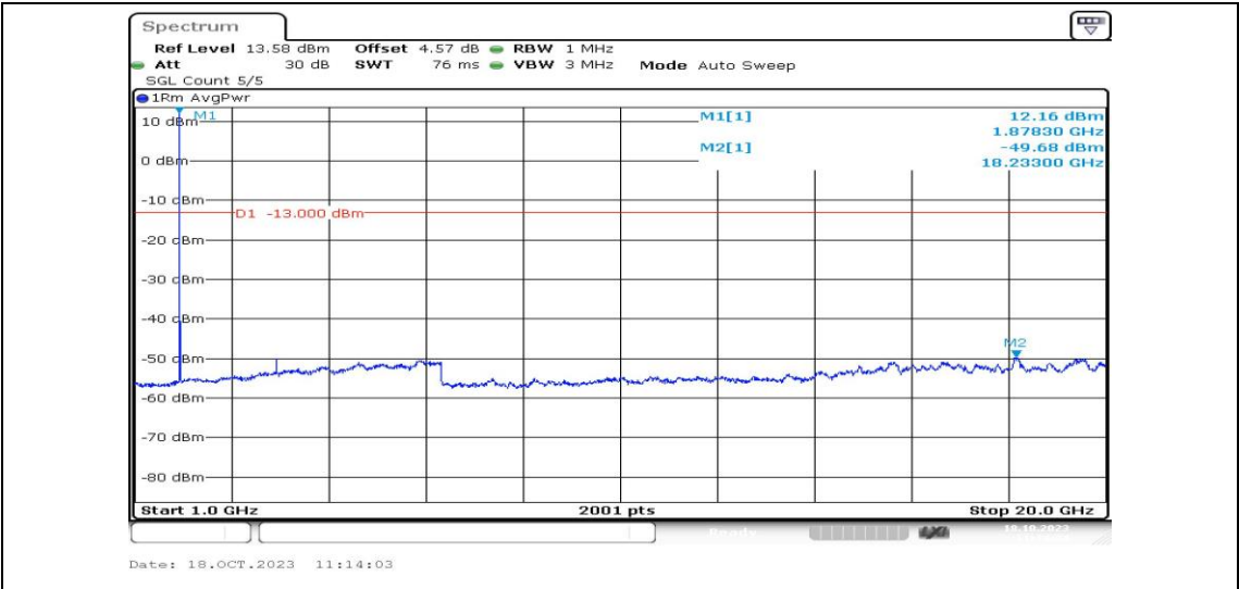
Band2-3MHz-QPSK-18900-1RB#0-Range4:1000~20000MHz-PASS
