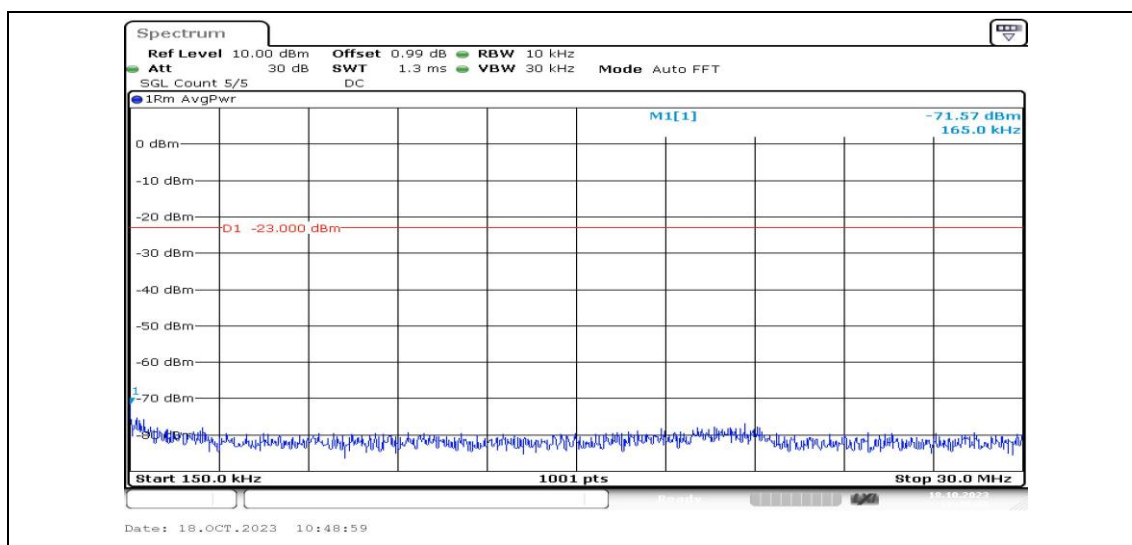
Band2-1.4MHz-16QAM-18607-1RB#0-Range2:0.15~30MHz-PASS
