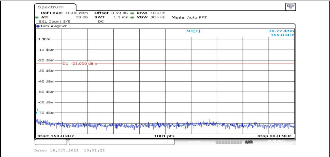
Band2-1.4MHz-QPSK-19193-1RB#0-Range2:0.15~30MHz-PASS
