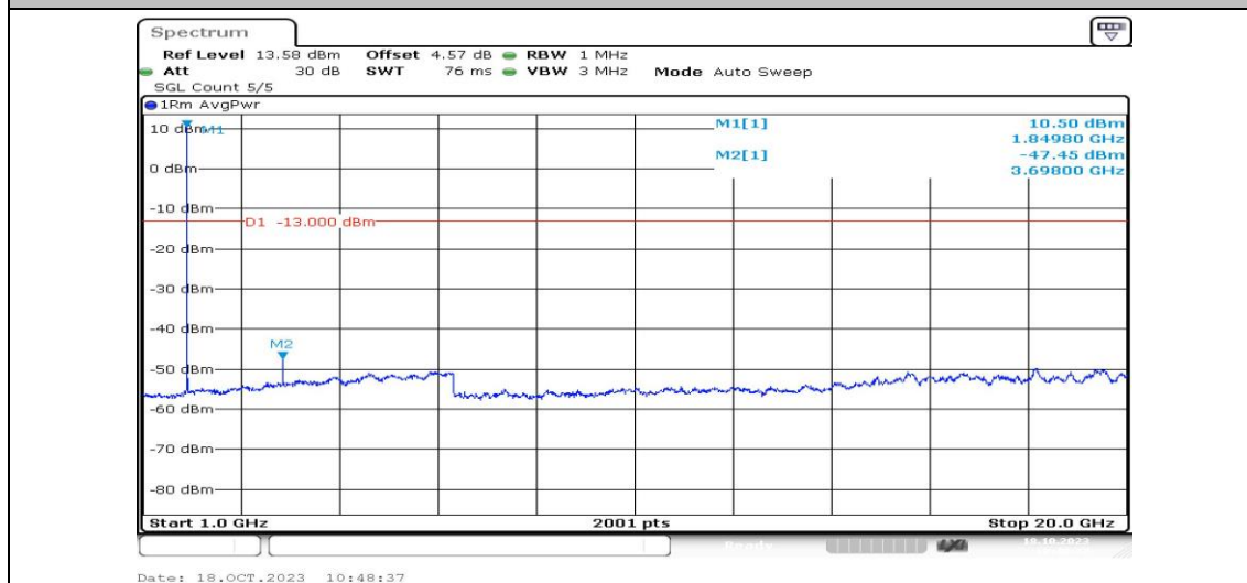
Band2-1.4MHz-QPSK-18607-1RB#0-Range4:1000~20000MHz-PASS
