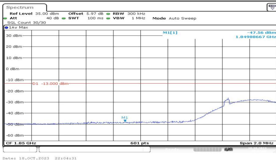
Band2-15MHz-16QAM-18675-1RB#74-PASS
