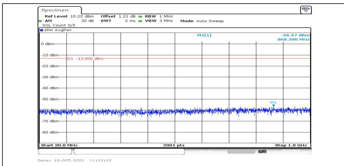
Band2-3MHz-QPSK-18615-1RB#0-Range3:30~1000MHz-PASS
