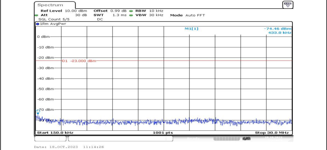
Band2-3MHz-16QAM-18900-1RB#0-Range2:0.15~30MHz-PASS
