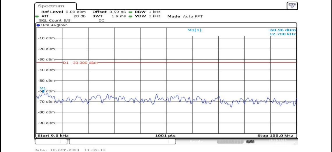
Band2-5MHz-16QAM-18900-1RB#0-Range1:0.009~0.15MHz-PASS
