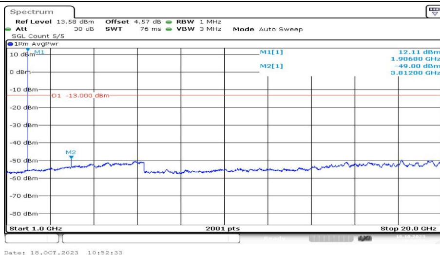
Band2-1.4MHz-16QAM-19193-1RB#0-Range4:1000~20000MHz-PASS
