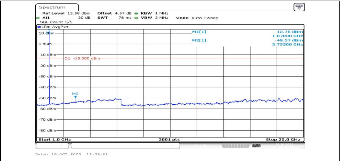
Band2-5MHz-QPSK-18900-1RB#0-Range4:1000~20000MHz-PASS
