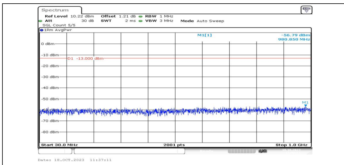
Band2-5MHz-QPSK-18625-1RB#0-Range3:30~1000MHz-PASS
