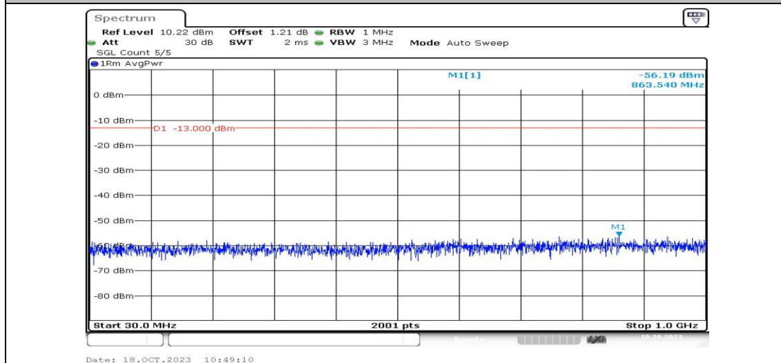
Band2-1.4MHz-16QAM-18607-1RB#0-Range3:30~1000MHz-PASS
