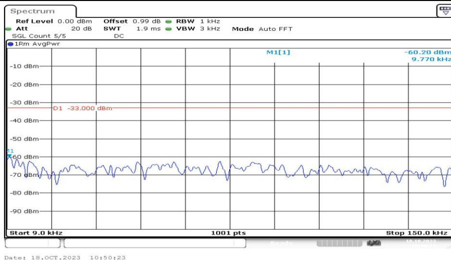
Band2-1.4MHz-16QAM-18900-1RB#0-Range1:0.009~0.15MHz-PASS
