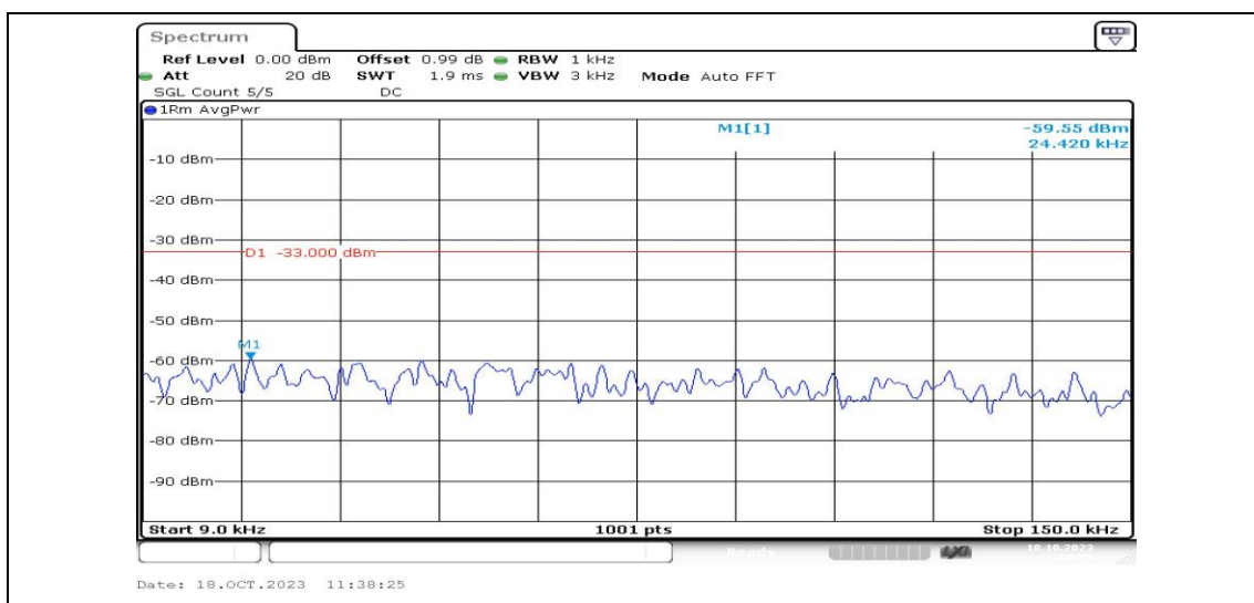
Band2-5MHz-QPSK-18900-1RB#0-Range1:0.009~0.15MHz-PASS
