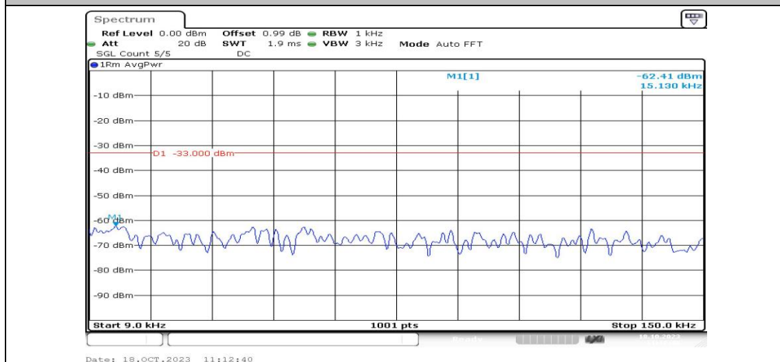
Band2-3MHz-16QAM-18615-1RB#0-Range1:0.009~0.15MHz-PASS
