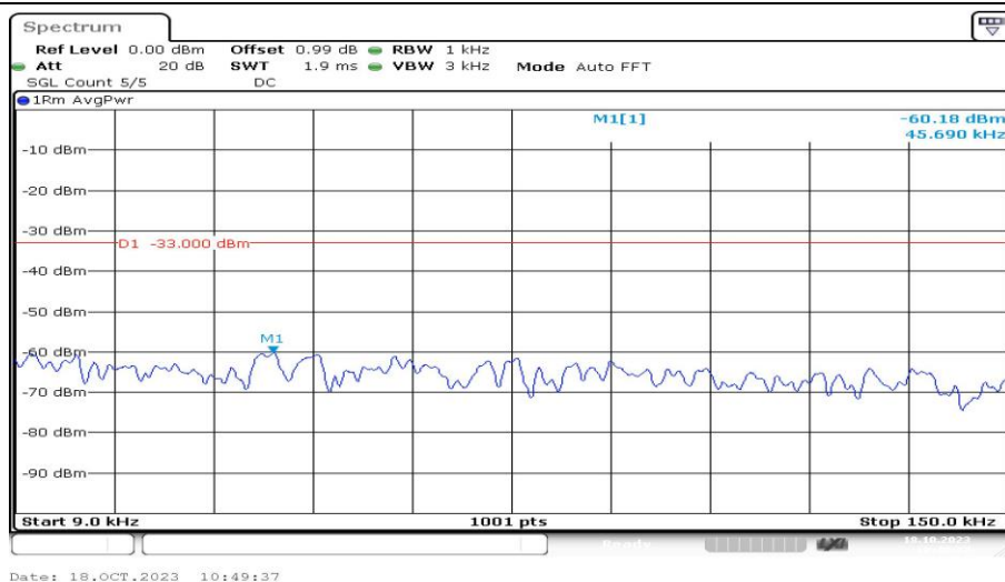
Band2-1.4MHz-QPSK-18900-1RB#0-Range1:0.009~0.15MHz-PASS
