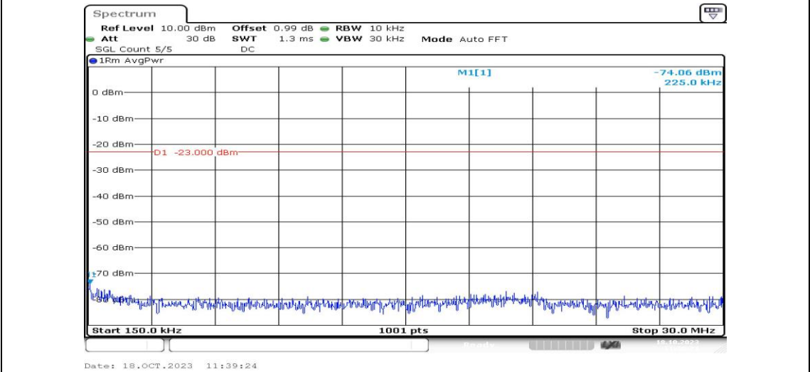
Band2-5MHz-16QAM-18900-1RB#0-Range2:0.15~30MHz-PASS
