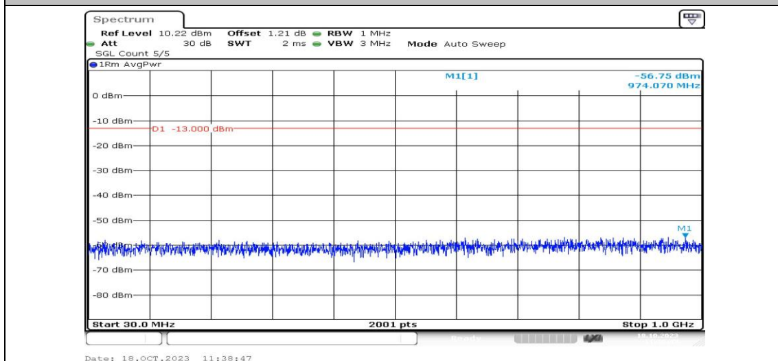
Band2-5MHz-QPSK-18900-1RB#0-Range3:30~1000MHz-PASS
