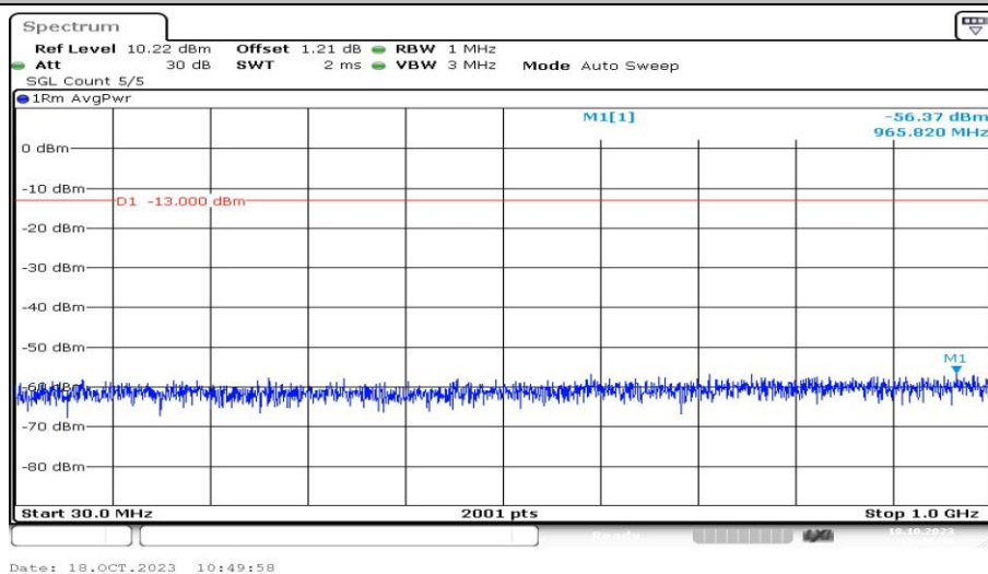
Band2-1.4MHz-QPSK-18900-1RB#0-Range3:30~1000MHz-PASS
