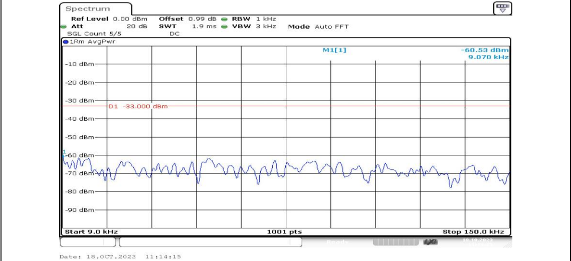
Band2-3MHz-16QAM-18900-1RB#0-Range1:0.009~0.15MHz-PASS
