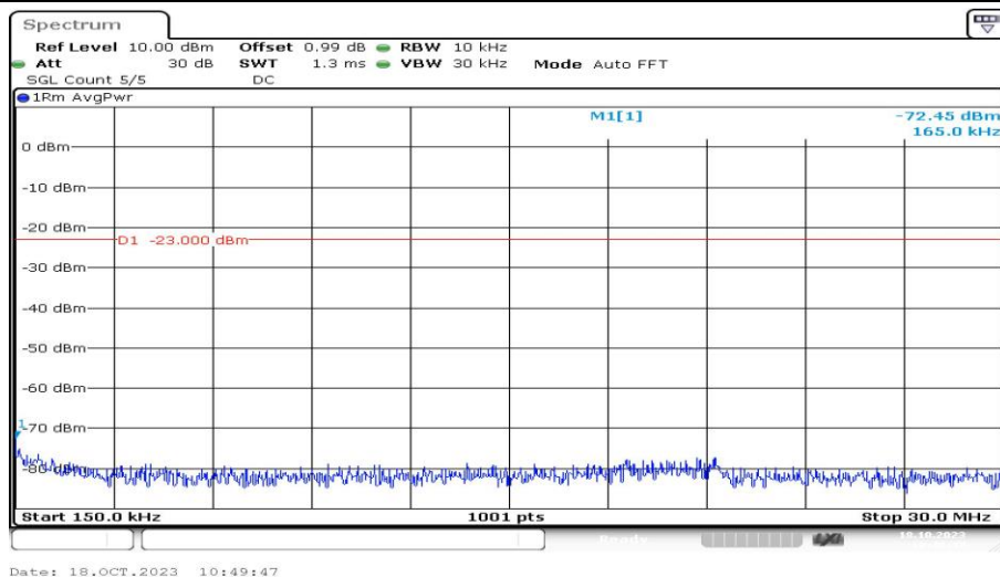
Band2-1.4MHz-QPSK-18900-1RB#0-Range2:0.15~30MHz-PASS
