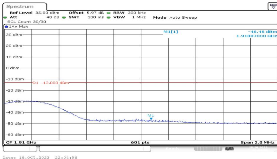
Band2-15MHz-16QAM-19125-1RB#0-PASS
