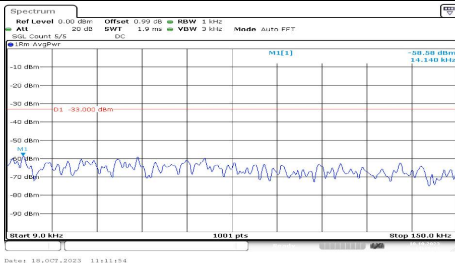
Band2-3MHz-QPSK-18615-1RB#0-Range1:0.009~0.15MHz-PASS
