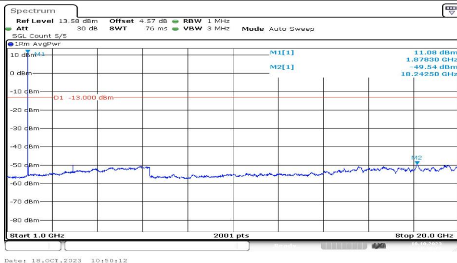
Band2-1.4MHz-QPSK-18900-1RB#0-Range4:1000~20000MHz-PASS
