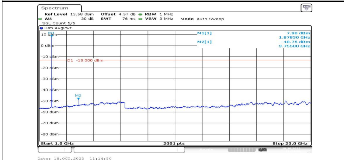
Band2-3MHz-16QAM-18900-1RB#0-Range4:1000~20000MHz-PASS
