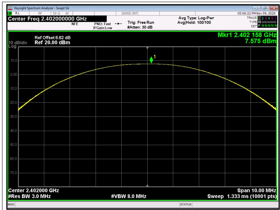
(Channel 0, 2402MHz)
