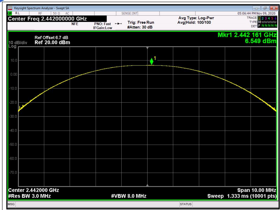
(Channel 20, 2442MHz)
