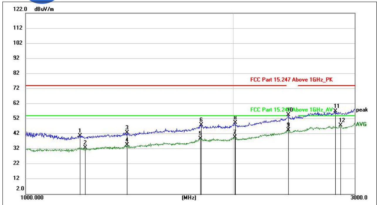
(LE 1M PHY _2442MHz, Antenna Horizontal, 1GHz to 3GHz)
