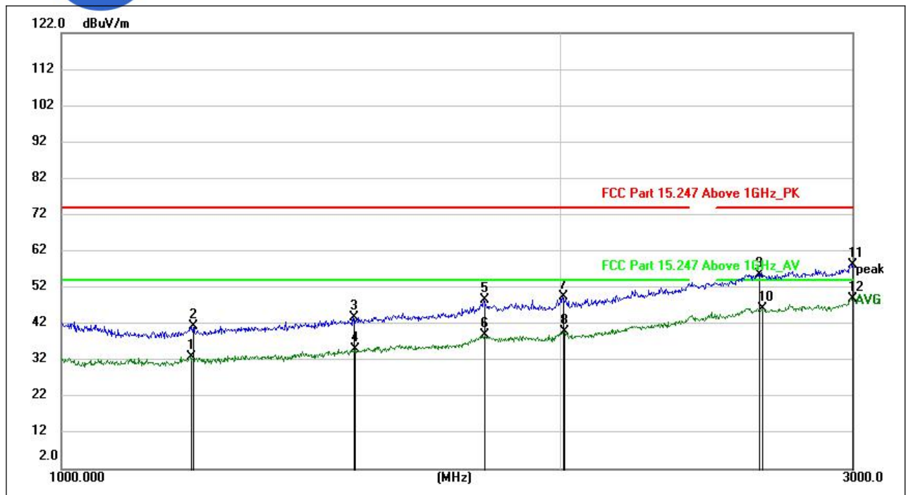
(LE 1M PHY _2442MHz, Antenna Vertical , 1GHz to 3GHz)
