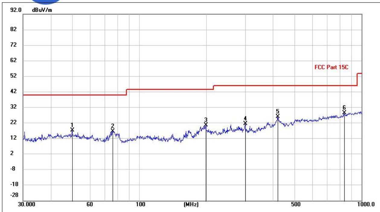
(LE 1M PHY_2442MHz, Antenna Horizontal, 30MHz to 1GHz)
