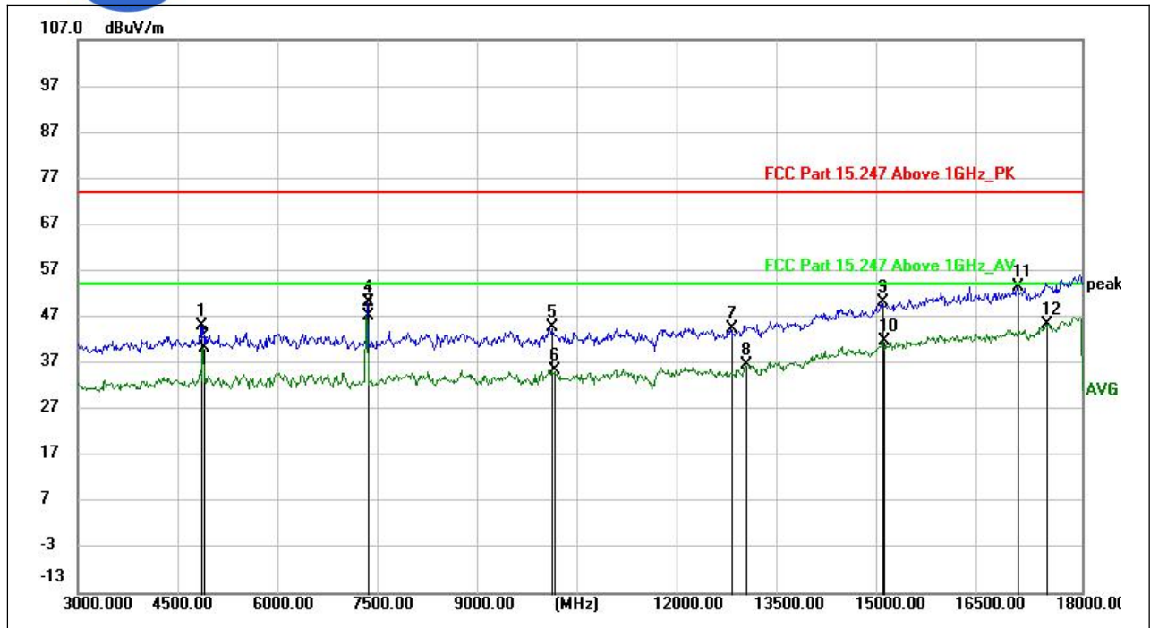
(LE 1M PHY _2442MHz, Antenna Vertical, 3GHz to 18GHz)
