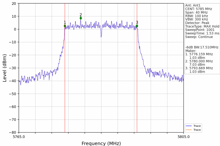
802.11ax(HEW20)_MCH_5785MHz_RU242_Left_Ant1_NTNV
