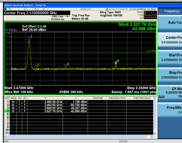
BLE_1M-Ant1-High-2480-1.80
