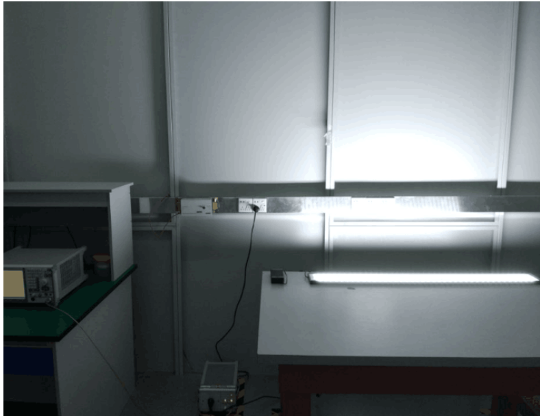
Radiated Emissions
