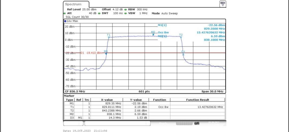
Band26-15MHz-QPSK-26965-75RB#0
