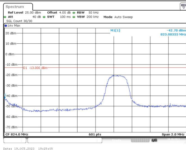
Band26-3MHz-QPSK-26805-15RB#0
