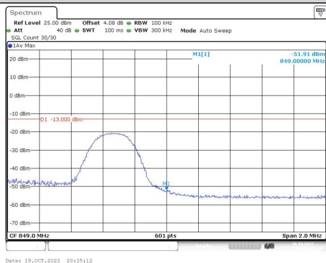
Band26-5MHz-QPSK-27015-1RB#24
