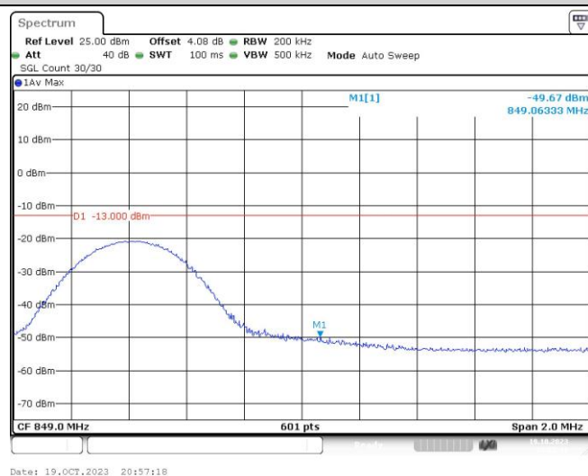
Band26-10MHz-QPSK-26990-1RB#49
