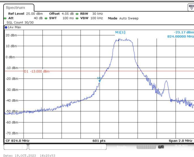
Band26-1.4MHz-16QAM-26797-1RB#5
