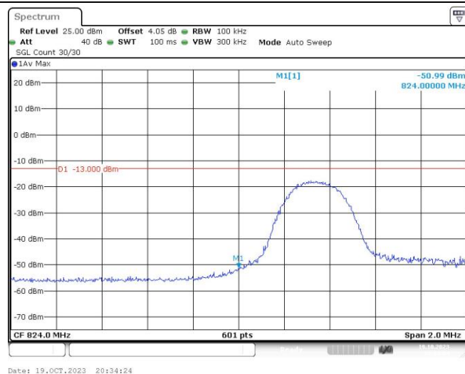
Band26-5MHz-16QAM-26815-25RB#0
