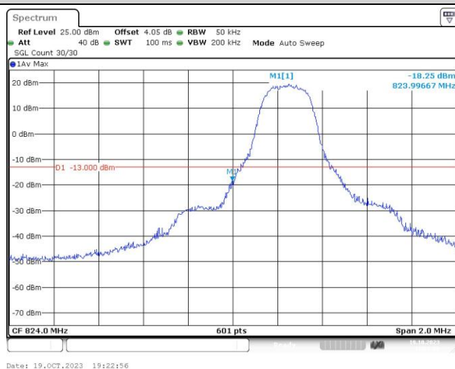
Band26-3MHz-QPSK-26805-1RB#14
