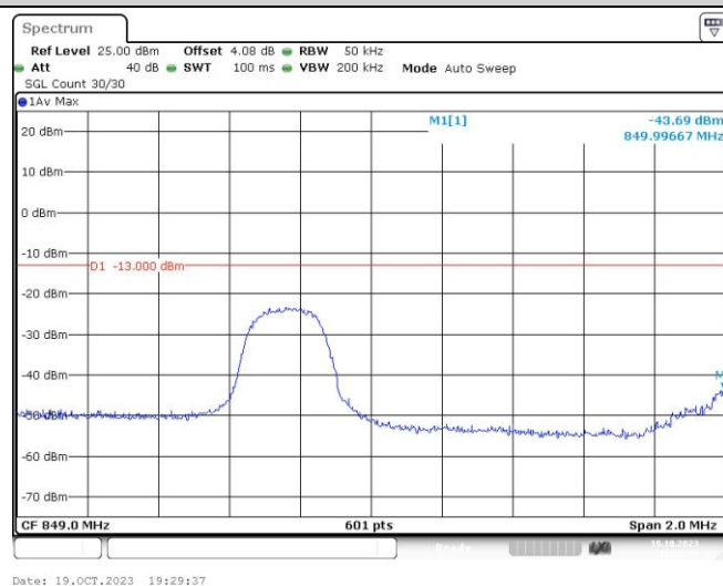
Band26-3MHz-QPSK-27025-1RB#14
