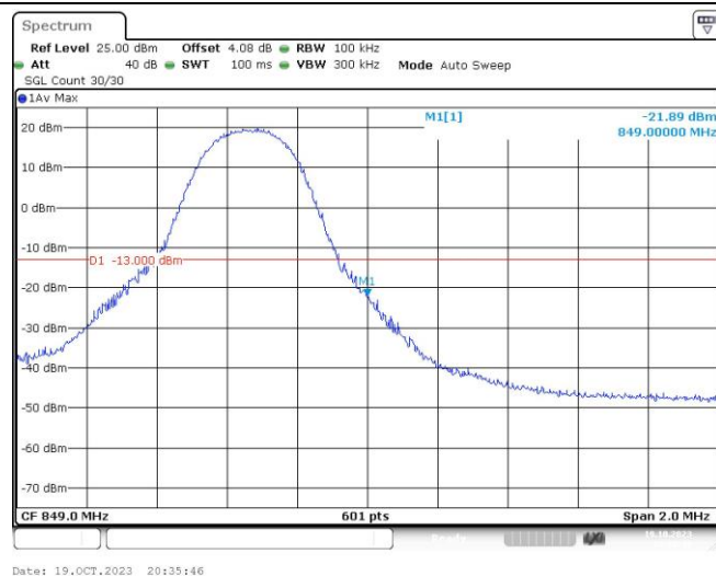
Band26-5MHz-16QAM-27015-25RB#0
