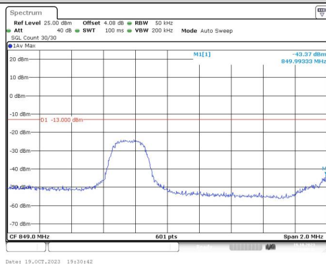
Band26-3MHz-16QAM-27025-1RB#14
