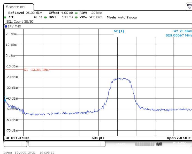
Band26-3MHz-16QAM-26805-15RB#0
