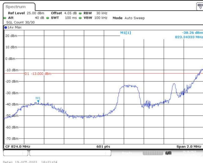
Band26-1.4MHz-QPSK-26797-6RB#0
