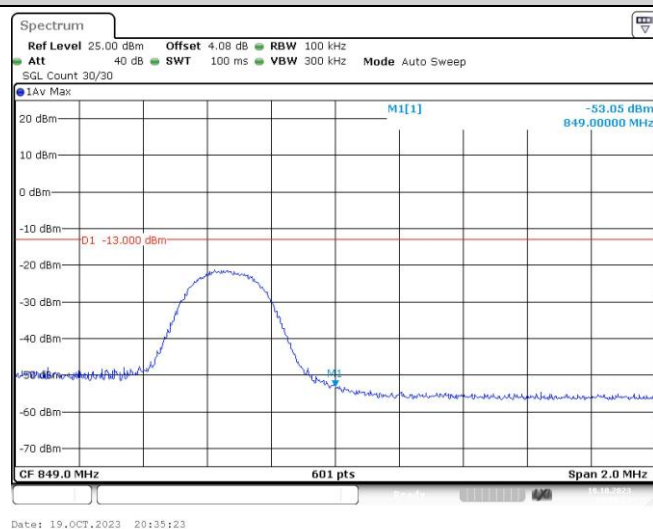
Band26-5MHz-16QAM-27015-1RB#24
