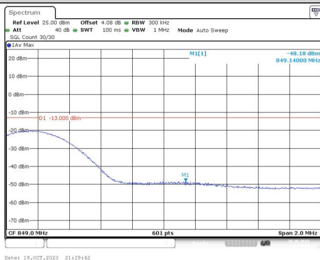
Band26-15MHz-16QAM-26965-1RB#74
