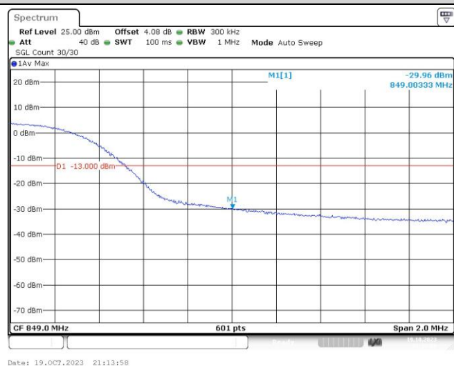
Band26-15MHz-16QAM-26865-1RB#0
