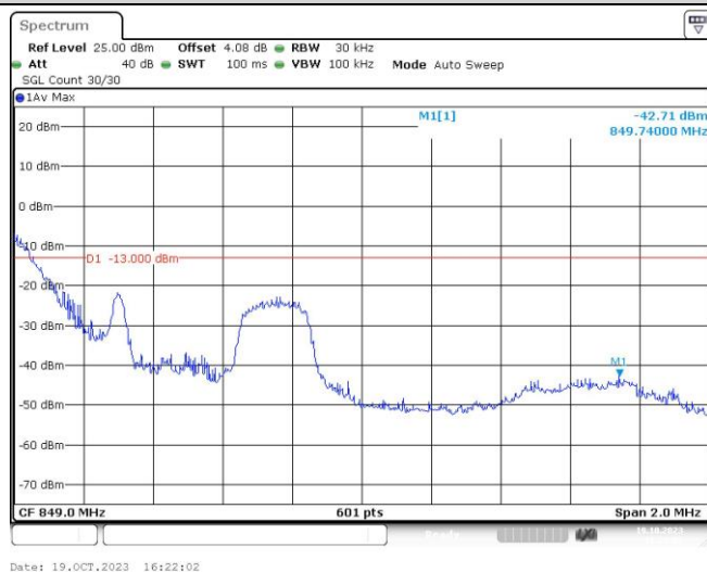
Band26-1.4MHz-QPSK-27033-1RB#5
