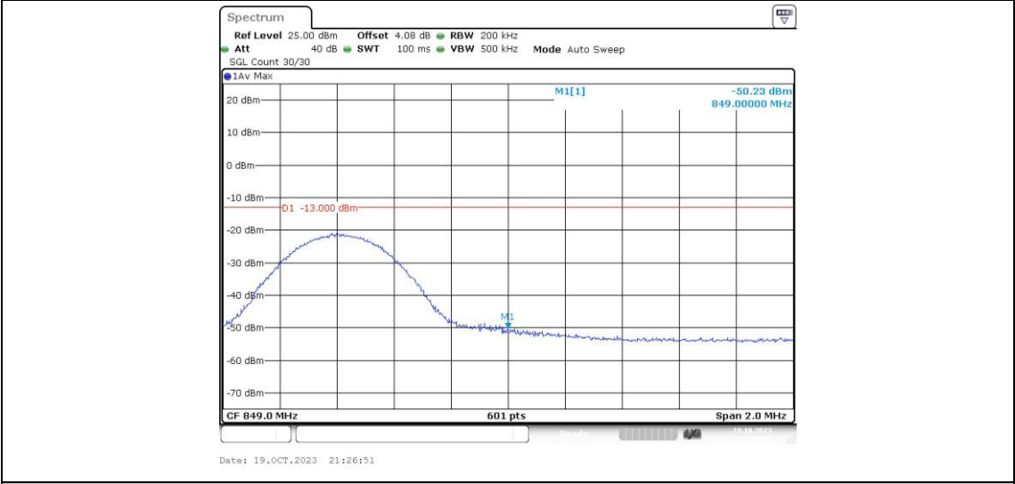
Band26-10MHz-16QAM-26990-1RB#49
