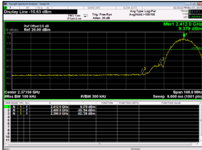
Bandedge-CH01
