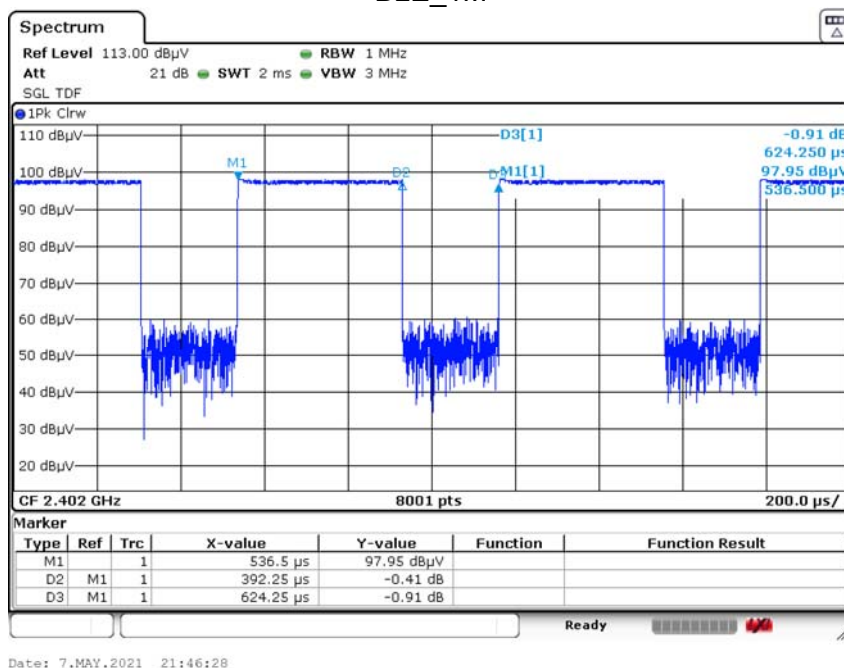
BLE_1M
