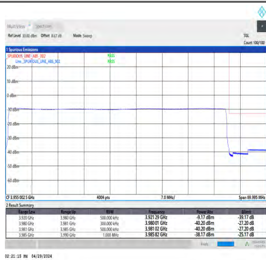
1-N77-3700-3980-30-60-L-6-CP-QPSK-Outer _Full-162@0-Ant1-1--PASS-see graph
