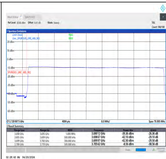
1-N77-3700-3980-30-70-L-6-CP-QPSK-Outer _Full-189@0-Ant1-1--PASS-see graph
