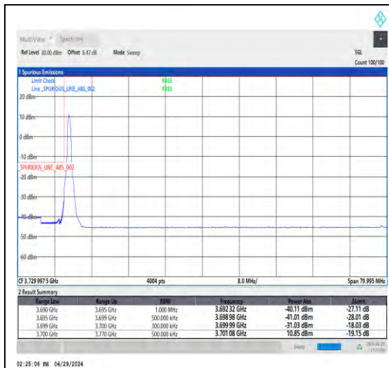
1-N77-3700-3980-30-70-L-4-CP-QPSK-Edge _1RB_Left-1@0-Ant1-1--PASS-see graph
