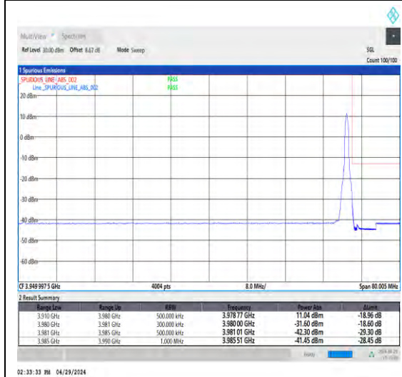
1-N77-3700-3980-30-70-H-5-CP-QPSK-Edge _1RB_Right-1@188-Ant1-1--PASS-see graph
