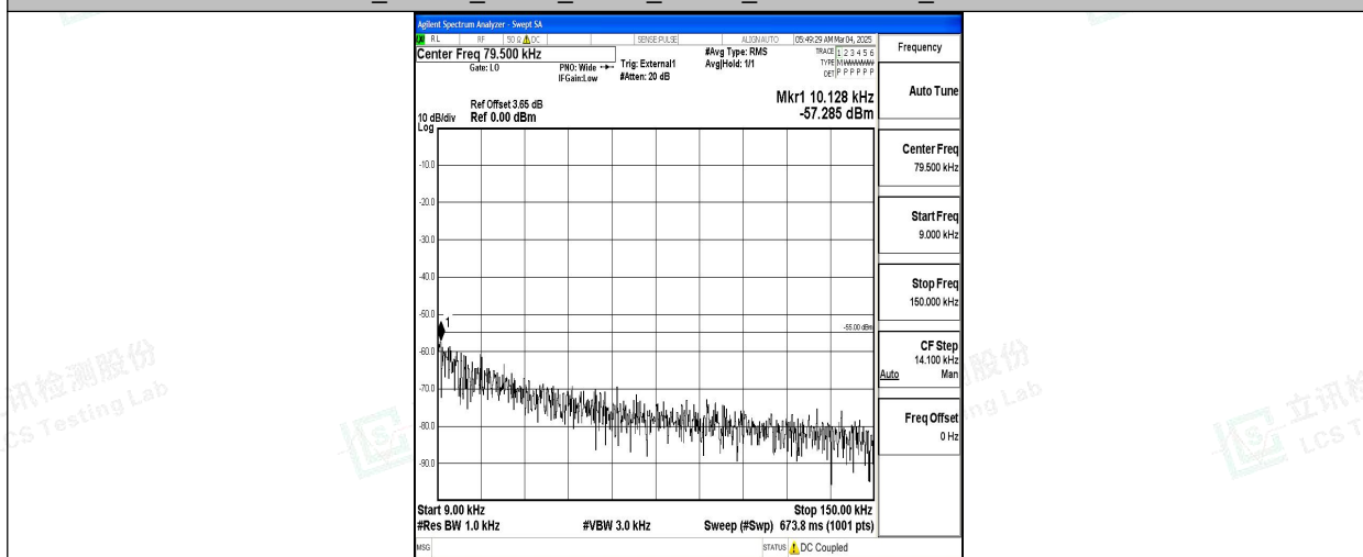
Band38_15MHz_16QAM_38175_1RB#0_0.009~0.15_0.009~0.15
