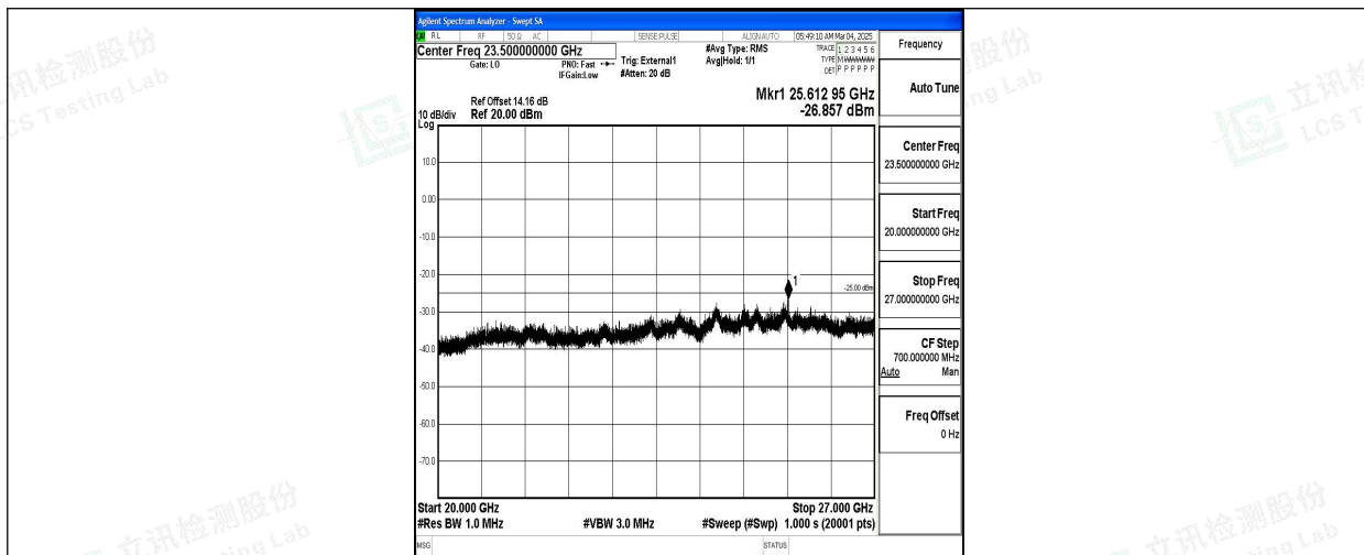
Band38_15MHz_QPSK_38175_1RB#0_20000~27000_20000~27000
