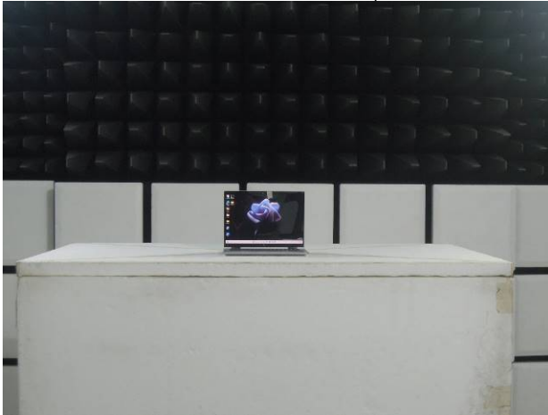
FCC_22_24_27_2G_Setup
