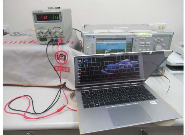
FCC_22_24_27_2G_Conducted Setup
