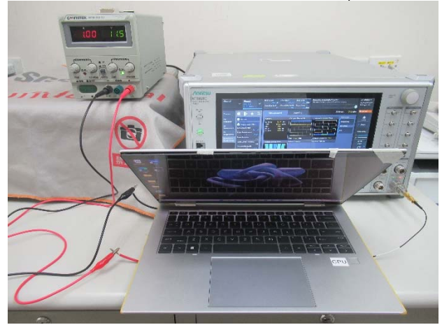
FCC_22_24_27_Cat-M1_Conducted Setup
