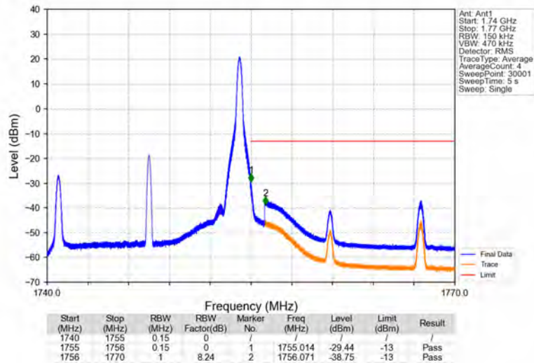
Band4_15MHz_16QAM_HCH_1747.5MHz_RB_1_74_NTNV
