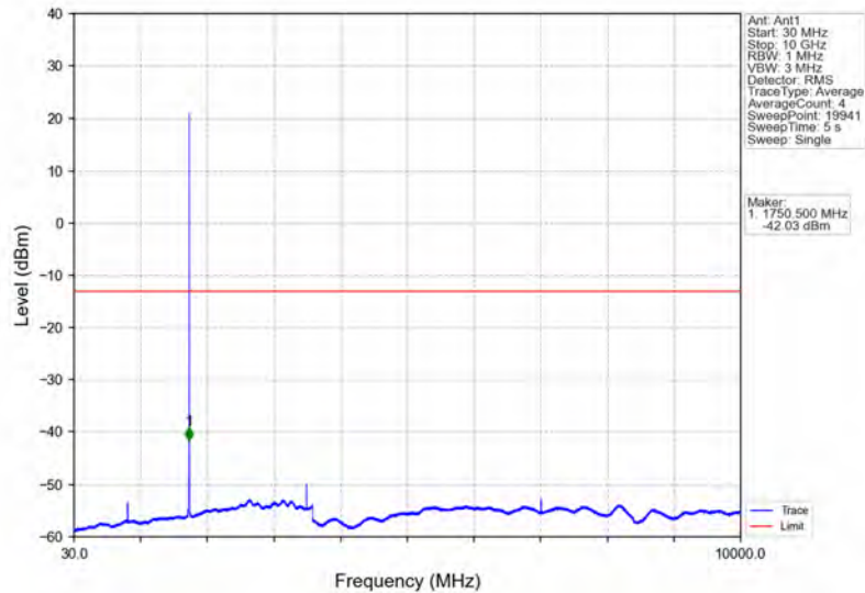
Band4_1.4MHz_16QAM_HCH_1754.3MHz_RB_1_0_NTNV
