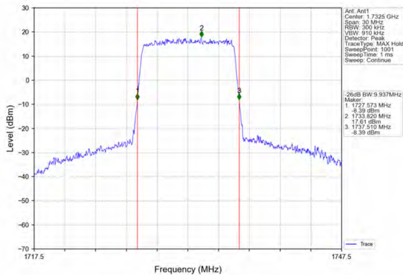
Band4_10MHz_16QAM_MCH_1732.5MHz_RB_50_0_NTNV
