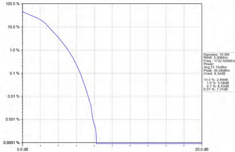
Band4_5MHz_16QAM_MCH_1732.5MHz_RB_25_0_NTNV
