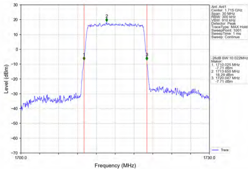
Band4_10MHz_QPSK_LCH_1715MHz_RB_50_0_NTNV
