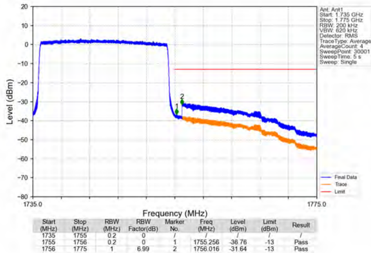
Band4_20MHz_64QAM_HCH_1745MHz_RB_100_0_NTNV
