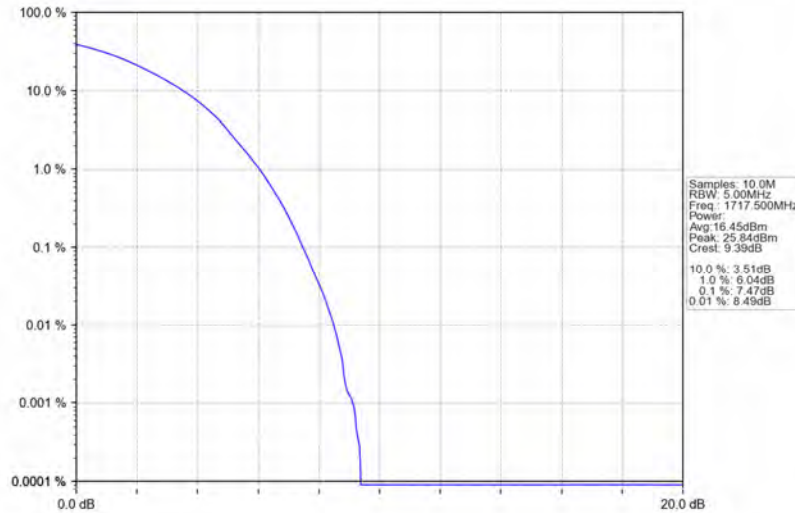
Band4_15MHz_64QAM_LCH_1717.5MHz_RB_75_0_NTNV
