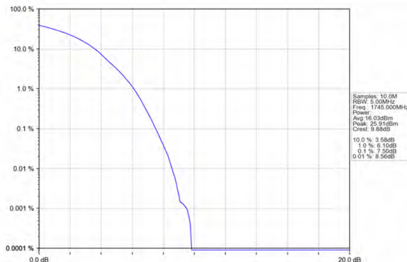
Band4_20MHz_16QAM_HCH_1745MHz_RB_100_0_NTNV
