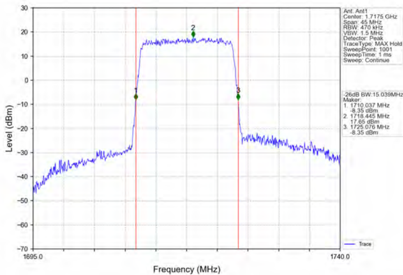
Band4_15MHz_16QAM_LCH_1717.5MHz_RB_75_0_NTNV
