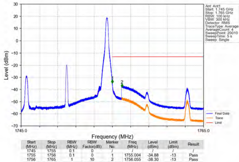
Band4_10MHz_64QAM_HCH_1750MHz_RB_1_49_NTNV
