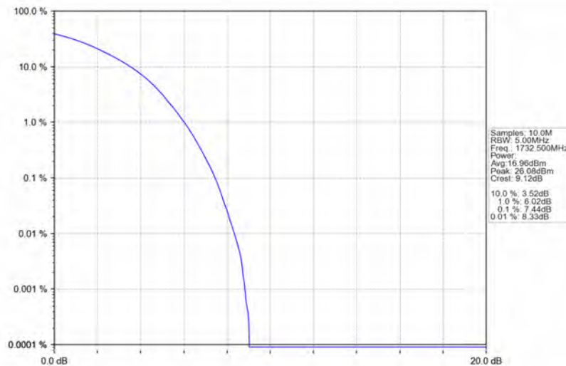
Band4_15MHz_64QAM_MCH_1732.5MHz_RB_75_0_NTNV
