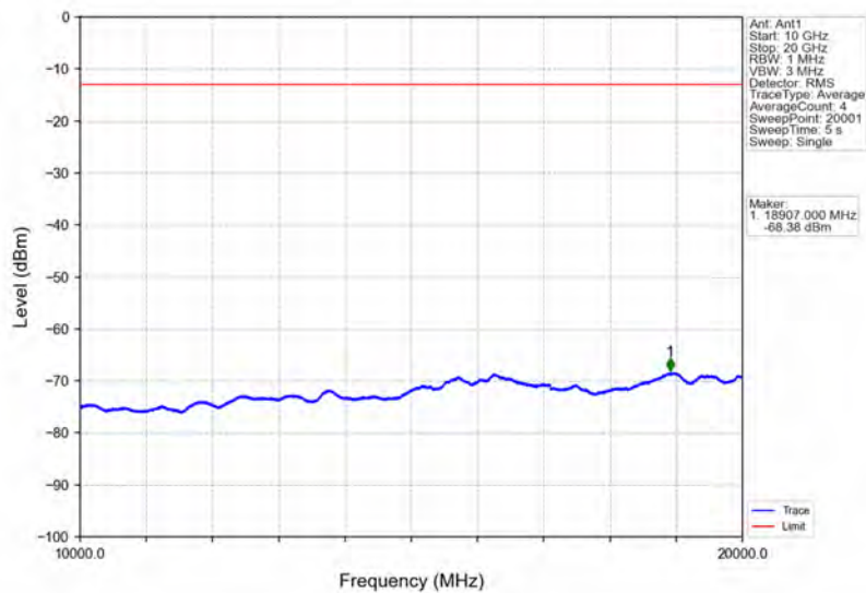
Band4_10MHz_64QAM_HCH_1750MHz_RB_1_0_NTNV
