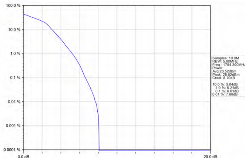
Band4_1.4MHz_16QAM_HCH_1754.3MHz_RB_6_0_NTNV
