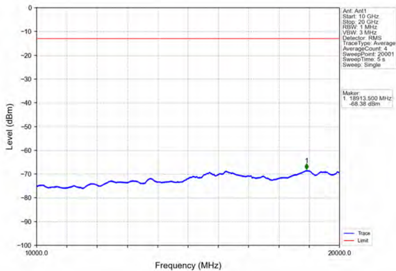
Band4_10MHz_64QAM_MCH_1732.5MHz_RB_1_0_NTNV
