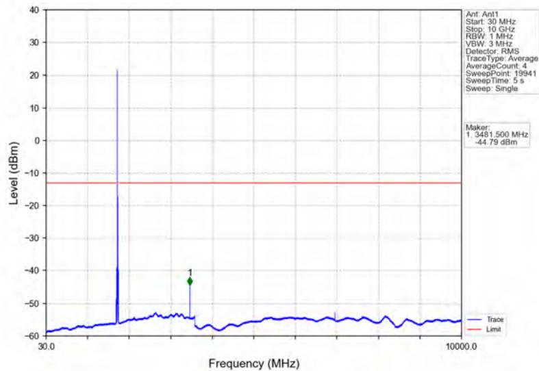
Band4_15MHz_64QAM_HCH_1747.5MHz_RB_1_0_NTNV
