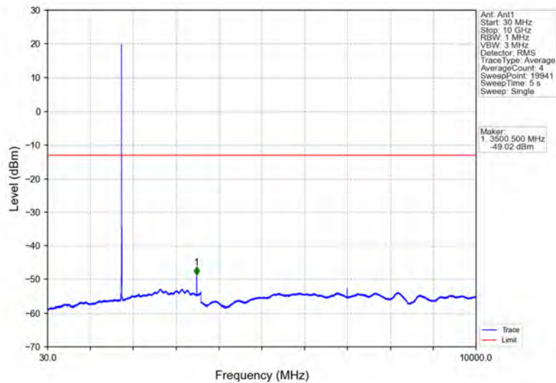
Band4_5MHz_64QAM_HCH_1752.5MHz_RB_1_0_NTNV
