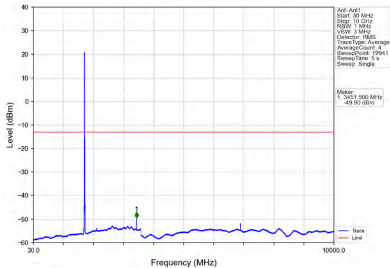
Band4_15MHz_64QAM_MCH_1732.5MHz_RB_1_0_NTNV
