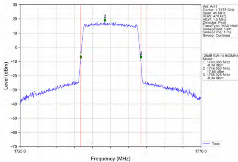
Band4_15MHz_16QAM_HCH_1747.5MHz_RB_75_0_NTNV
