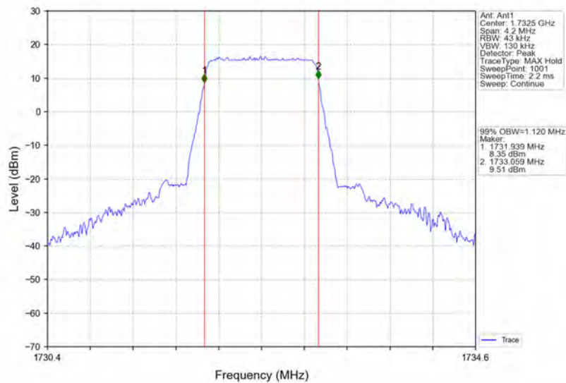
Band4_1.4MHz_64QAM_MCH_1732.5MHz_RB_6_0_NTNV
