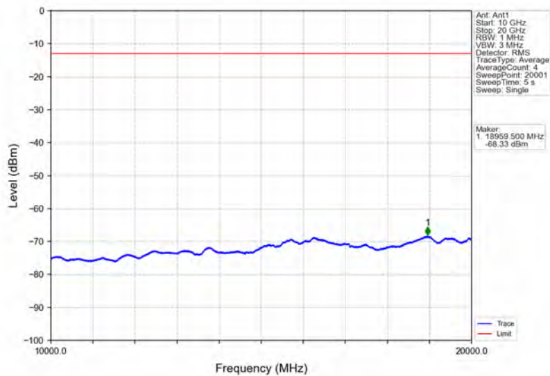
Band4_5MHz_16QAM_MCH_1732.5MHz_RB_1_0_NTNV
