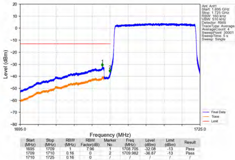
Band4_15MHz_16QAM_LCH_1717.5MHz_RB_75_0_NTNV
