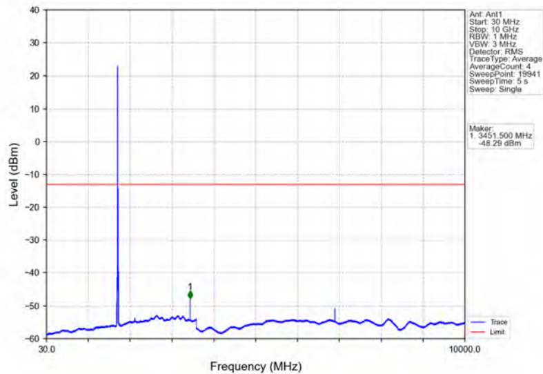
Band4_15MHz_QPSK_MCH_1732.5MHz_RB_1_0_NTNV
