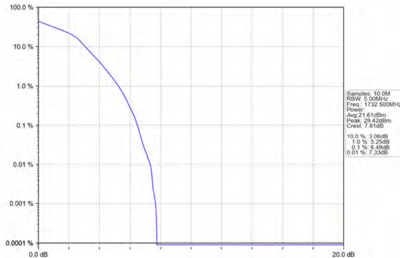
Band4_1.4MHz_16QAM_MCH_1732.5MHz_RB_6_0_NTNV
