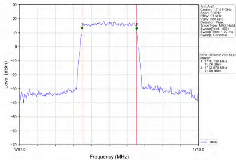
Band4_3MHz_QPSK_LCH_1711.5MHz_RB_15_0_NTNV
