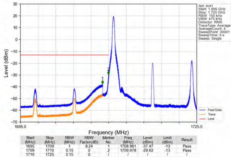
Band4_15MHz_64QAM_LCH_1717.5MHz_RB_1_0_NTNV
