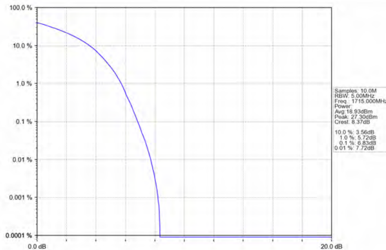
Band4_10MHz_16QAM_LCH_1715MHz_RB_50_0_NTNV
