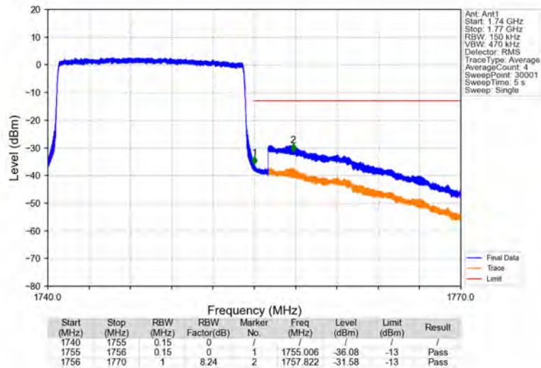
Band4_15MHz_64QAM_HCH_1747.5MHz_RB_75_0_NTNV
