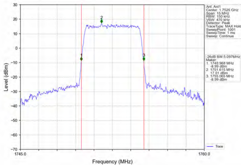
Band4_5MHz_16QAM_HCH_1752.5MHz_RB_25_0_NTNV
