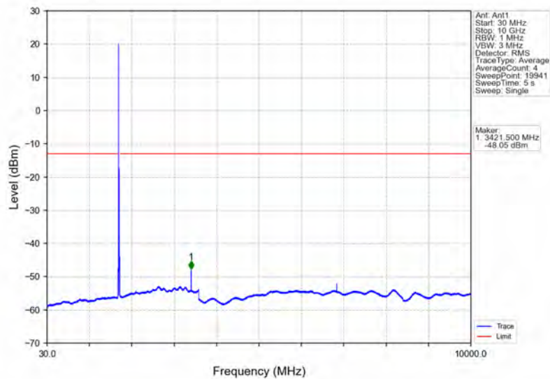
Band4_15MHz_64QAM_LCH_1717.5MHz_RB_1_0_NTNV
