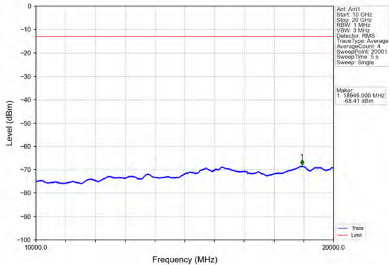
Band4_1.4MHz_QPSK_LCH_1710.7MHz_RB_6_0_NTNV
