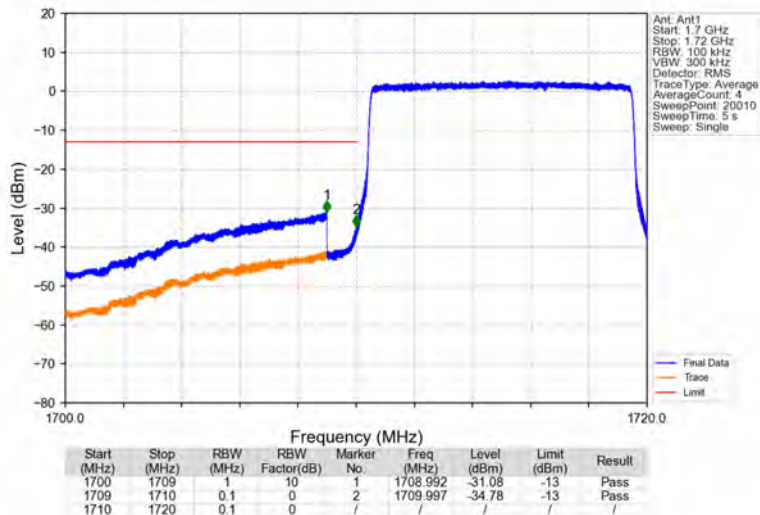
Band4_10MHz_64QAM_LCH_1715MHz_RB_50_0_NTNV
