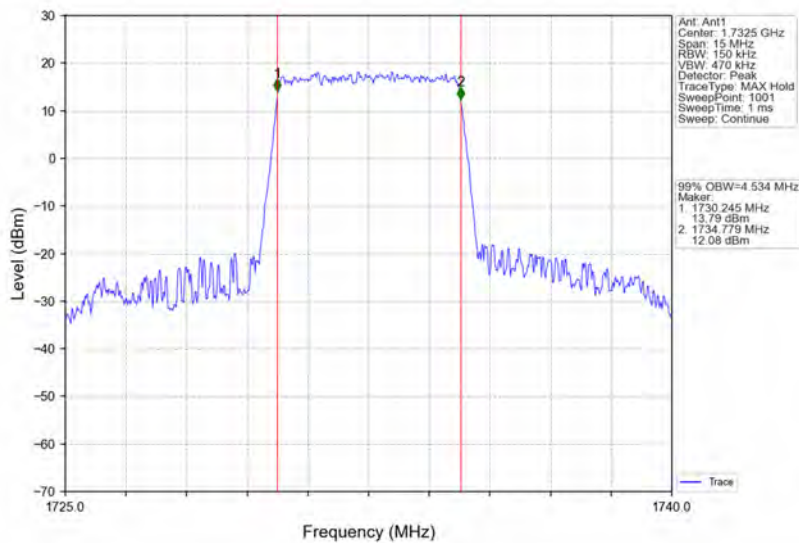
Band4_5MHz_QPSK_MCH_1732.5MHz_RB_25_0_NTNV
