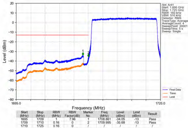
Band4_15MHz_QPSK_LCH_1717.5MHz_RB_75_0_NTNV
