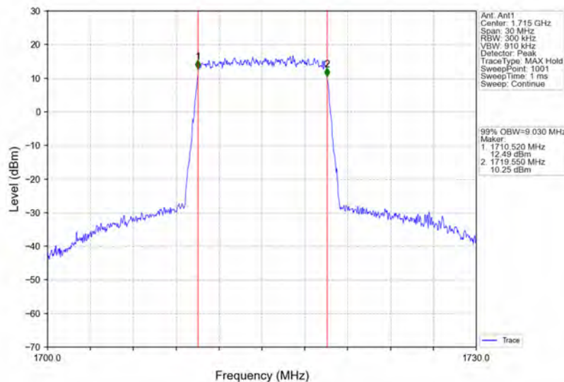
Band4_10MHz_64QAM_LCH_1715MHz_RB_50_0_NTNV
