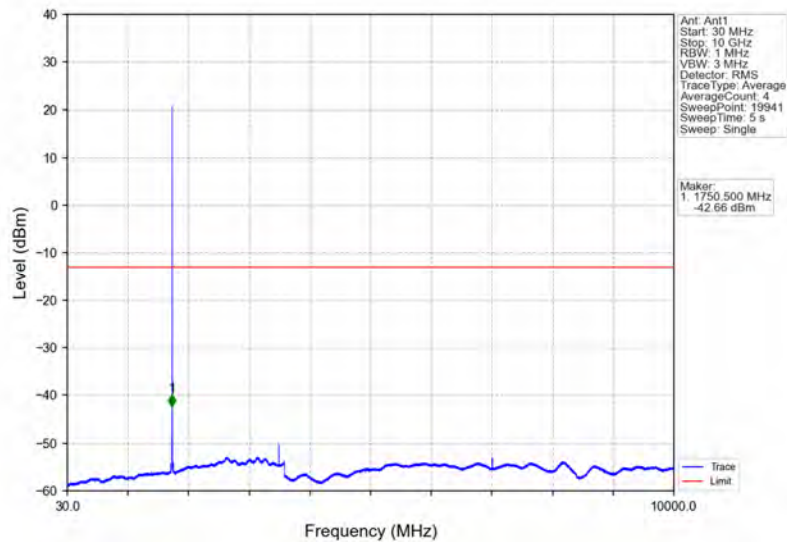
Band4_1.4MHz_64QAM_HCH_1754.3MHz_RB_1_0_NTNV
