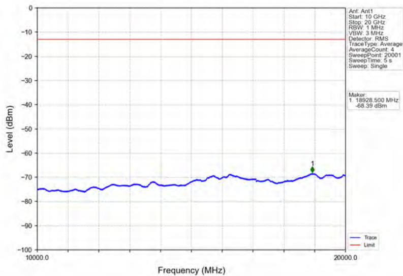
Band4_5MHz_QPSK_HCH_1752.5MHz_RB_1_0_NTNV
