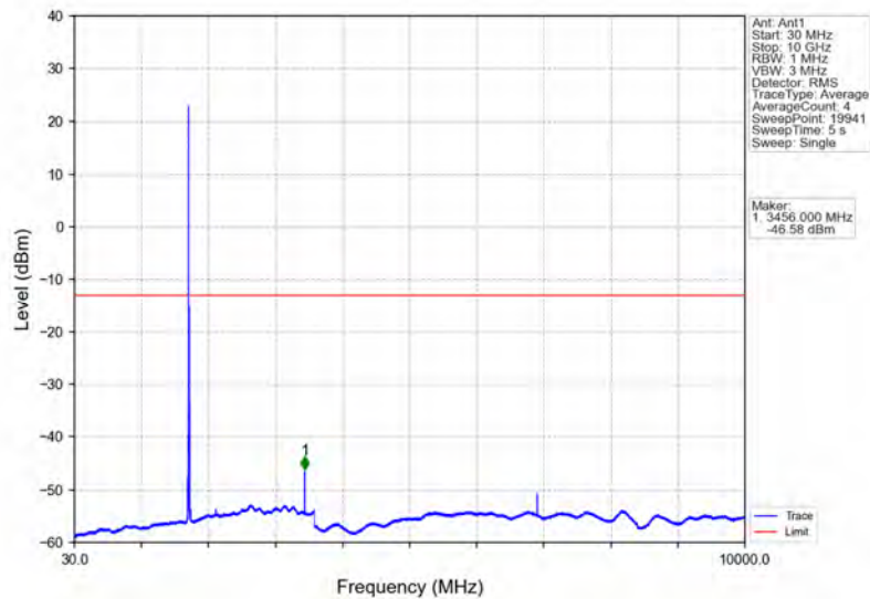
Band4_10MHz_16QAM_MCH_1732.5MHz_RB_1_0_NTNV
