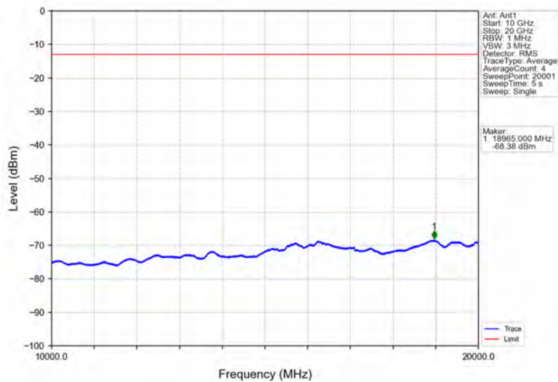
Band4_15MHz_16QAM_MCH_1732.5MHz_RB_1_0_NTNV
