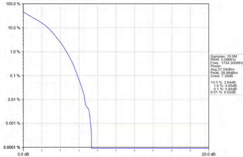
Band4_1.4MHz_QPSK_HCH_1754.3MHz_RB_6_0_NTNV
