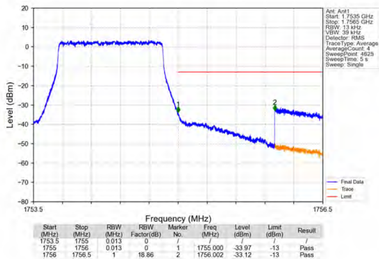
Band4_1.4MHz_16QAM_HCH_1754.3MHz_RB_6_0_NTNV
