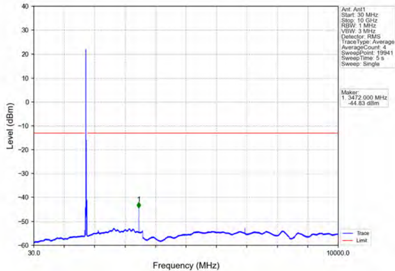
Band4_20MHz_64QAM_HCH_1745MHz_RB_1_0_NTNV
