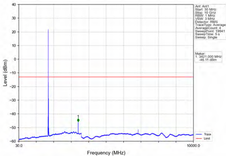
Band4_10MHz_16QAM_LCH_1715MHz_RB_1_0_NTNV
