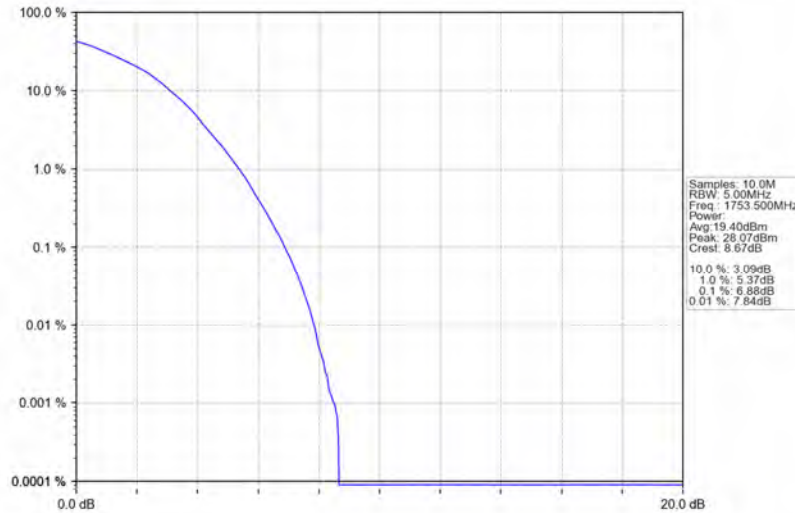
Band4_3MHz_64QAM_HCH_1753.5MHz_RB_15_0_NTNV
