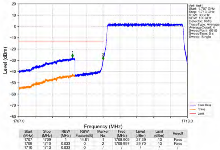
Band4_3MHz_64QAM_LCH_1711.5MHz_RB_15_0_NTNV
