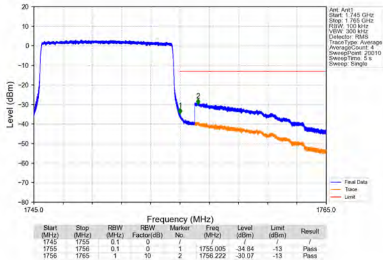
Band4_10MHz_16QAM_HCH_1750MHz_RB_50_0_NTNV
