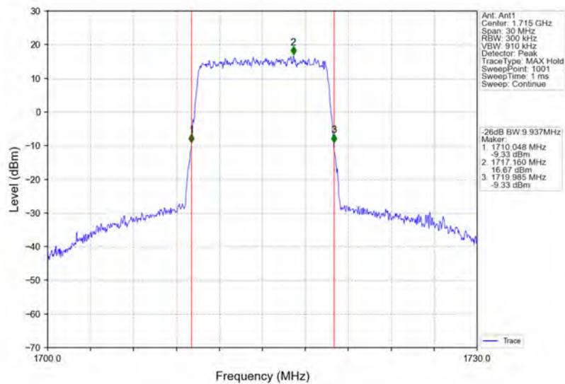
Band4_10MHz_64QAM_LCH_1715MHz_RB_50_0_NTNV
