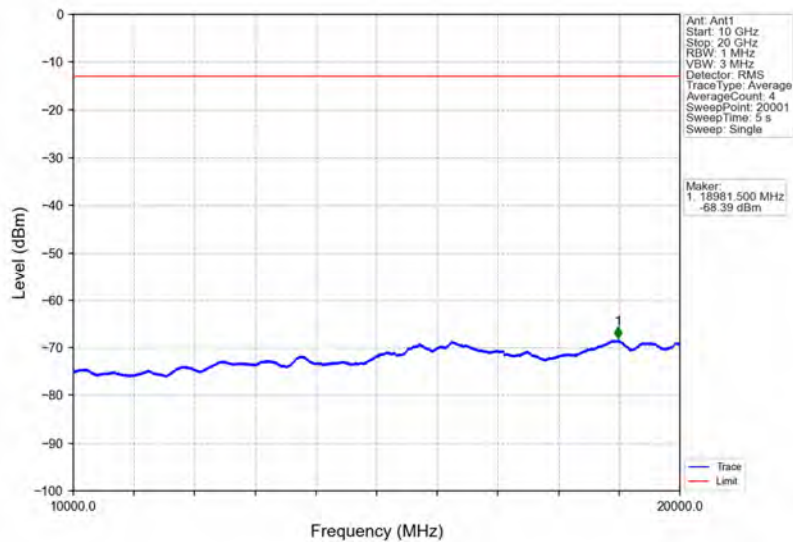
Band4_3MHz_64QAM_LCH_1711.5MHz_RB_15_0_NTNV
