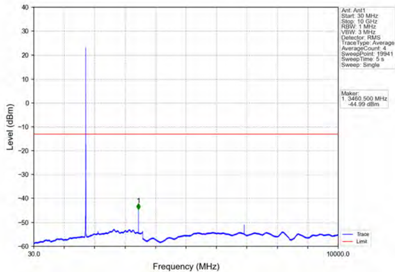
Band4_5MHz_QPSK_MCH_1732.5MHz_RB_1_0_NTNV
