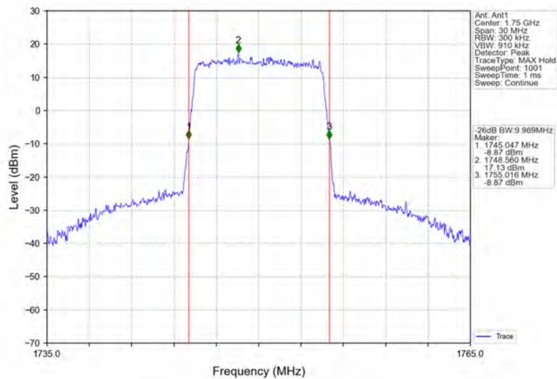
Band4_10MHz_64QAM_HCH_1750MHz_RB_50_0_NTNV
