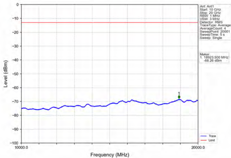
Band4_3MHz_QPSK_MCH_1732.5MHz_RB_1_0_NTNV
