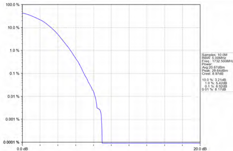
Band4_1.4MHz_64QAM_MCH_1732.5MHz_RB_6_0_NTNV
