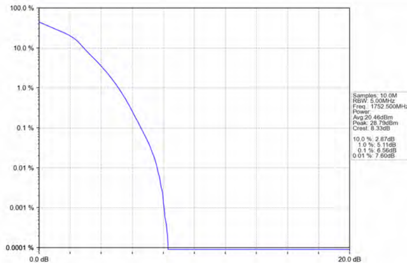
Band4_5MHz_16QAM_HCH_1752.5MHz_RB_25_0_NTNV
