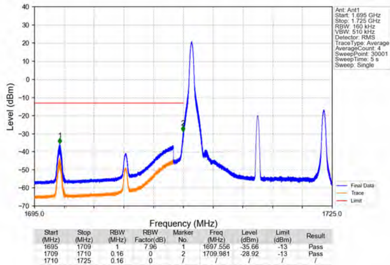
Band4_15MHz_16QAM_LCH_1717.5MHz_RB_1_0_NTNV
