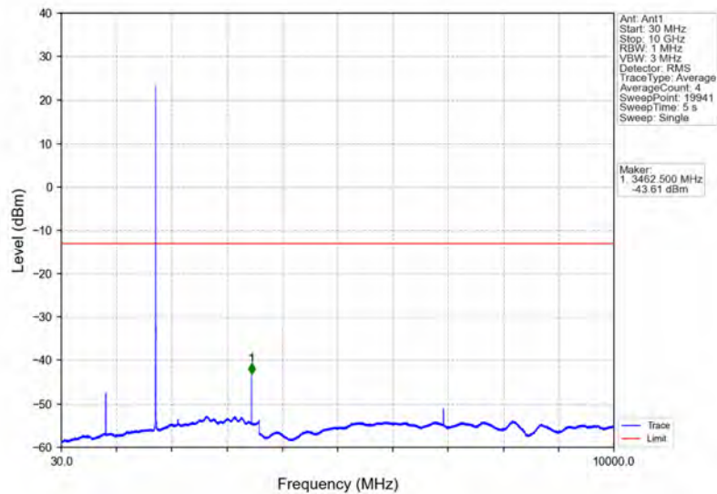
Band4_3MHz_QPSK_MCH_1732.5MHz_RB_1_0_NTNV
