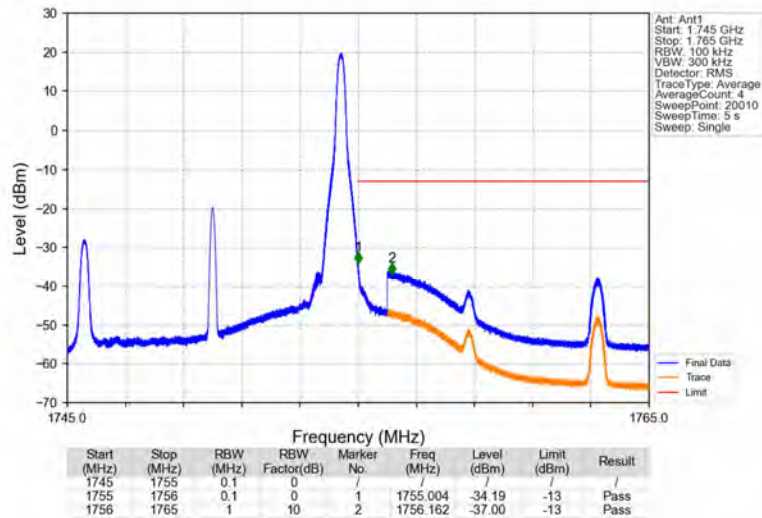
Band4_10MHz_16QAM_HCH_1750MHz_RB_1_49_NTNV
