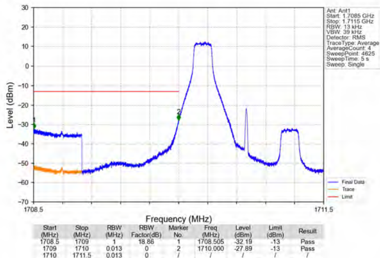
Band4_1.4MHz_16QAM_LCH_1710.7MHz_RB_1_0_NTNV
