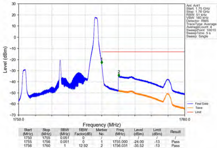
Band4_5MHz_QPSK_HCH_1752.5MHz_RB_1_24_NTNV
