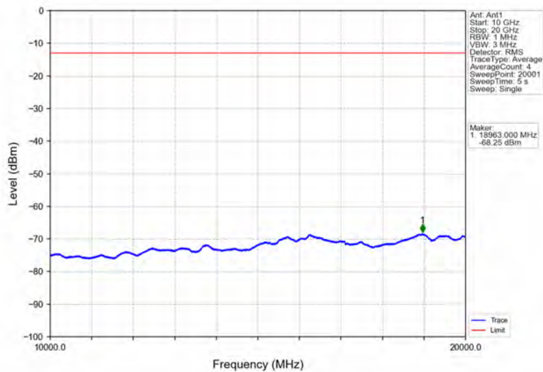
Band4_10MHz_16QAM_MCH_1732.5MHz_RB_1_0_NTNV
