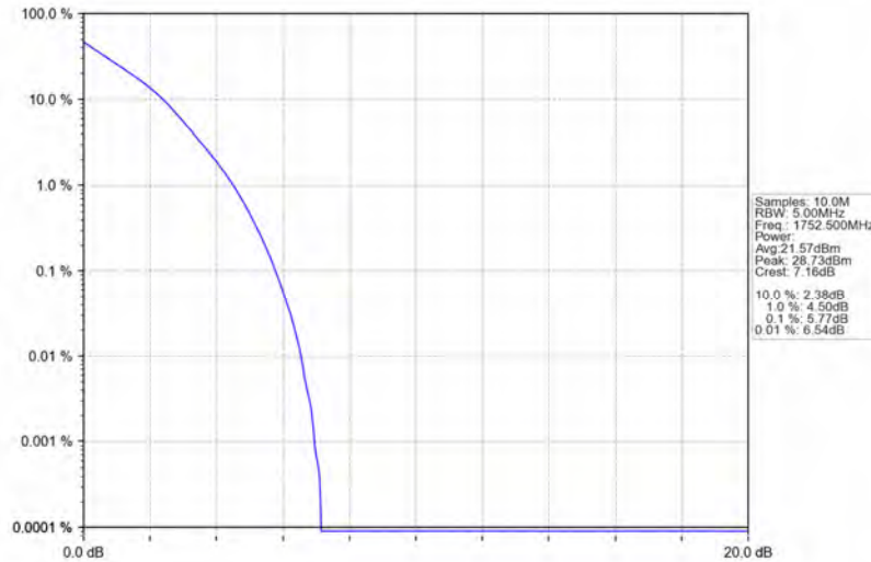
Band4_5MHz_QPSK_HCH_1752.5MHz_RB_25_0_NTNV
