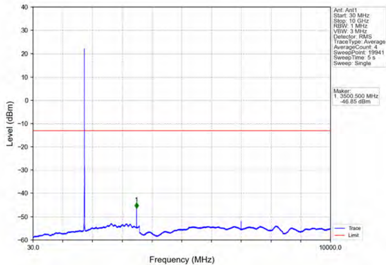
Band4_5MHz_QPSK_HCH_1752.5MHz_RB_1_0_NTNV
