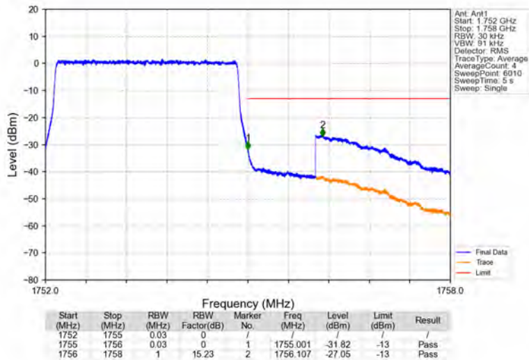
Band4_3MHz_64QAM_HCH_1753.5MHz_RB_15_0_NTNV
