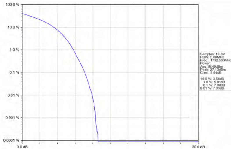
Band4_10MHz_64QAM_MCH_1732.5MHz_RB_50_0_NTNV
