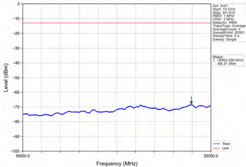
Band4_15MHz_QPSK_LCH_1717.5MHz_RB_75_0_NTNV
