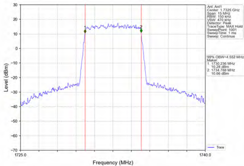
Band4_5MHz_64QAM_MCH_1732.5MHz_RB_25_0_NTNV
