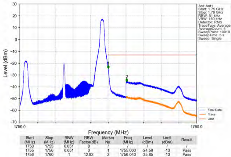
Band4_5MHz_16QAM_HCH_1752.5MHz_RB_1_24_NTNV
