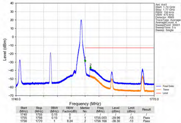
Band4_15MHz_64QAM_HCH_1747.5MHz_RB_1_74_NTNV
