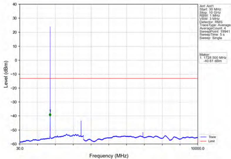
Band4_1.4MHz_QPSK_MCH_1732.5MHz_RB_1_0_NTNV
