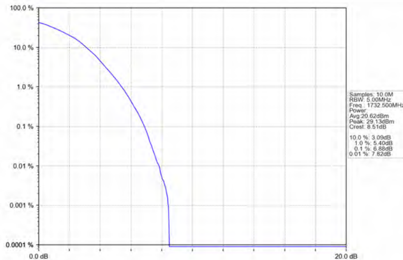
Band4_3MHz_64QAM_MCH_1732.5MHz_RB_15_0_NTNV
