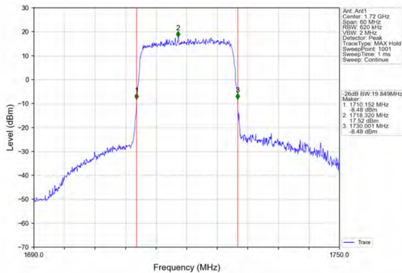
Band4_20MHz_64QAM_LCH_1720MHz_RB_100_0_NTNV
