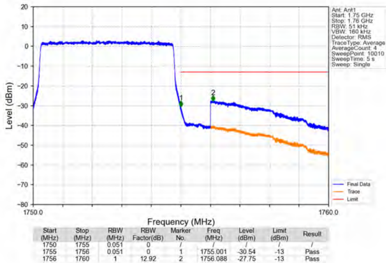
Band4_5MHz_16QAM_HCH_1752.5MHz_RB_25_0_NTNV
