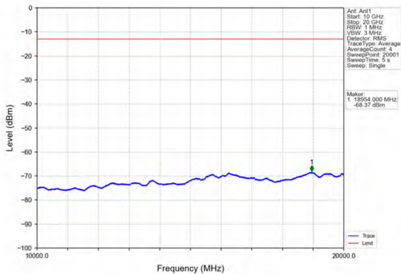
Band4_15MHz_QPSK_MCH_1732.5MHz_RB_1_0_NTNV
