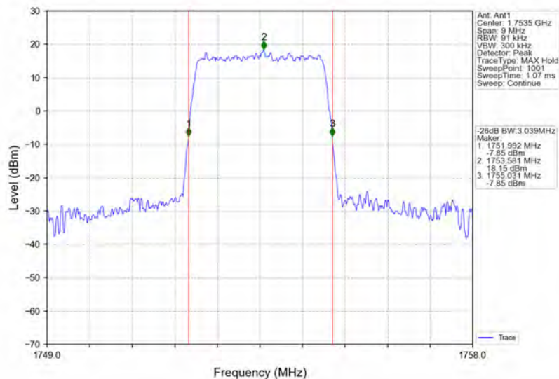
Band4_3MHz_QPSK_HCH_1753.5MHz_RB_15_0_NTNV
