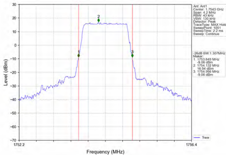
Band4_1.4MHz_16QAM_HCH_1754.3MHz_RB_6_0_NTNV
