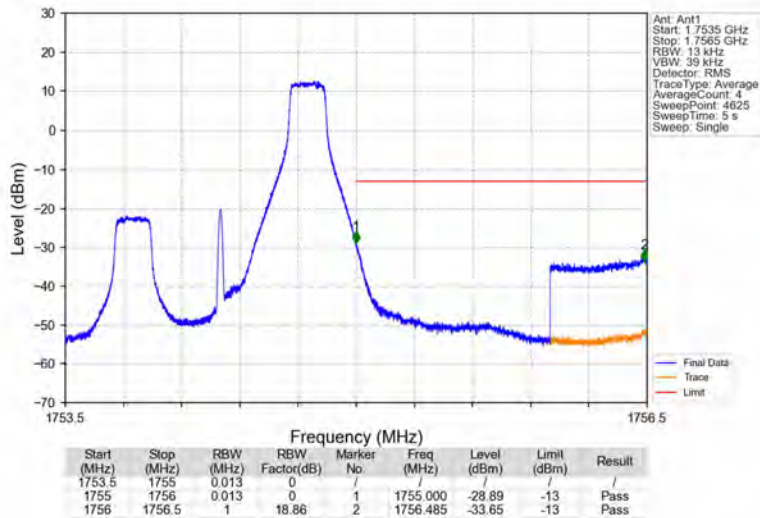
Band4_1.4MHz_QPSK_HCH_1754.3MHz_RB_1_5_NTNV
