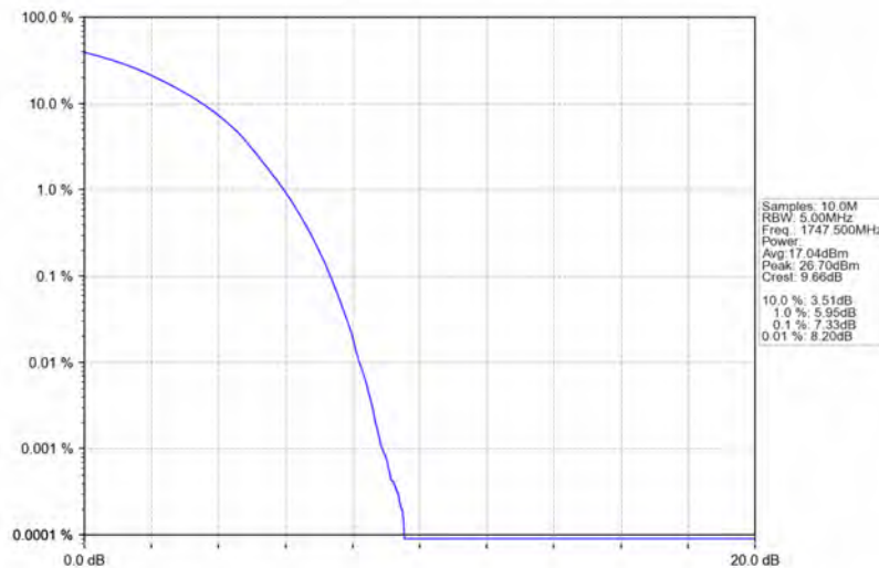
Band4_15MHz_16QAM_HCH_1747.5MHz_RB_75_0_NTNV
