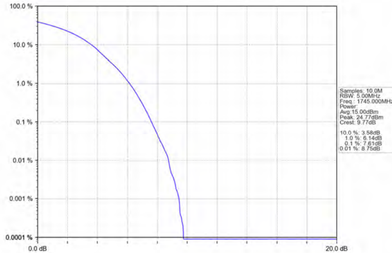
Band4_20MHz_64QAM_HCH_1745MHz_RB_100_0_NTNV
