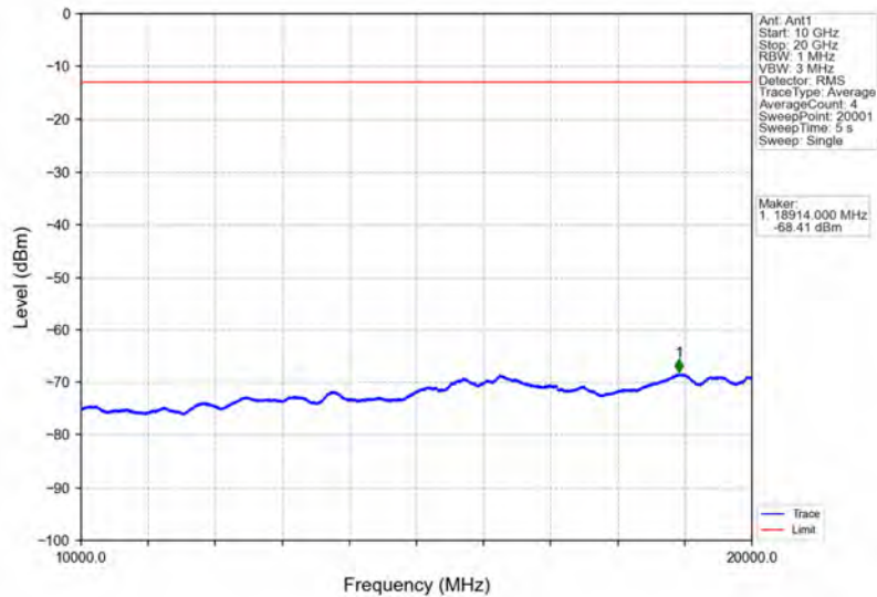
Band4_10MHz_16QAM_LCH_1715MHz_RB_50_0_NTNV
