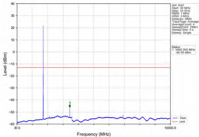
Band4_5MHz_64QAM_MCH_1732.5MHz_RB_1_0_NTNV
