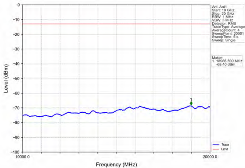
Band4_1.4MHz_16QAM_MCH_1732.5MHz_RB_1_0_NTNV
