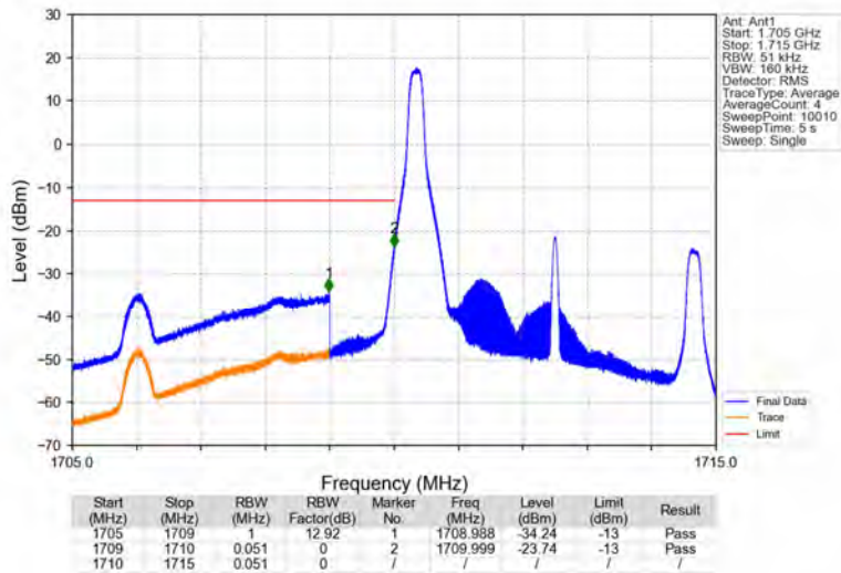
Band4_5MHz_16QAM_LCH_1712.5MHz_RB_1_0_NTNV
