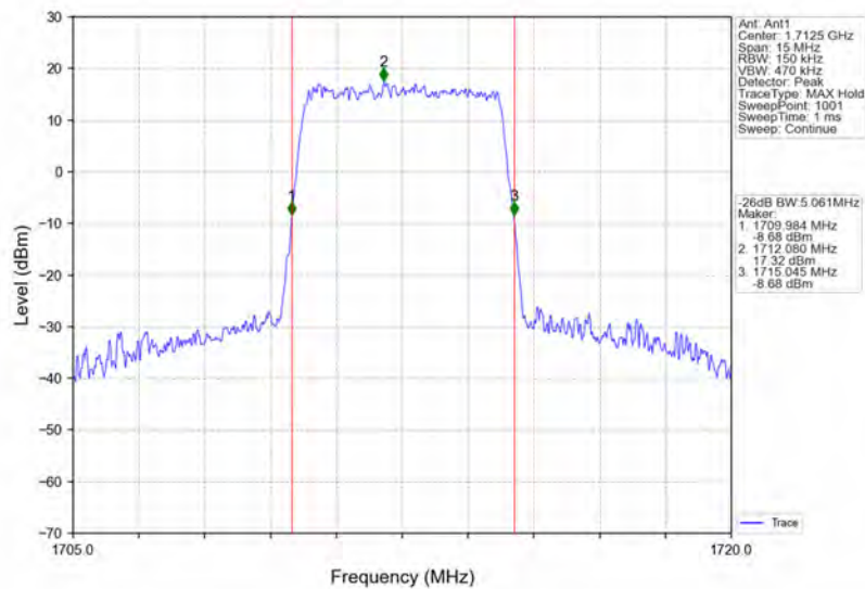
Band4_5MHz_16QAM_LCH_1712.5MHz_RB_25_0_NTNV
