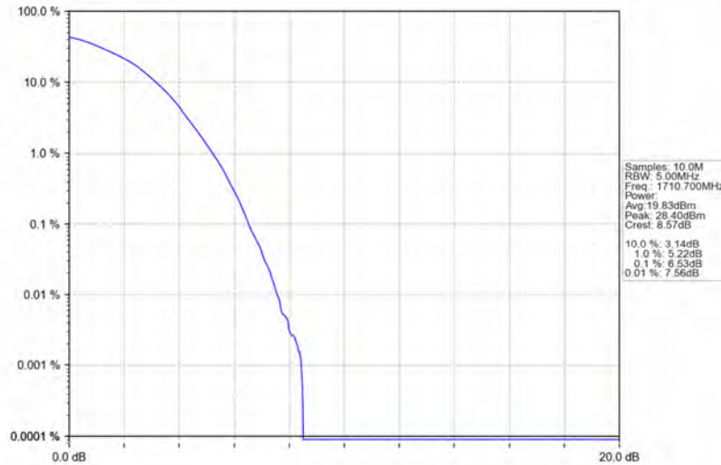
Band4_1.4MHz_64QAM_LCH_1710.7MHz_RB_6_0_NTNV
