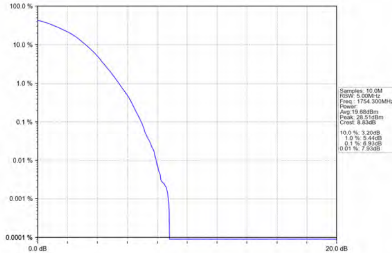
Band4_1.4MHz_64QAM_HCH_1754.3MHz_RB_6_0_NTNV
