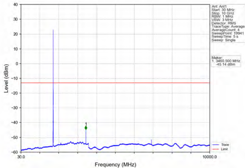
Band4_5MHz_16QAM_MCH_1732.5MHz_RB_1_0_NTNV
