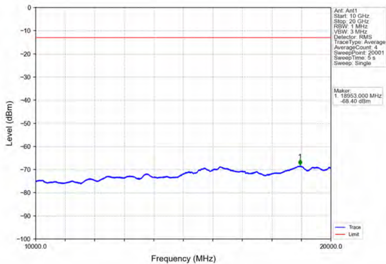
Band4_5MHz_64QAM_HCH_1752.5MHz_RB_1_0_NTNV
