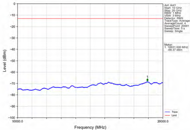
Band4_10MHz_16QAM_HCH_1750MHz_RB_1_0_NTNV
