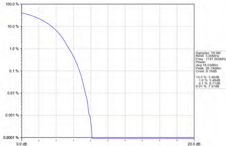
Band4_15MHz_QPSK_HCH_1747.5MHz_RB_75_0_NTNV
