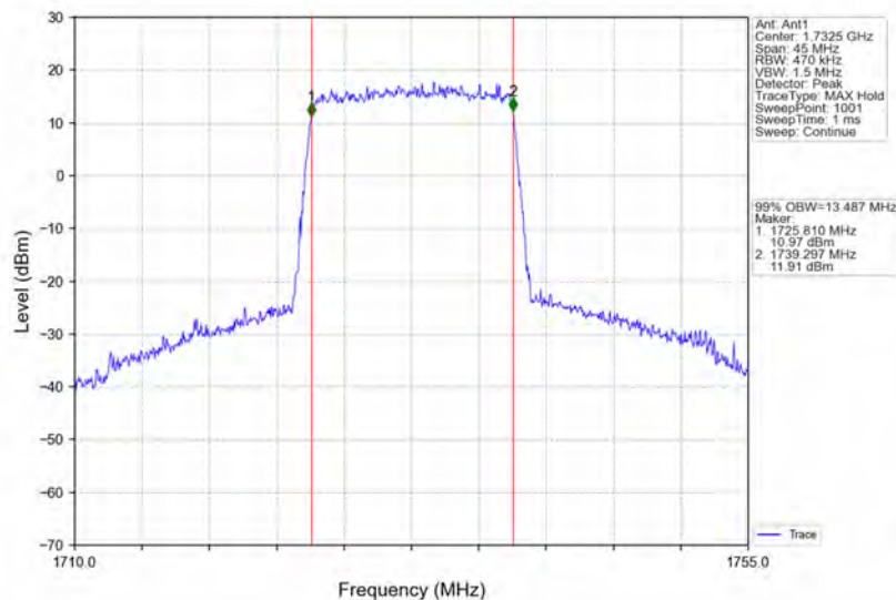
Band4_15MHz_64QAM_MCH_1732.5MHz_RB_75_0_NTNV
