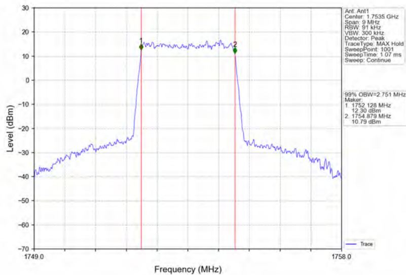
Band4_3MHz_64QAM_HCH_1753.5MHz_RB_15_0_NTNV
