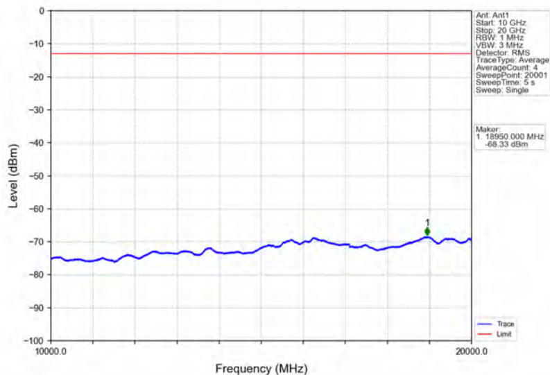
Band4_10MHz_QPSK_MCH_1732.5MHz_RB_1_0_NTNV
