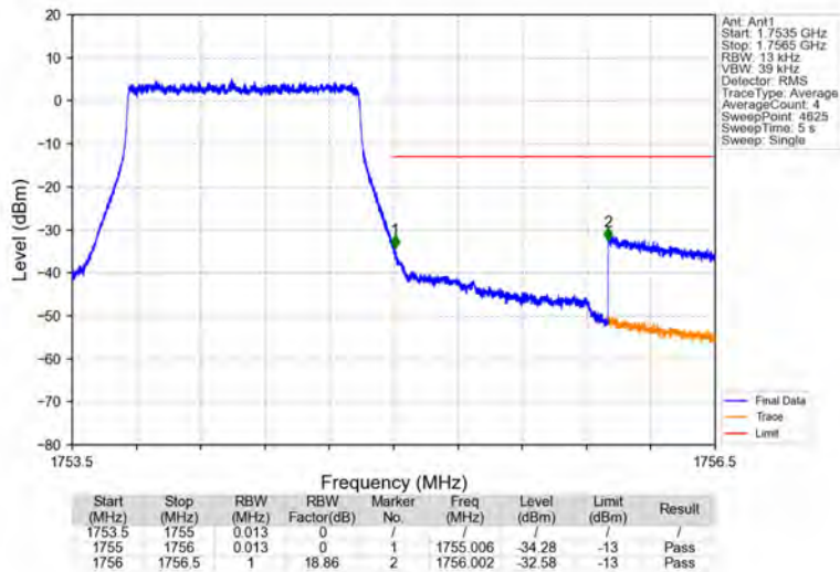
Band4_1.4MHz_QPSK_HCH_1754.3MHz_RB_6_0_NTNV
