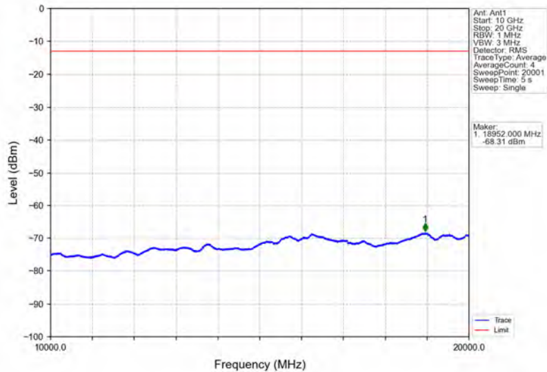
Band4_1.4MHz_16QAM_LCH_1710.7MHz_RB_6_0_NTNV
