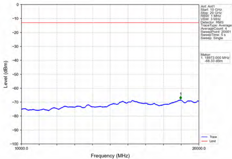
Band4_1.4MHz_64QAM_HCH_1754.3MHz_RB_1_0_NTNV
