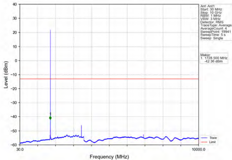
Band4_1.4MHz_64QAM_MCH_1732.5MHz_RB_1_0_NTNV
