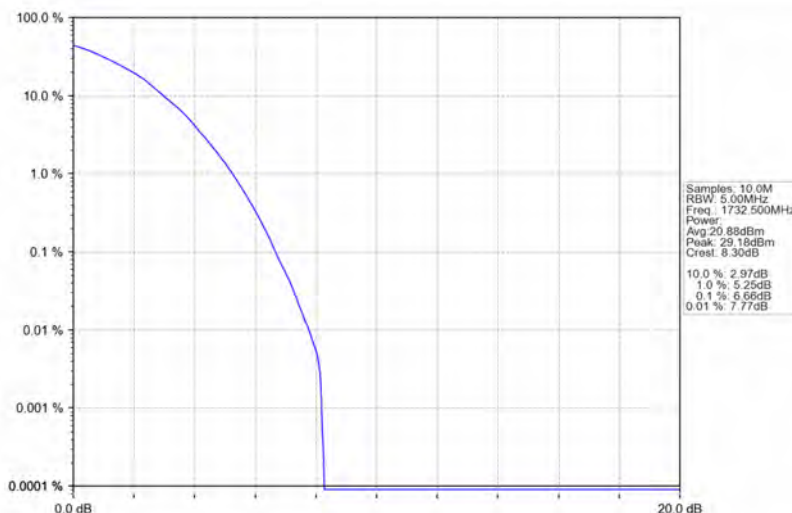
Band4_5MHz_64QAM_MCH_1732.5MHz_RB_25_0_NTNV
