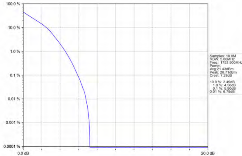
Band4_3MHz_QPSK_HCH_1753.5MHz_RB_15_0_NTNV
