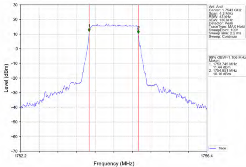
Band4_1.4MHz_16QAM_HCH_1754.3MHz_RB_6_0_NTNV
