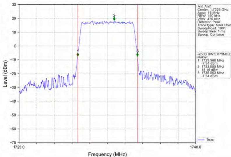
Band4_5MHz_QPSK_MCH_1732.5MHz_RB_25_0_NTNV
