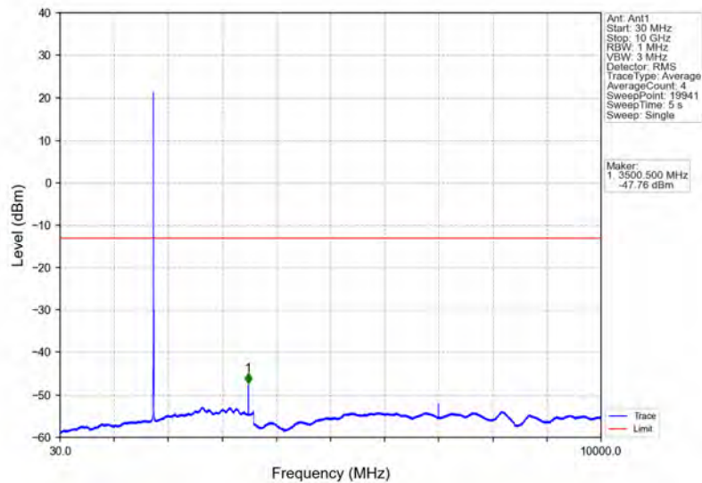
Band4_5MHz_16QAM_HCH_1752.5MHz_RB_1_0_NTNV
