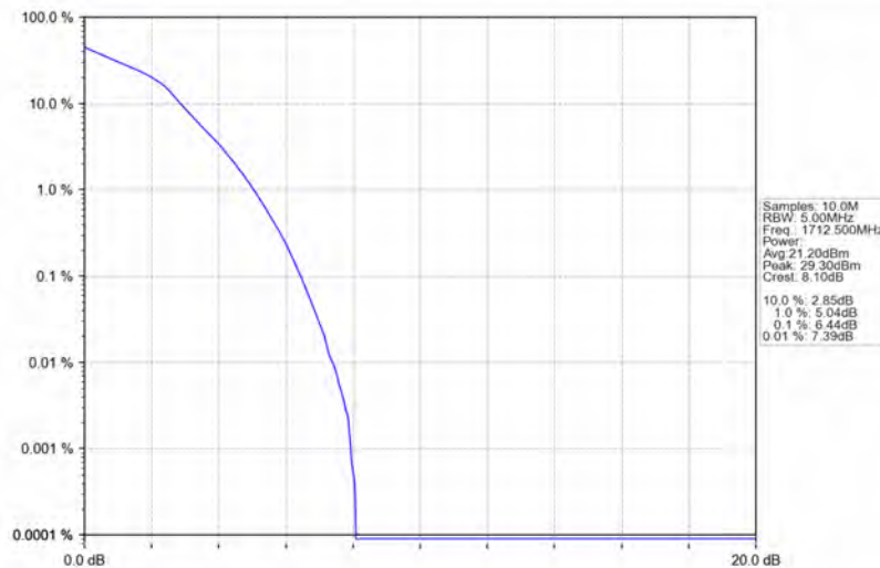
Band4_5MHz_16QAM_LCH_1712.5MHz_RB_25_0_NTNV
