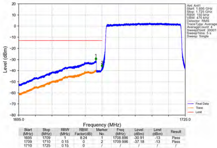
Band4_15MHz_64QAM_LCH_1717.5MHz_RB_75_0_NTNV
