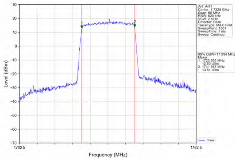
Band4_20MHz_16QAM_MCH_1732.5MHz_RB_100_0_NTNV
