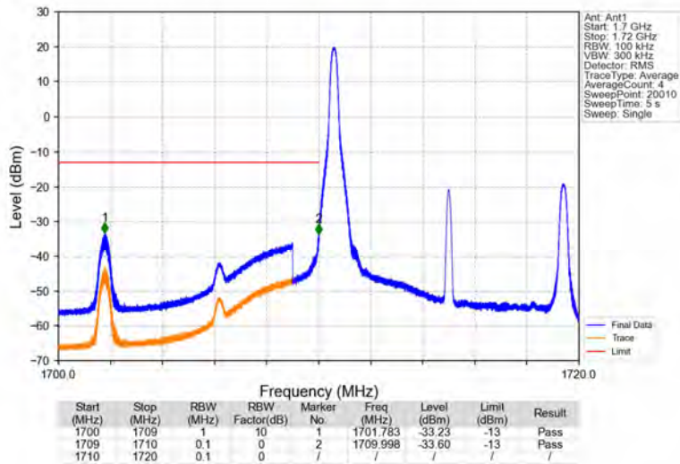
Band4_10MHz_16QAM_LCH_1715MHz_RB_1_0_NTNV
