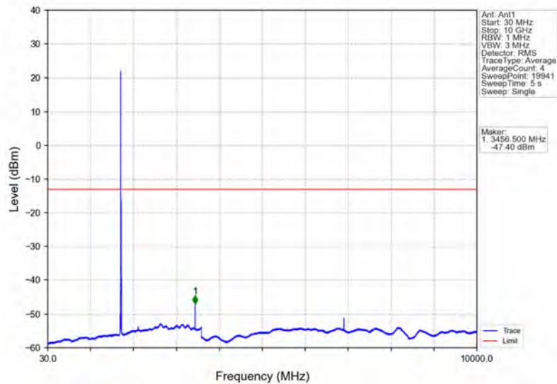
Band4_10MHz_64QAM_MCH_1732.5MHz_RB_1_0_NTNV
