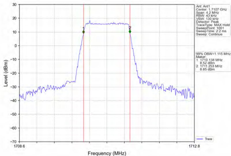
Band4_1.4MHz_16QAM_LCH_1710.7MHz_RB_6_0_NTNV
