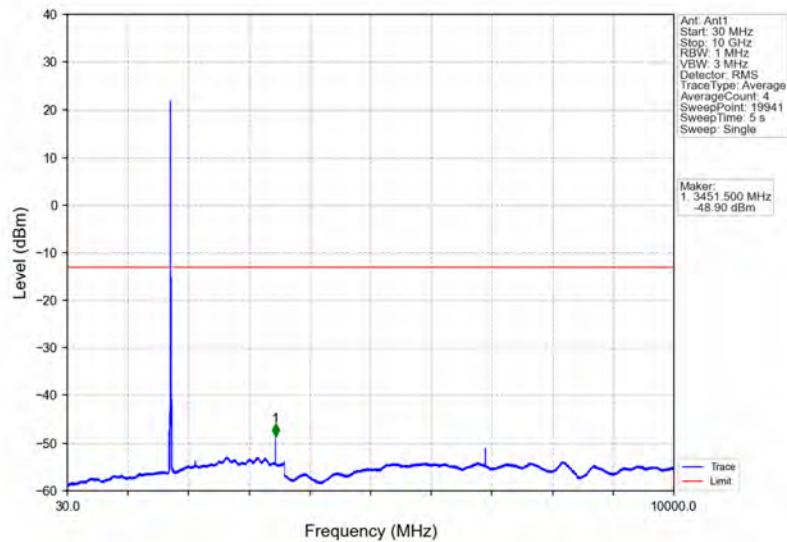
Band4_15MHz_16QAM_MCH_1732.5MHz_RB_1_0_NTNV
