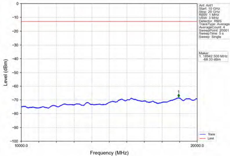
Band4_3MHz_16QAM_LCH_1711.5MHz_RB_15_0_NTNV
