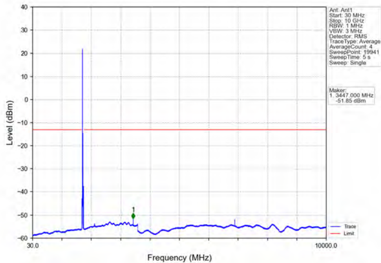
Band4_20MHz_16QAM_MCH_1732.5MHz_RB_1_0_NTNV
