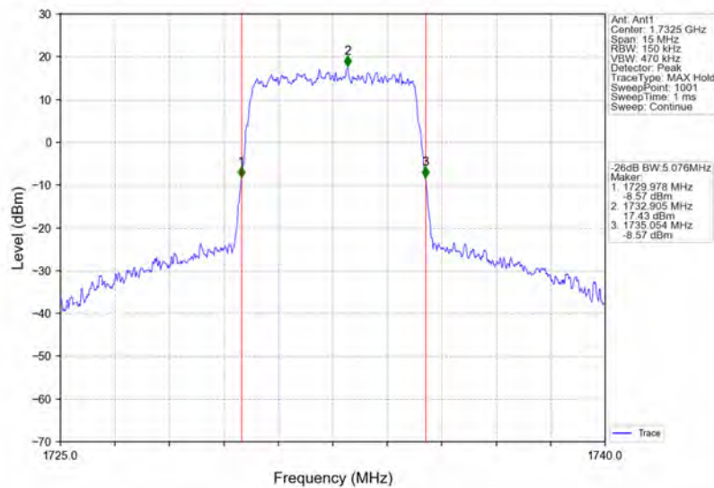
Band4_5MHz_64QAM_MCH_1732.5MHz_RB_25_0_NTNV
