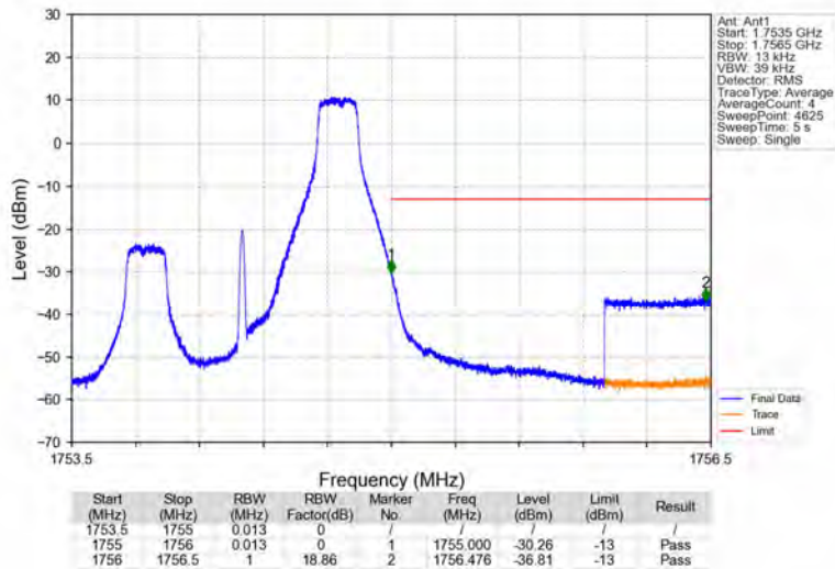
Band4_1.4MHz_64QAM_HCH_1754.3MHz_RB_1_5_NTNV
