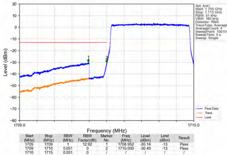
Band4_5MHz_16QAM_LCH_1712.5MHz_RB_25_0_NTNV
