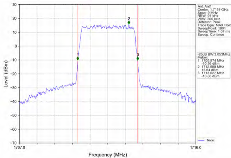
Band4_3MHz_64QAM_LCH_1711.5MHz_RB_15_0_NTNV
