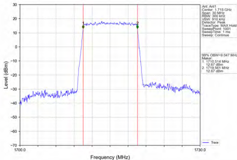
Band4_10MHz_QPSK_LCH_1715MHz_RB_50_0_NTNV
