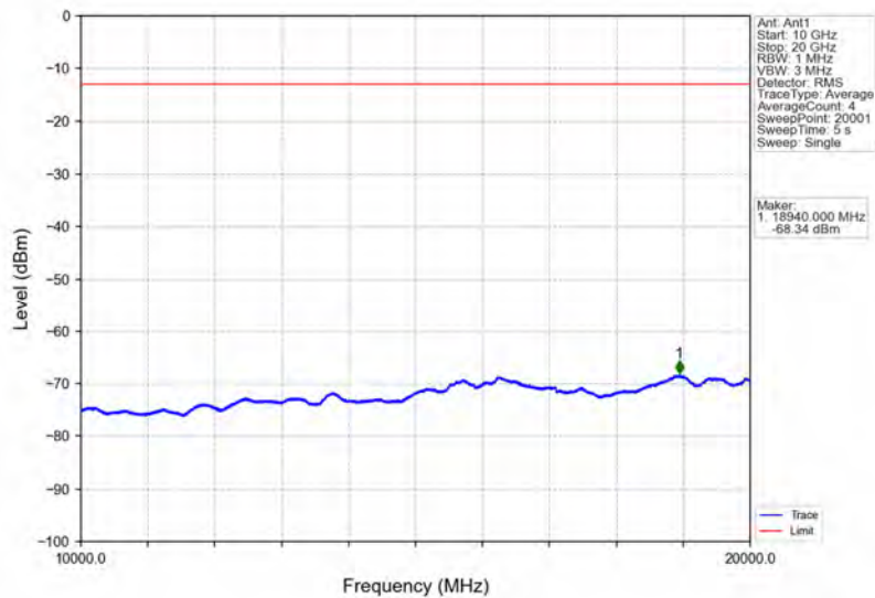
Band4_15MHz_64QAM_LCH_1717.5MHz_RB_75_0_NTNV
