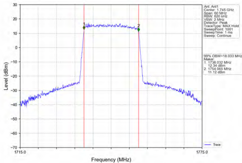
Band4_20MHz_64QAM_HCH_1745MHz_RB_100_0_NTNV
