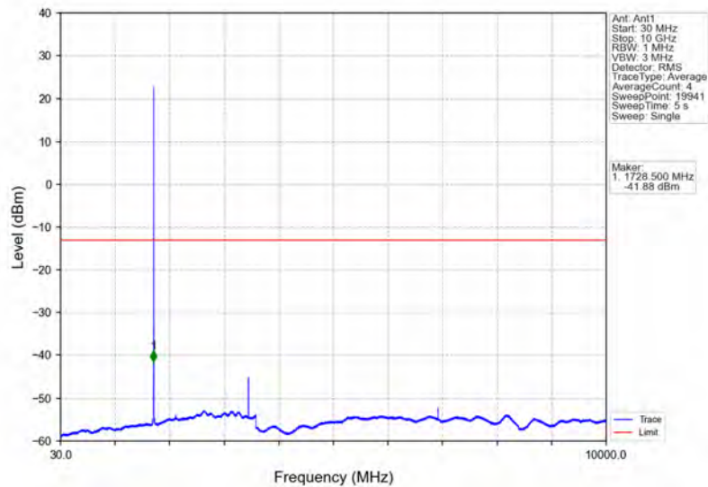
Band4_1.4MHz_16QAM_MCH_1732.5MHz_RB_1_0_NTNV
