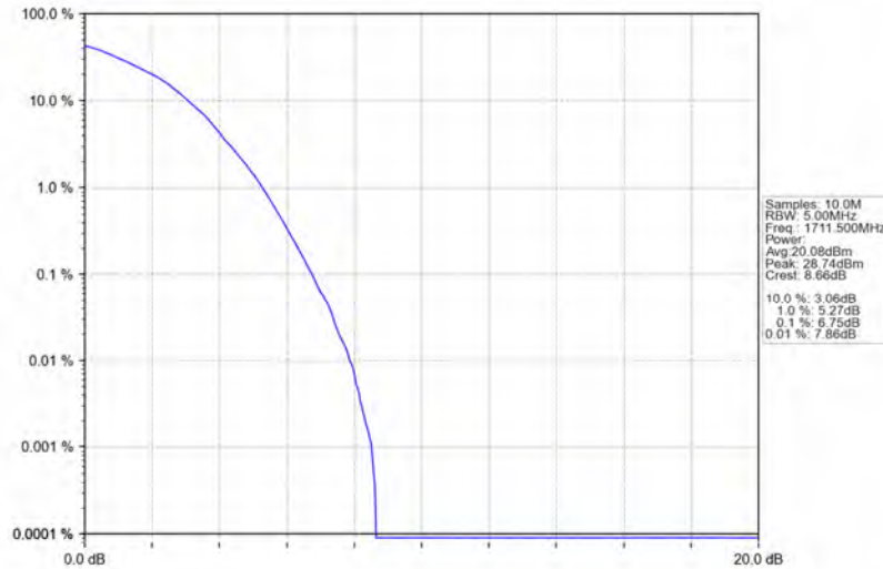
Band4_3MHz_64QAM_LCH_1711.5MHz_RB_15_0_NTNV
