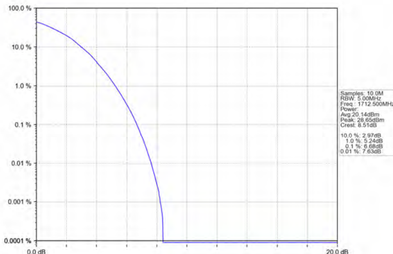
Band4_5MHz_64QAM_LCH_1712.5MHz_RB_25_0_NTNV
