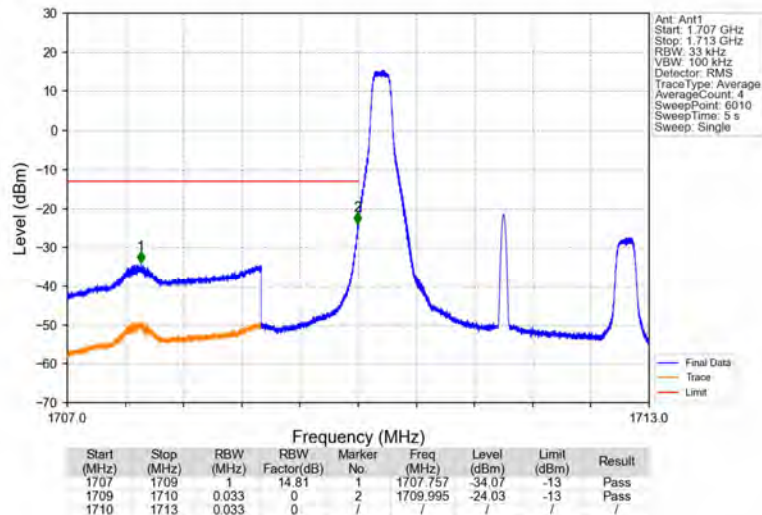
Band4_3MHz_64QAM_LCH_1711.5MHz_RB_1_0_NTNV
