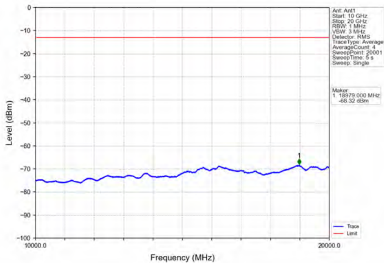
Band4_5MHz_QPSK_MCH_1732.5MHz_RB_1_0_NTNV
