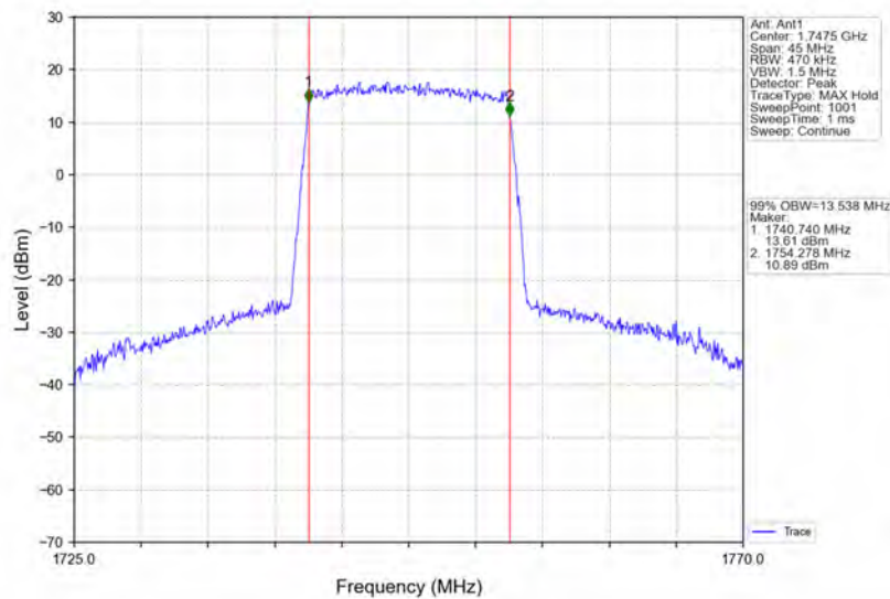
Band4_15MHz_16QAM_HCH_1747.5MHz_RB_75_0_NTNV
