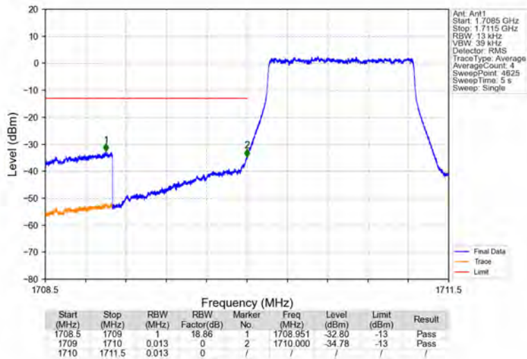
Band4_1.4MHz_64QAM_LCH_1710.7MHz_RB_6_0_NTNV
