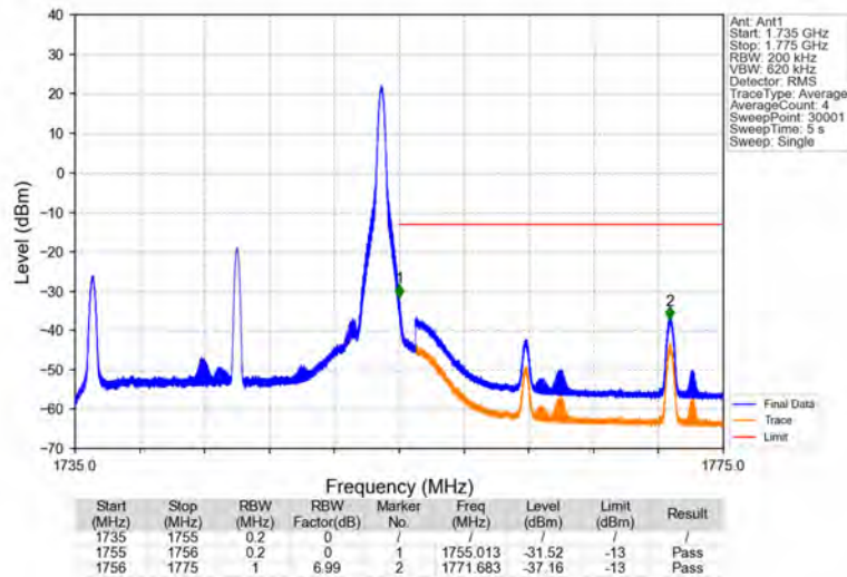
Band4_20MHz_16QAM_HCH_1745MHz_RB_1_99_NTNV
