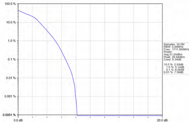
Band4_3MHz_16QAM_LCH_1711.5MHz_RB_15_0_NTNV
