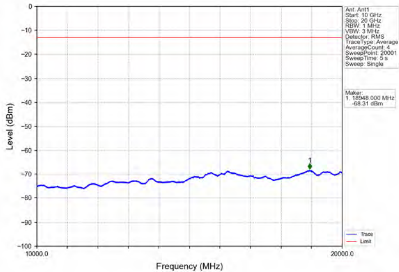
Band4_15MHz_16QAM_LCH_1717.5MHz_RB_75_0_NTNV
