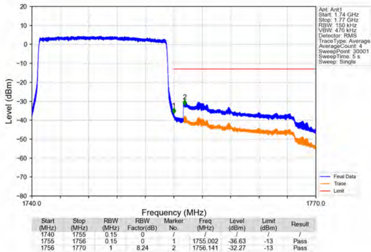
Band4_15MHz_QPSK_HCH_1747.5MHz_RB_75_0_NTNV
