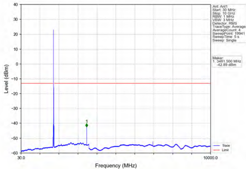
Band4_15MHz_QPSK_HCH_1747.5MHz_RB_1_0_NTNV
