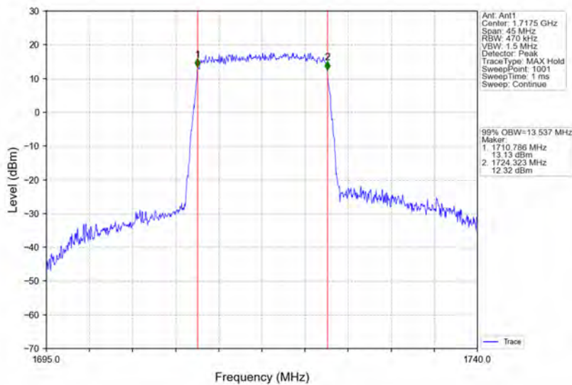
Band4_15MHz_16QAM_LCH_1717.5MHz_RB_75_0_NTNV
