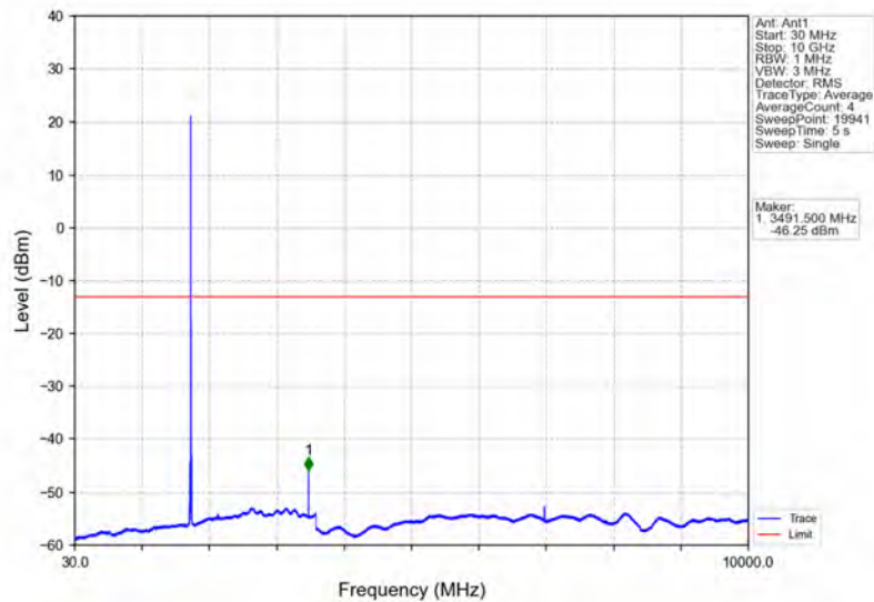
Band4_10MHz_64QAM_HCH_1750MHz_RB_1_0_NTNV
