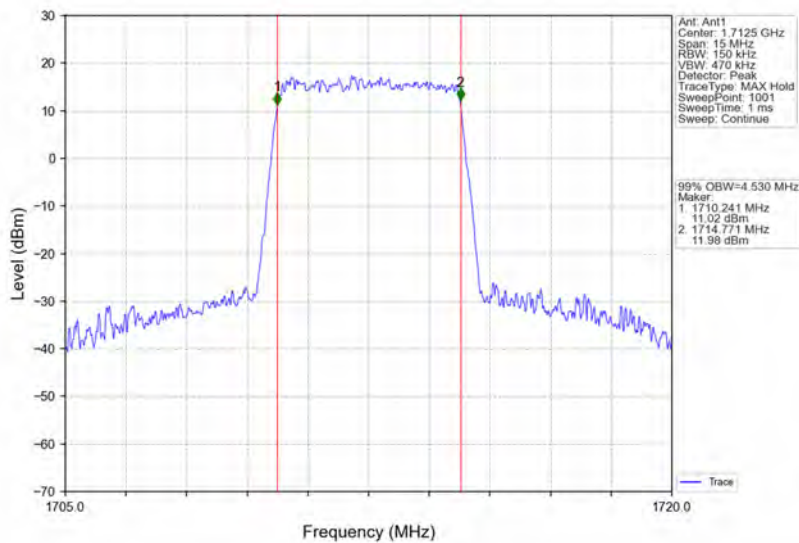
Band4_5MHz_16QAM_LCH_1712.5MHz_RB_25_0_NTNV
