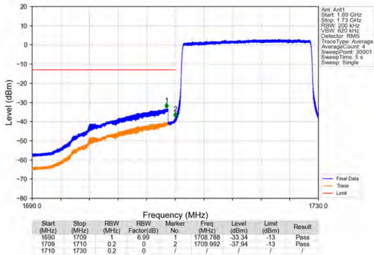
Band4_20MHz_64QAM_LCH_1720MHz_RB_100_0_NTNV
