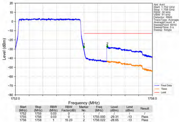
Band4_3MHz_QPSK_HCH_1753.5MHz_RB_15_0_NTNV
