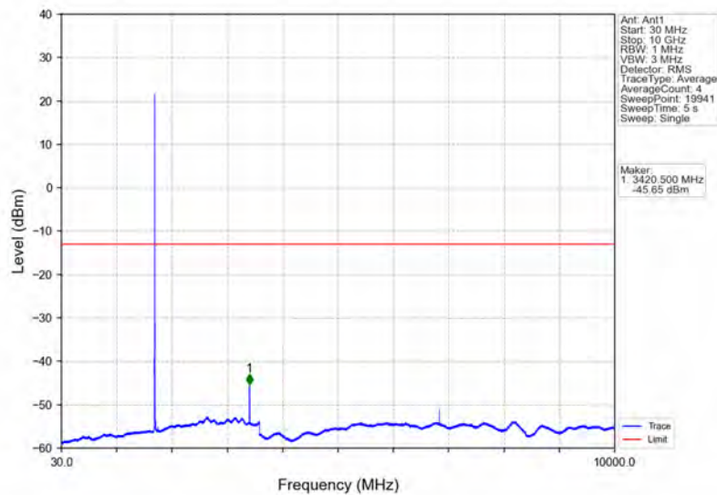
Band4_3MHz_16QAM_LCH_1711.5MHz_RB_1_0_NTNV
