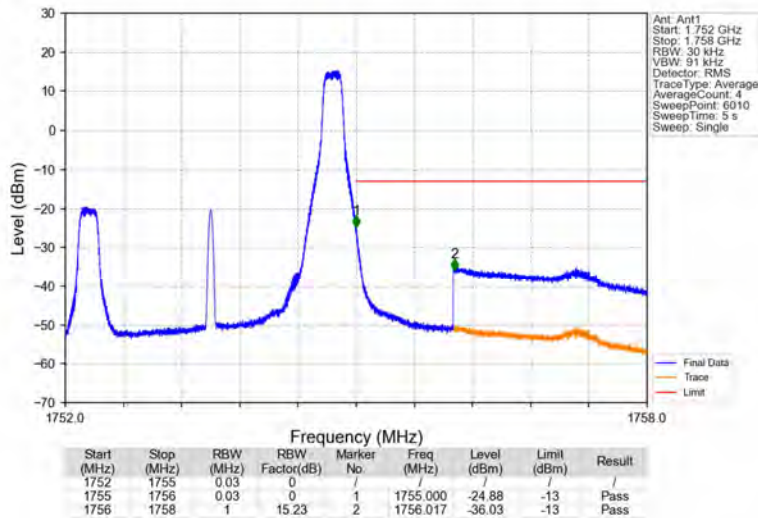
Band4_3MHz_16QAM_HCH_1753.5MHz_RB_1_14_NTNV
