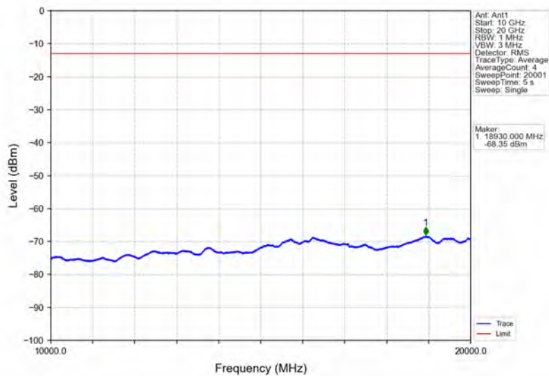
Band4_15MHz_16QAM_HCH_1747.5MHz_RB_1_0_NTNV
