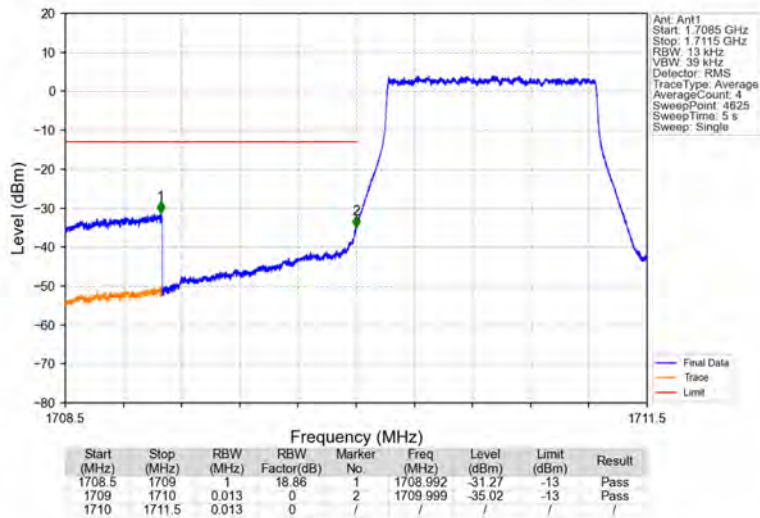
Band4_1.4MHz_16QAM_LCH_1710.7MHz_RB_6_0_NTNV
