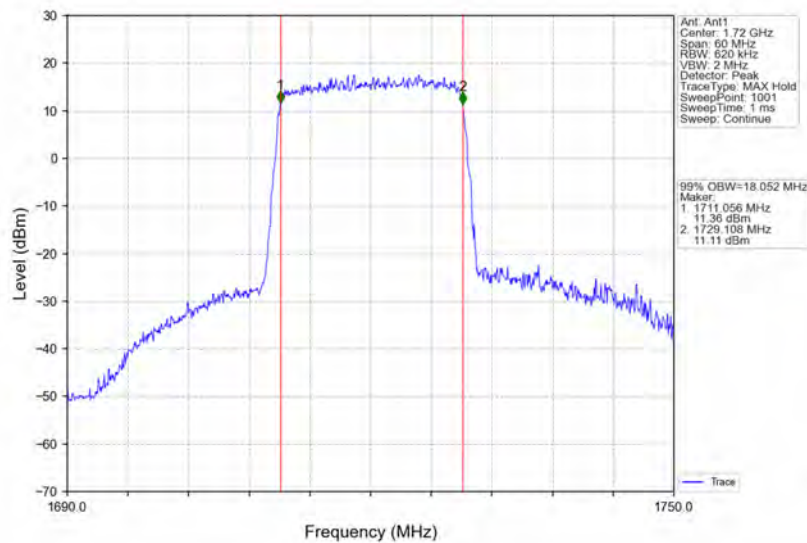
Band4_20MHz_64QAM_LCH_1720MHz_RB_100_0_NTNV
