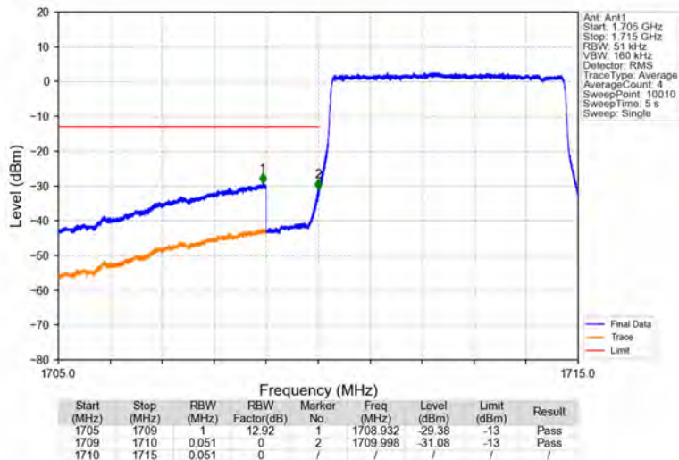
Band4_5MHz_64QAM_LCH_1712.5MHz_RB_25_0_NTNV
