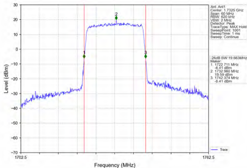
Band4_20MHz_16QAM_MCH_1732.5MHz_RB_100_0_NTNV
