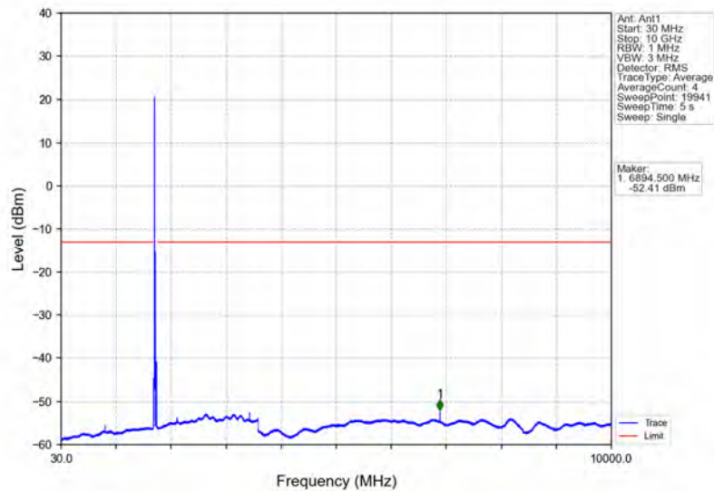
Band4_20MHz_64QAM_MCH_1732.5MHz_RB_1_0_NTNV
