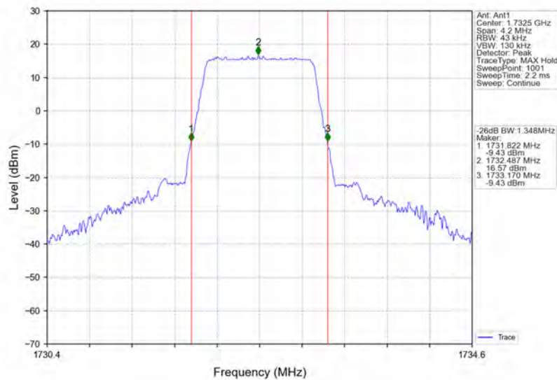
Band4_1.4MHz_64QAM_MCH_1732.5MHz_RB_6_0_NTNV
