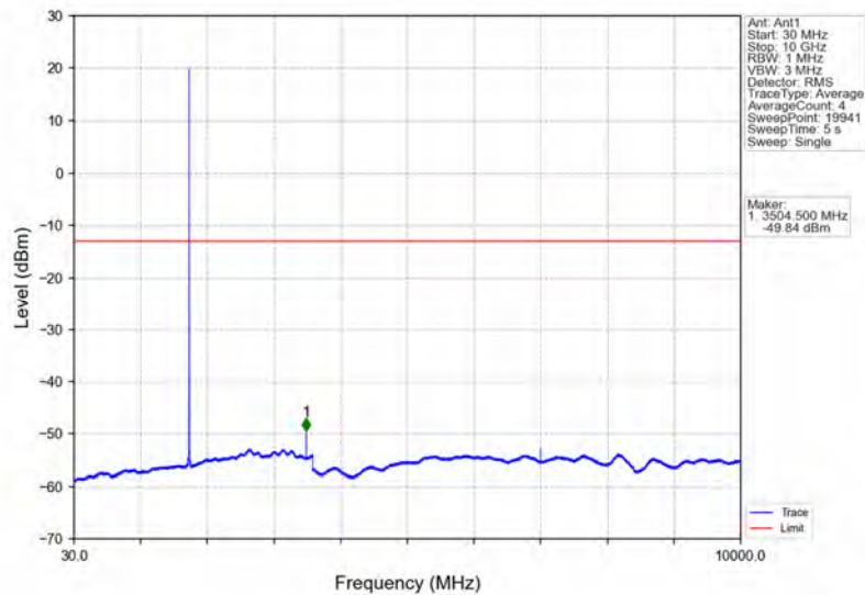
Band4_3MHz_64QAM_HCH_1753.5MHz_RB_1_0_NTNV
