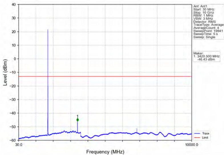
Band4_5MHz_16QAM_LCH_1712.5MHz_RB_1_0_NTNV
