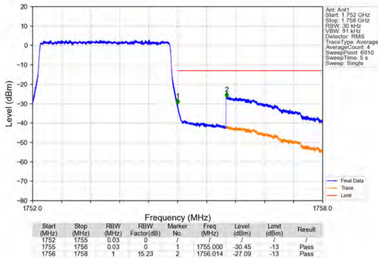
Band4_3MHz_16QAM_HCH_1753.5MHz_RB_15_0_NTNV
