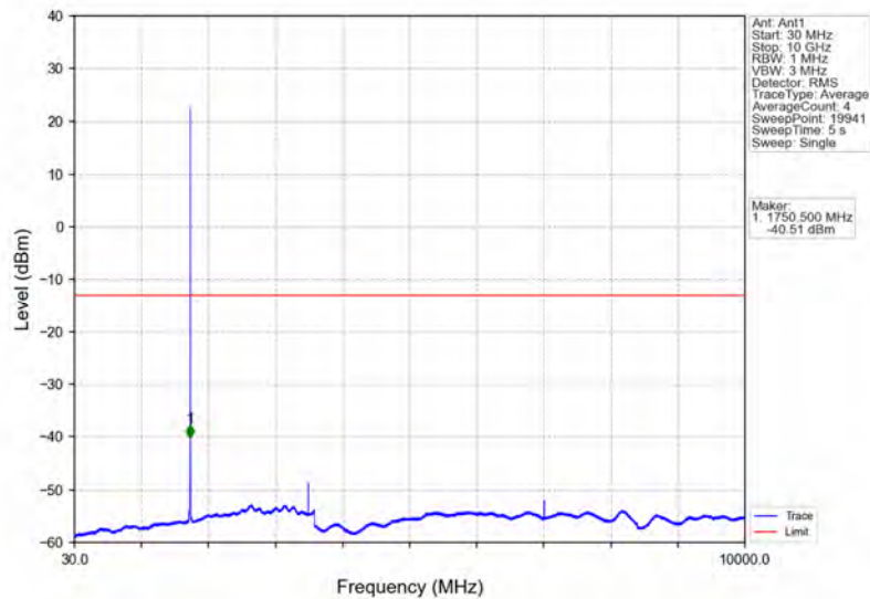
Band4_1.4MHz_QPSK_HCH_1754.3MHz_RB_1_0_NTNV
