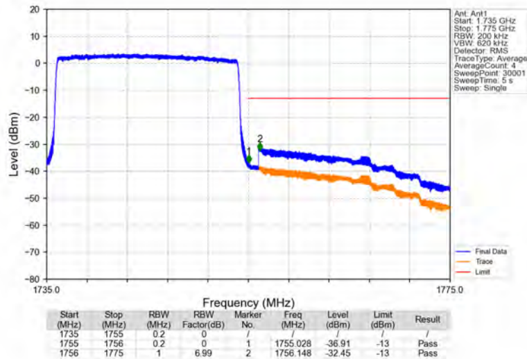
Band4_20MHz_16QAM_HCH_1745MHz_RB_100_0_NTNV
