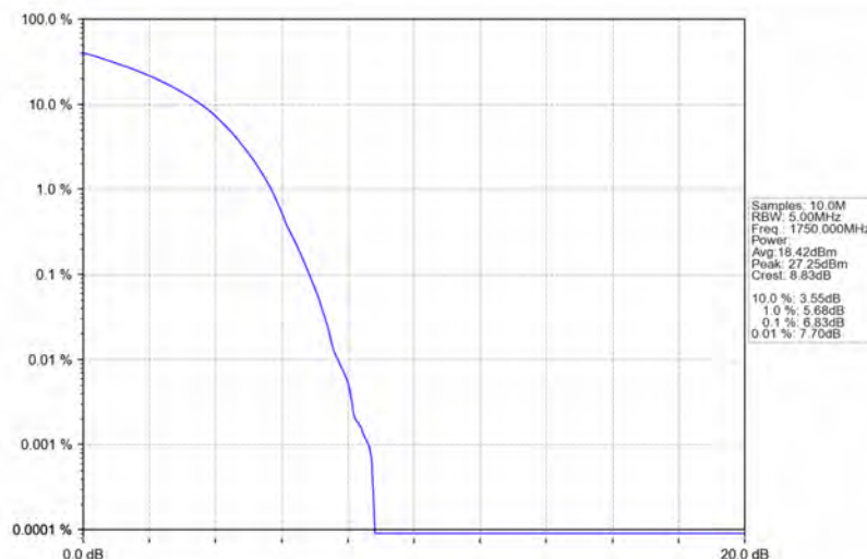
Band4_10MHz_16QAM_HCH_1750MHz_RB_50_0_NTNV
