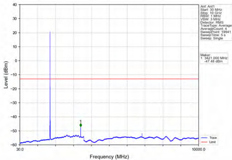
Band4_10MHz_64QAM_LCH_1715MHz_RB_1_0_NTNV
