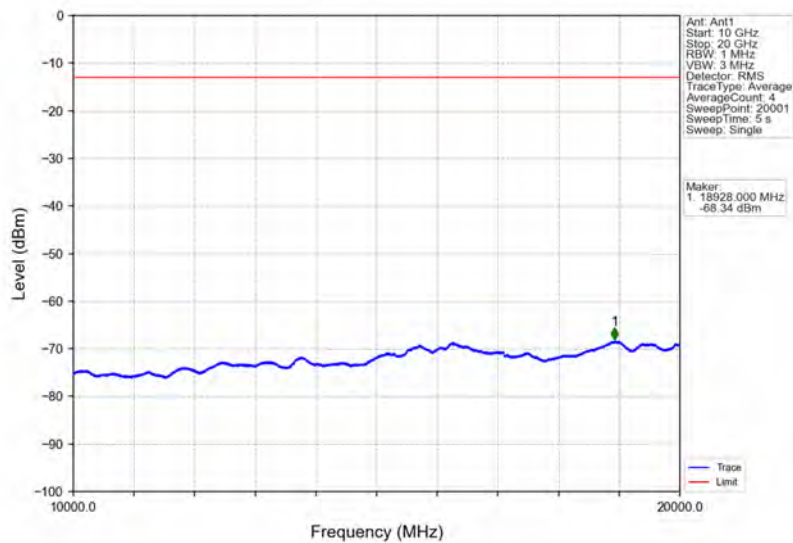
Band4_20MHz_16QAM_MCH_1732.5MHz_RB_1_0_NTNV
