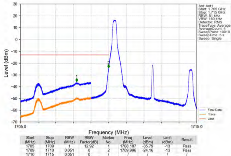
Band4_5MHz_64QAM_LCH_1712.5MHz_RB_1_0_NTNV
