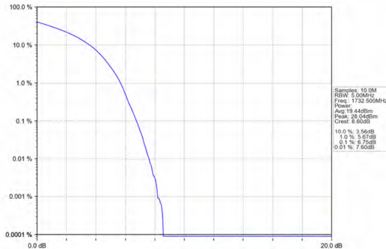
Band4_10MHz_16QAM_MCH_1732.5MHz_RB_50_0_NTNV
