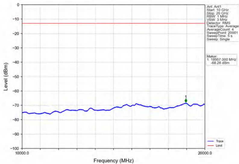
Band4_3MHz_QPSK_HCH_1753.5MHz_RB_1_0_NTNV
