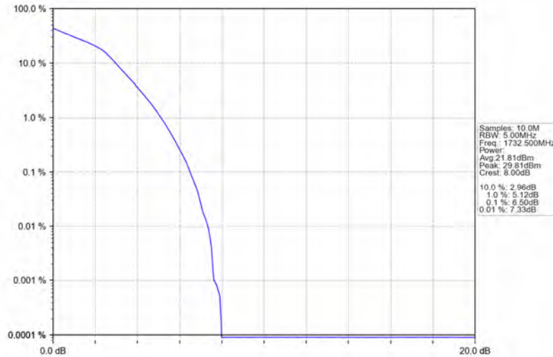
Band4_3MHz_16QAM_MCH_1732.5MHz_RB_15_0_NTNV
