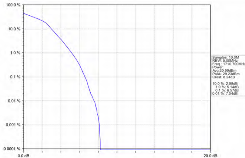
Band4_1.4MHz_16QAM_LCH_1710.7MHz_RB_6_0_NTNV
