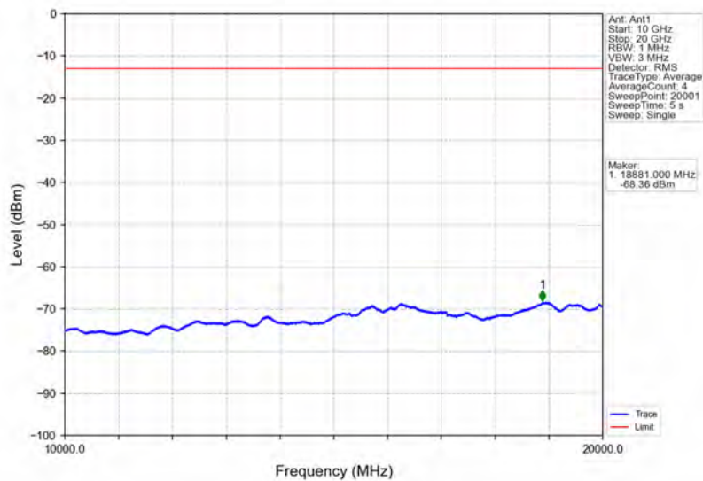
Band4_5MHz_64QAM_MCH_1732.5MHz_RB_1_0_NTNV
