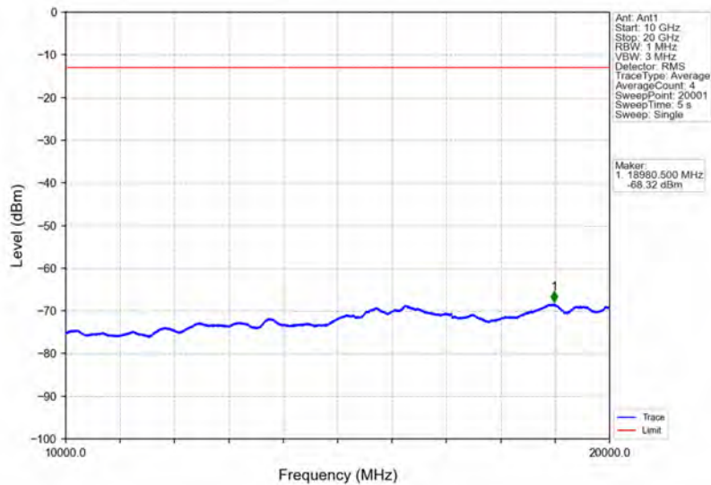
Band4_20MHz_64QAM_HCH_1745MHz_RB_1_0_NTNV
