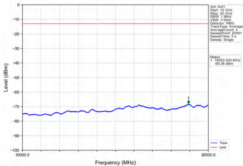
Band4_5MHz_16QAM_HCH_1752.5MHz_RB_1_0_NTNV
