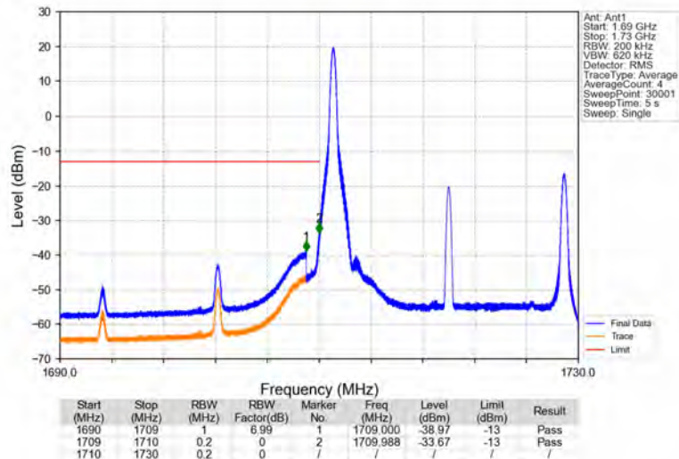
Band4_20MHz_64QAM_LCH_1720MHz_RB_1_0_NTNV
