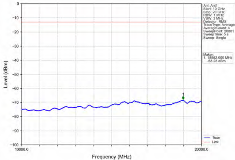
Band4_10MHz_64QAM_LCH_1715MHz_RB_50_0_NTNV
