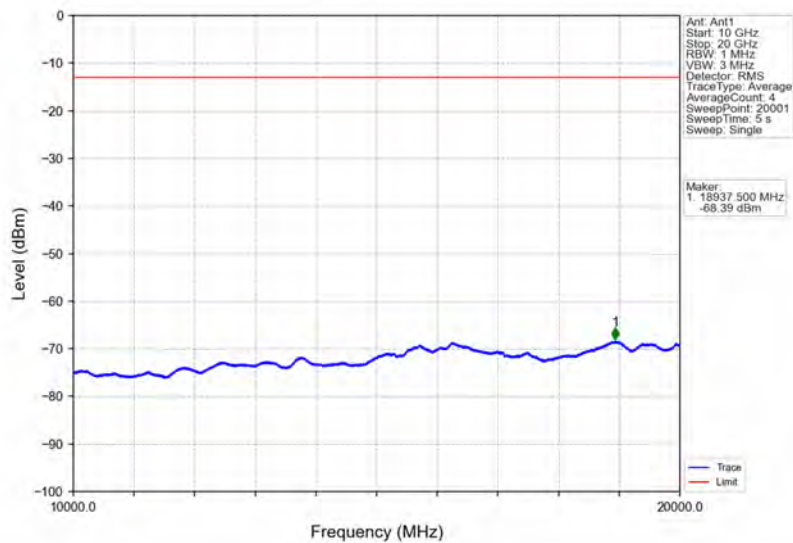
Band4_15MHz_QPSK_HCH_1747.5MHz_RB_1_0_NTNV
