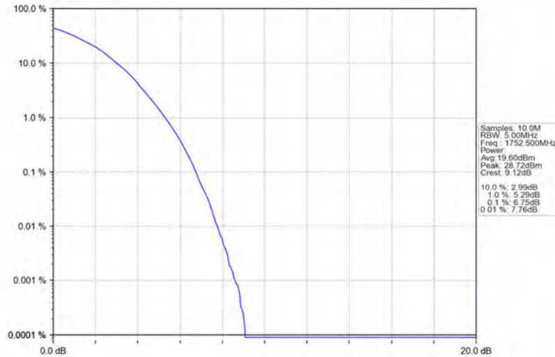
Band4_5MHz_64QAM_HCH_1752.5MHz_RB_25_0_NTNV
