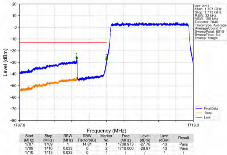
Band4_3MHz_16QAM_LCH_1711.5MHz_RB_15_0_NTNV
