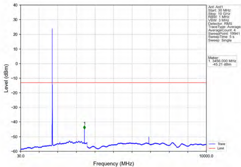
Band4_10MHz_QPSK_MCH_1732.5MHz_RB_1_0_NTNV
