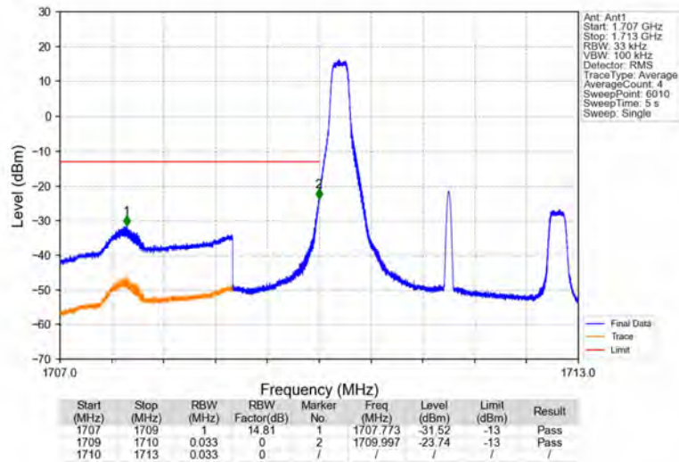
Band4_3MHz_16QAM_LCH_1711.5MHz_RB_1_0_NTNV
