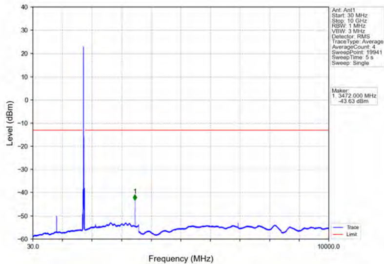
Band4_20MHz_16QAM_HCH_1745MHz_RB_1_0_NTNV
