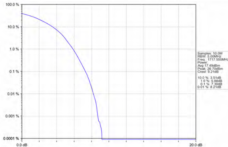
Band4_15MHz_16QAM_LCH_1717.5MHz_RB_75_0_NTNV
