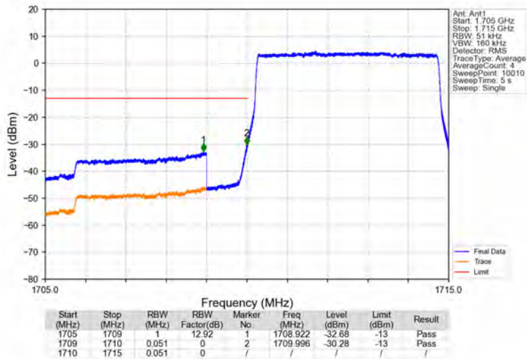
Band4_5MHz_QPSK_LCH_1712.5MHz_RB_25_0_NTNV
