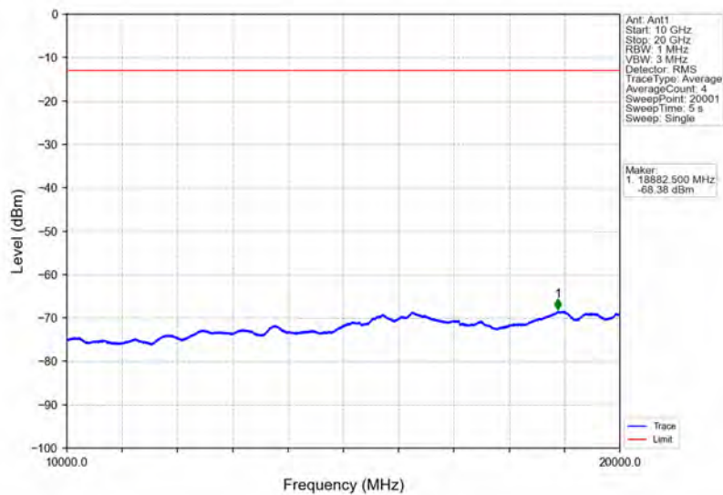
Band4_15MHz_64QAM_HCH_1747.5MHz_RB_1_0_NTNV
