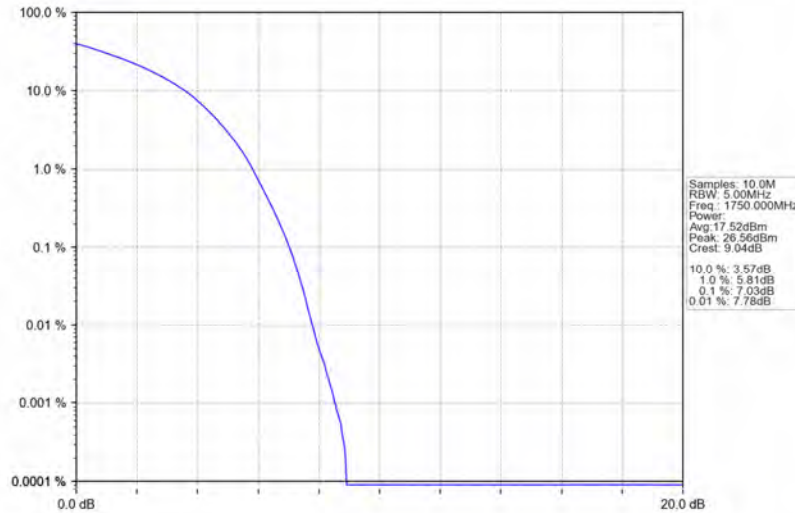
Band4_10MHz_64QAM_HCH_1750MHz_RB_50_0_NTNV
