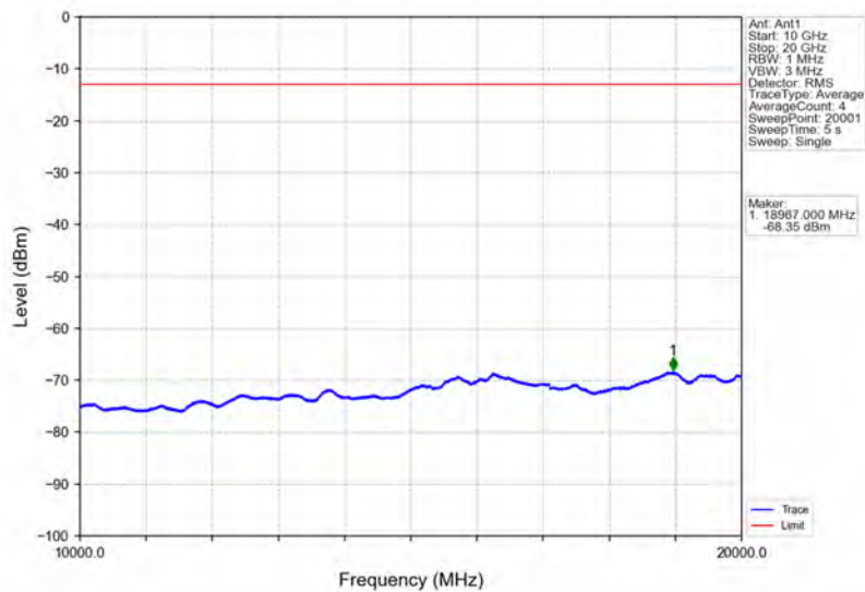
Band4_3MHz_64QAM_MCH_1732.5MHz_RB_1_0_NTNV
