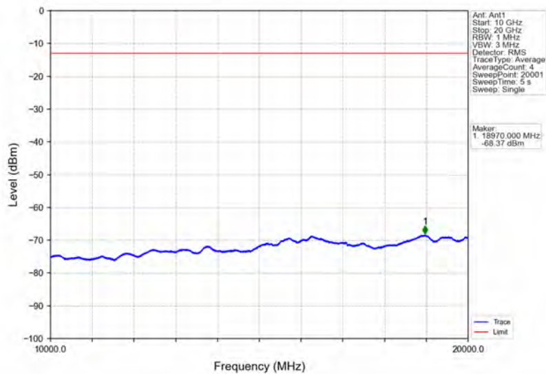
Band4_1.4MHz_QPSK_HCH_1754.3MHz_RB_1_0_NTNV
