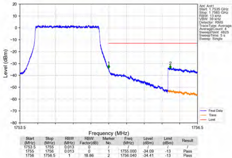
Band4_1.4MHz_64QAM_HCH_1754.3MHz_RB_6_0_NTNV
