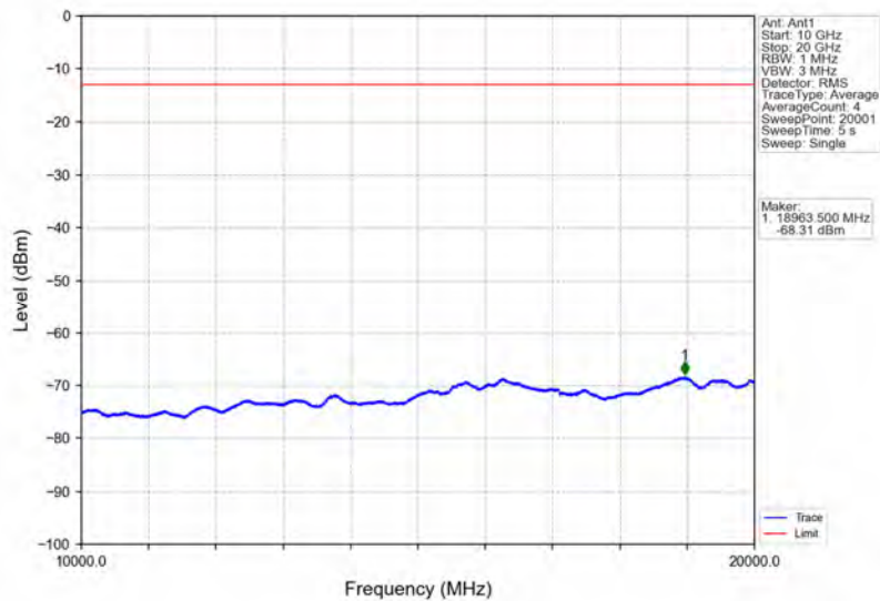
Band4_20MHz_64QAM_LCH_1720MHz_RB_100_0_NTNV
