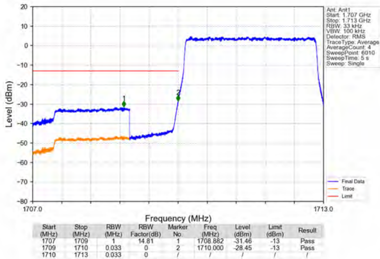
Band4_3MHz_QPSK_LCH_1711.5MHz_RB_15_0_NTNV
