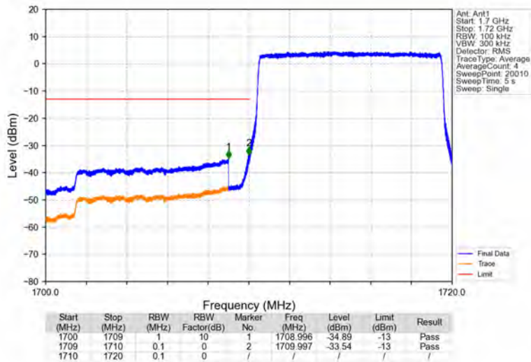
Band4_10MHz_QPSK_LCH_1715MHz_RB_50_0_NTNV
