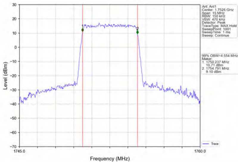
Band4_5MHz_16QAM_HCH_1752.5MHz_RB_25_0_NTNV
