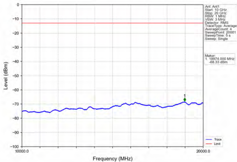
Band4_20MHz_16QAM_HCH_1745MHz_RB_1_0_NTNV
