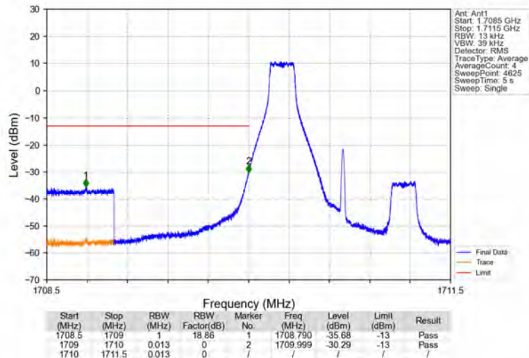
Band4_1.4MHz_64QAM_LCH_1710.7MHz_RB_1_0_NTNV
