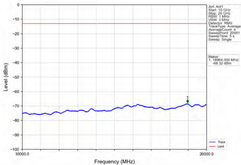
Band4_3MHz_64QAM_HCH_1753.5MHz_RB_1_0_NTNV
