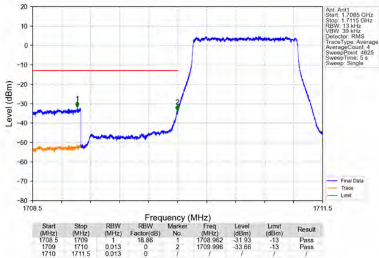
Band4_1.4MHz_QPSK_LCH_1710.7MHz_RB_6_0_NTNV
