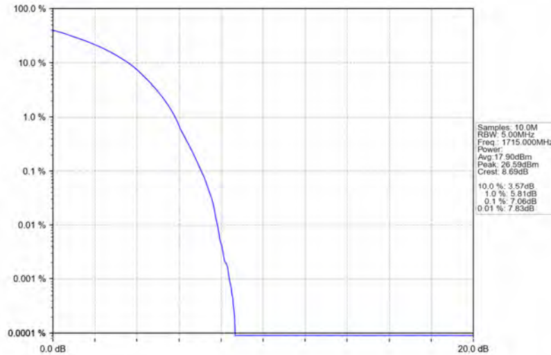
Band4_10MHz_64QAM_LCH_1715MHz_RB_50_0_NTNV
