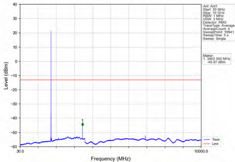
Band4_3MHz_64QAM_MCH_1732.5MHz_RB_1_0_NTNV
