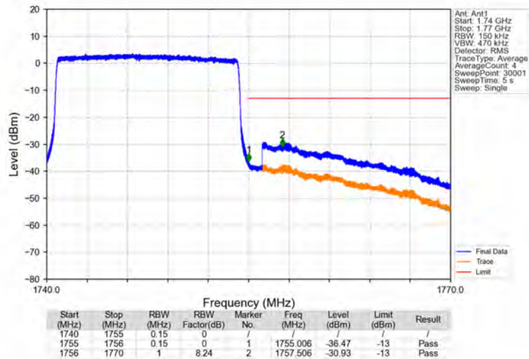
Band4_15MHz_16QAM_HCH_1747.5MHz_RB_75_0_NTNV
