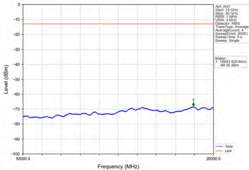
Band4_10MHz_QPSK_LCH_1715MHz_RB_50_0_NTNV
