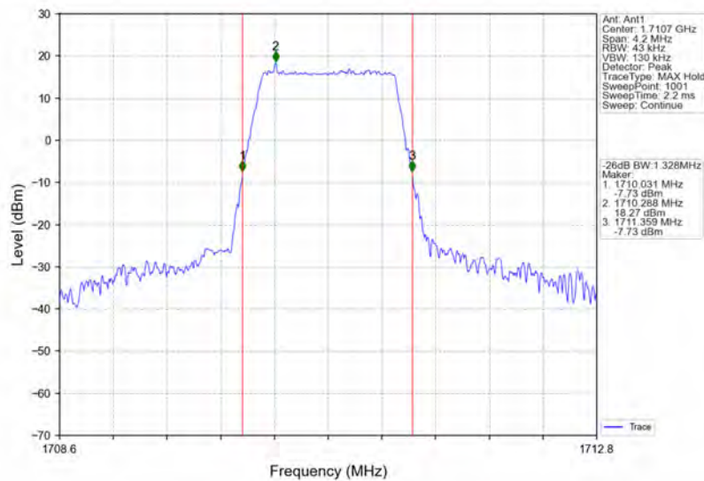
Band4_1.4MHz_16QAM_LCH_1710.7MHz_RB_6_0_NTNV
