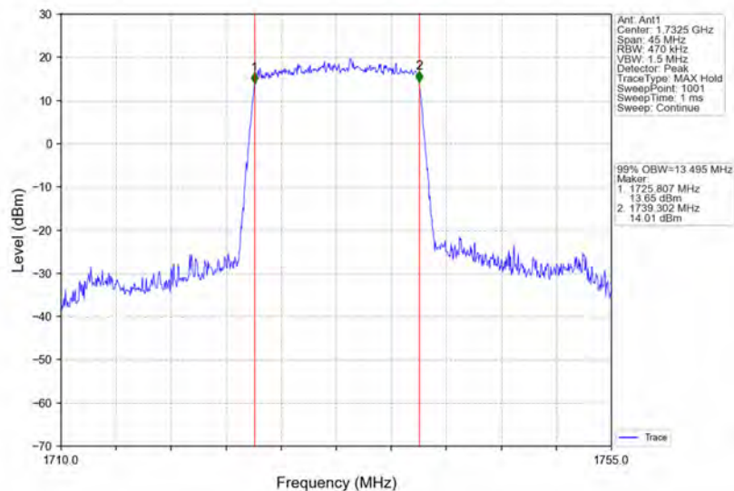
Band4_15MHz_QPSK_MCH_1732.5MHz_RB_75_0_NTNV
