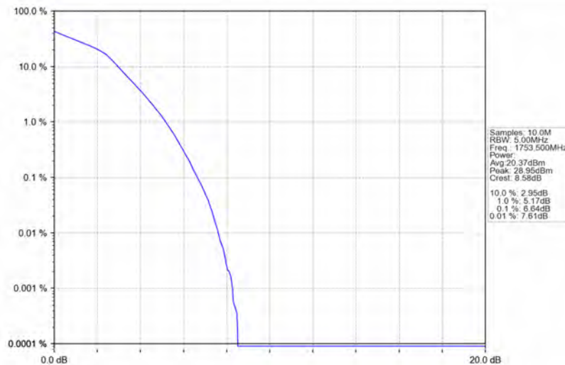
Band4_3MHz_16QAM_HCH_1753.5MHz_RB_15_0_NTNV
