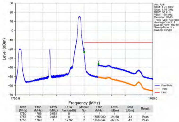
Band4_5MHz_64QAM_HCH_1752.5MHz_RB_1_24_NTNV
