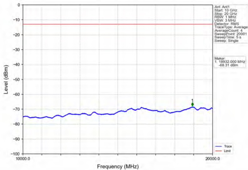
Band4_3MHz_16QAM_HCH_1753.5MHz_RB_1_0_NTNV
