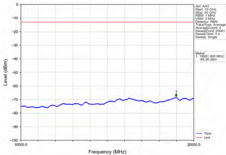
Band4_15MHz_64QAM_MCH_1732.5MHz_RB_1_0_NTNV
