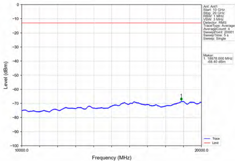
Band4_1.4MHz_64QAM_MCH_1732.5MHz_RB_1_0_NTNV
