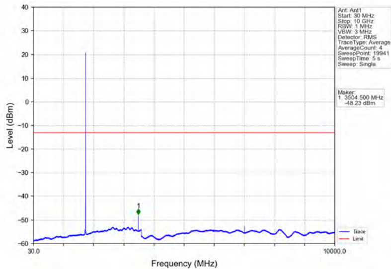
Band4_3MHz_16QAM_HCH_1753.5MHz_RB_1_0_NTNV
