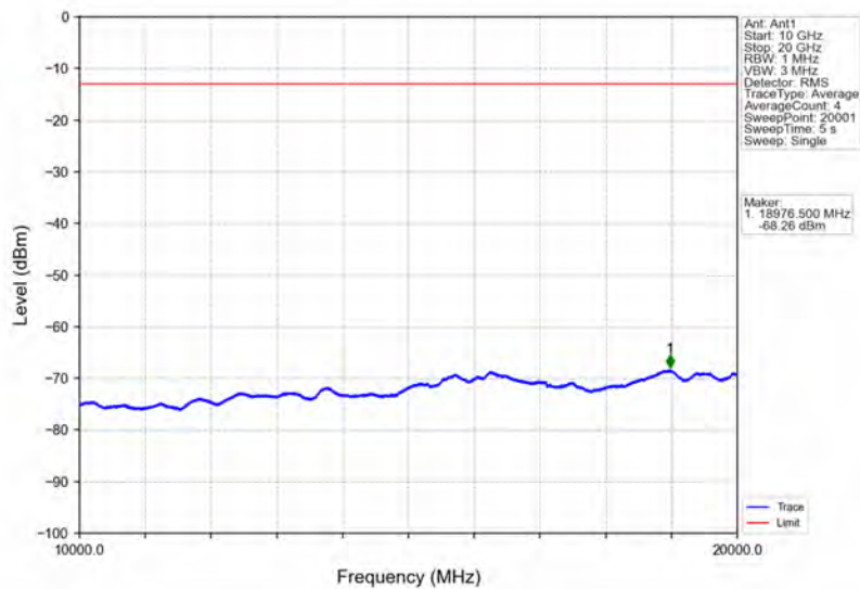
Band4_20MHz_64QAM_MCH_1732.5MHz_RB_1_0_NTNV
