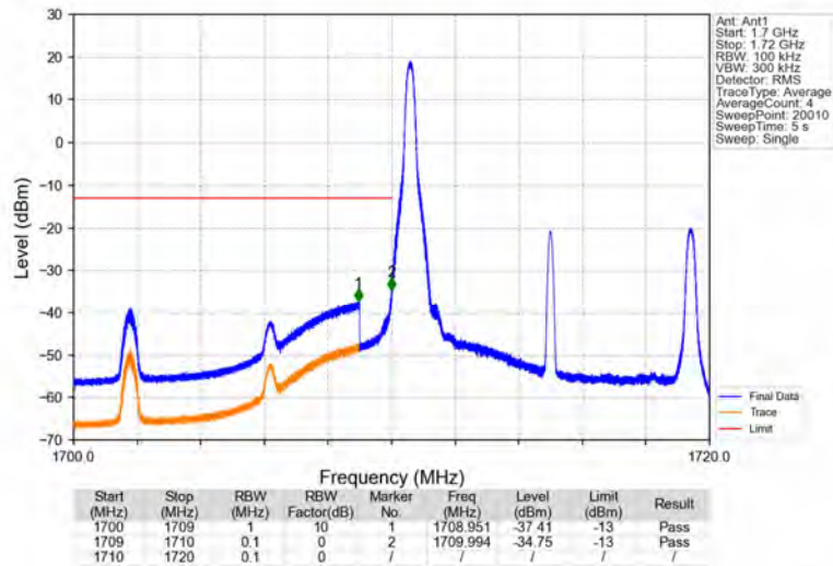
Band4_10MHz_64QAM_LCH_1715MHz_RB_1_0_NTNV
