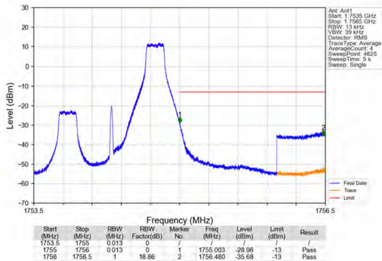
Band4_1.4MHz_16QAM_HCH_1754.3MHz_RB_1_5_NTNV
