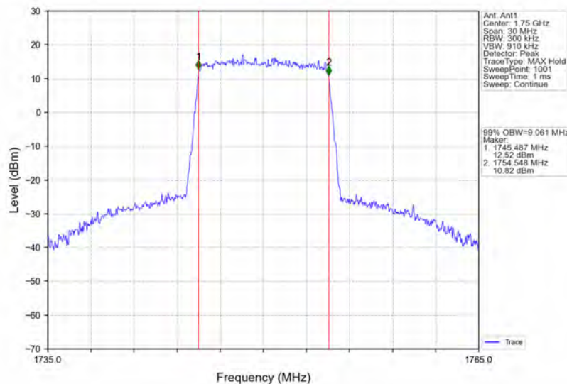
Band4_10MHz_64QAM_HCH_1750MHz_RB_50_0_NTNV
