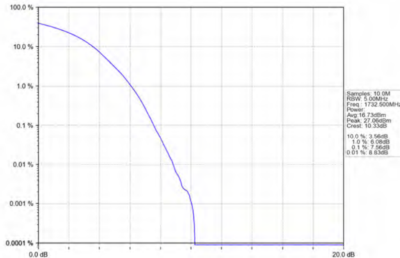
Band4_20MHz_16QAM_MCH_1732.5MHz_RB_100_0_NTNV
