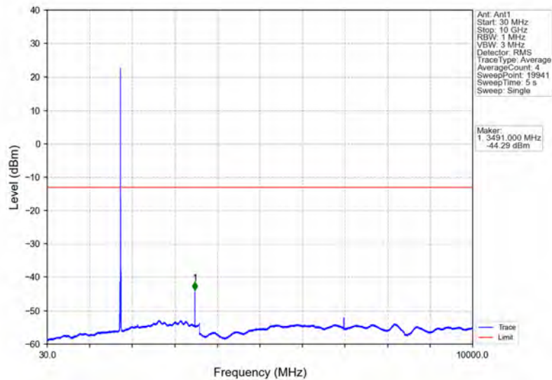
Band4_10MHz_16QAM_HCH_1750MHz_RB_1_0_NTNV
