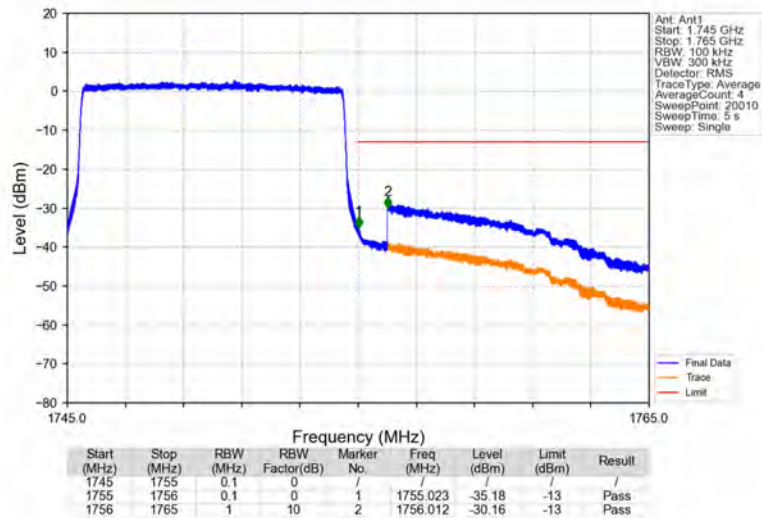
Band4_10MHz_64QAM_HCH_1750MHz_RB_50_0_NTNV
