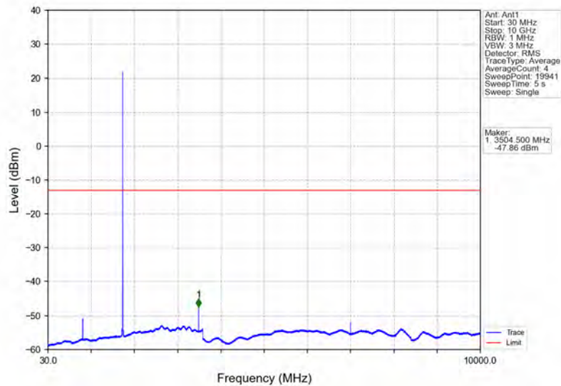
Band4_3MHz_QPSK_HCH_1753.5MHz_RB_1_0_NTNV
