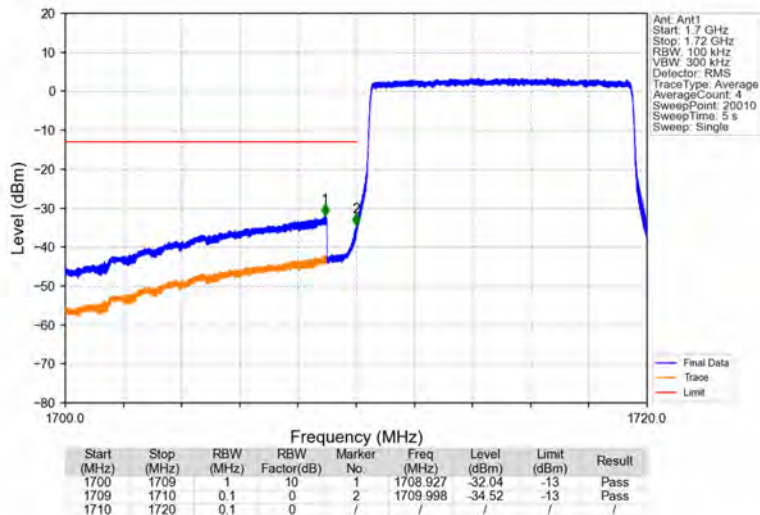
Band4_10MHz_16QAM_LCH_1715MHz_RB_50_0_NTNV
