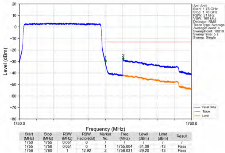
Band4_5MHz_QPSK_HCH_1752.5MHz_RB_25_0_NTNV
