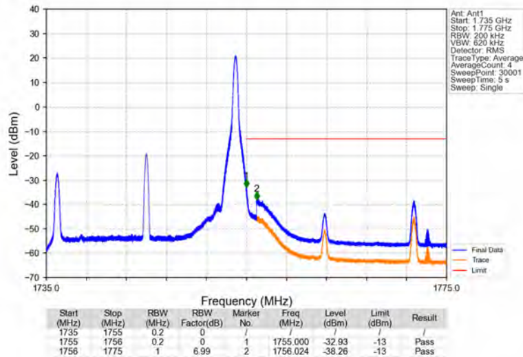
Band4_20MHz_64QAM_HCH_1745MHz_RB_1_99_NTNV
