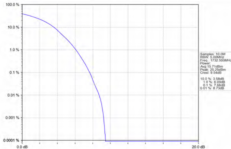
Band4_20MHz_64QAM_MCH_1732.5MHz_RB_100_0_NTNV
