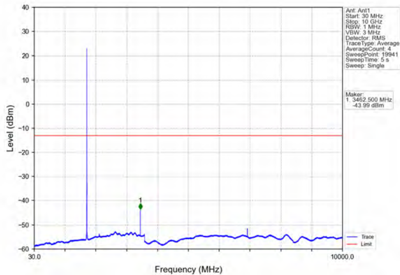
Band4_3MHz_16QAM_MCH_1732.5MHz_RB_1_0_NTNV
