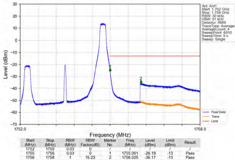
Band4_3MHz_64QAM_HCH_1753.5MHz_RB_1_14_NTNV
