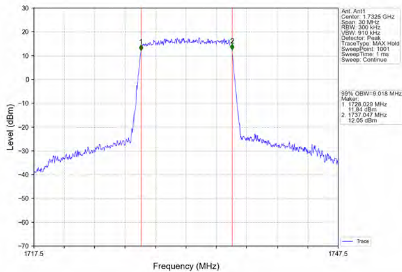
Band4_10MHz_16QAM_MCH_1732.5MHz_RB_50_0_NTNV
