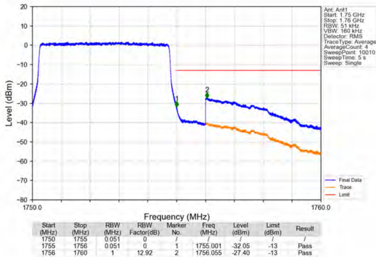
Band4_5MHz_64QAM_HCH_1752.5MHz_RB_25_0_NTNV
