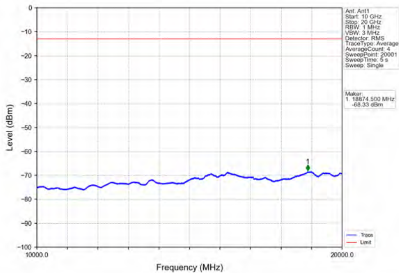
Band4_1.4MHz_16QAM_HCH_1754.3MHz_RB_1_0_NTNV
