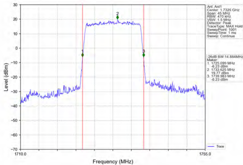
Band4_15MHz_QPSK_MCH_1732.5MHz_RB_75_0_NTNV
