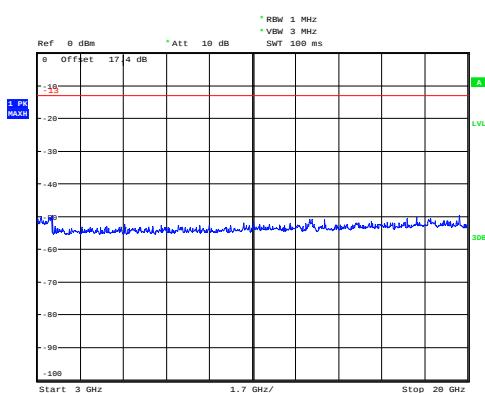
GSM 1900 CH-Low 3GHz~20GHz
