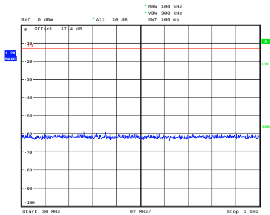
GSM 1900 CH-Low 30MHz~1GHz
