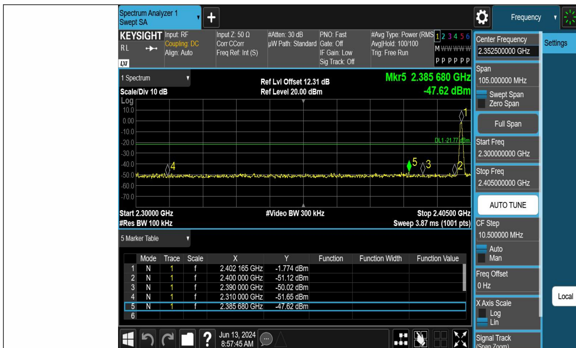
DH5-Ant1-2402-PASS
