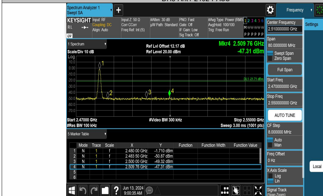
DH5-Ant1-2480-PASS
