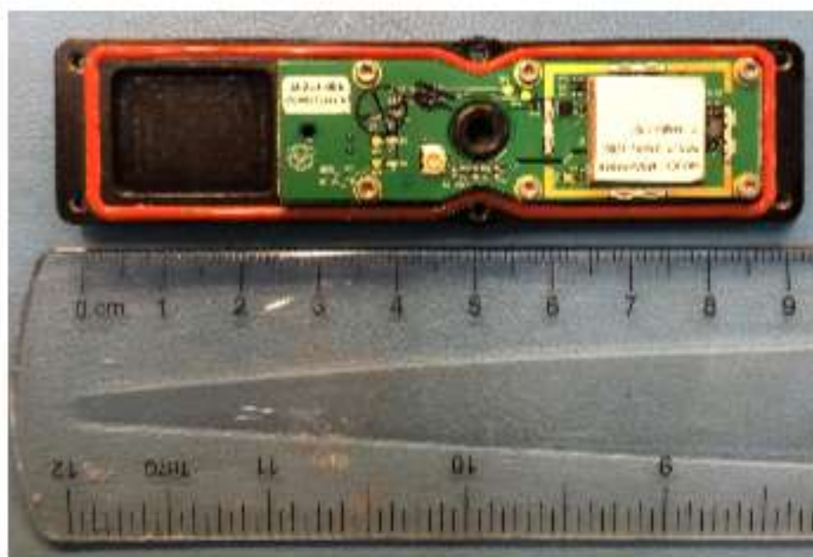
Figure 6: TW-1760 PCB, shield-can removed
