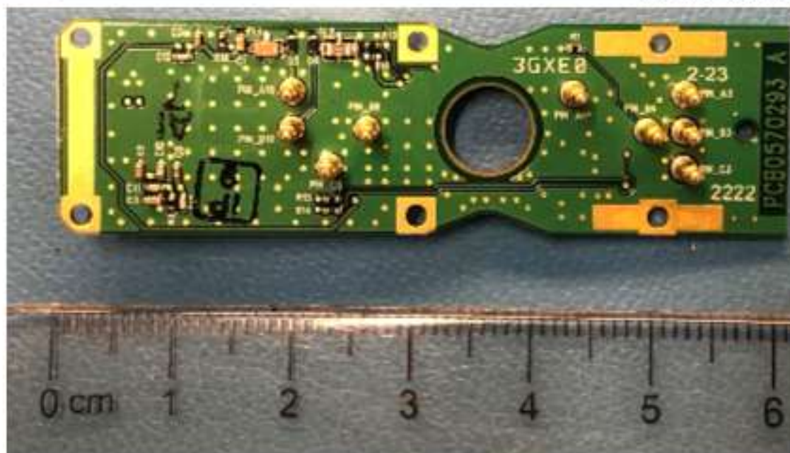
Figure 7: TW-1760 PCB, bottom
