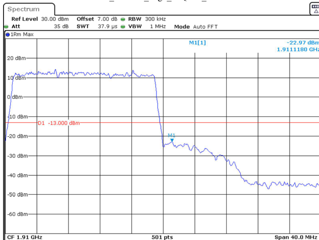
Band 2_20 MHz_High_16QAM_RB100#0
