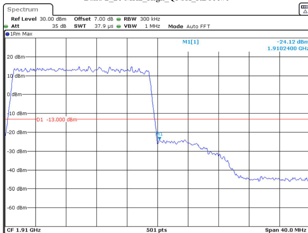
Band 2 20 MHz High QPSK RB100#0
