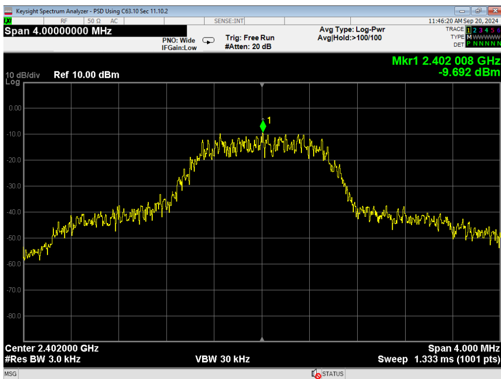
10, PSD, 2EDR, Low
