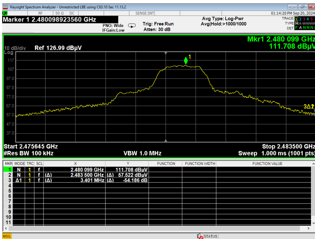
30, HBE Unrestricted, 3EDR
