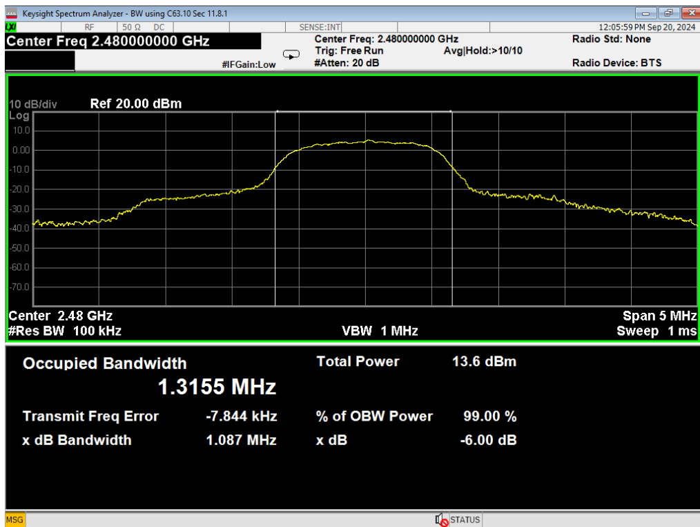
09, 6dB Bandwidth, 2EDR, High
