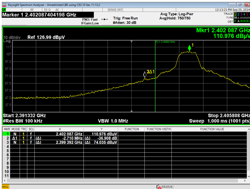
29, LBE Unrestricted, 3EDR
