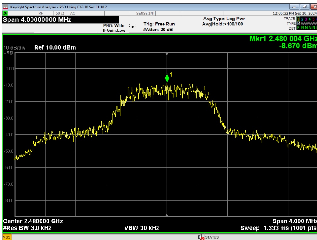
12, PSD, 2EDR, High
