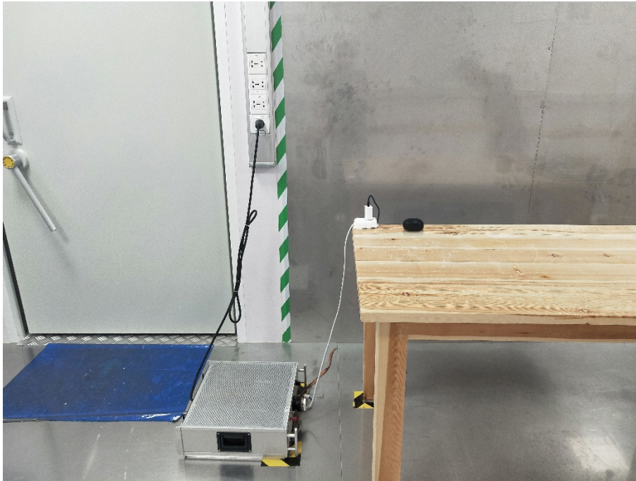
FCC: 2AJQ7ECHO Photo of Conducted Emission Measurement
