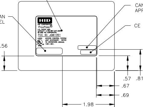
1351 LABEL LOCATION DRAWING
