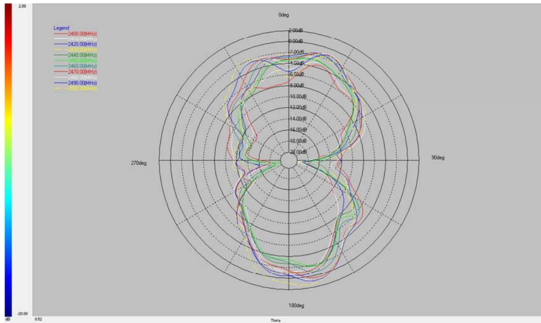
YZ plane ( \Phi = 90^\circ )
