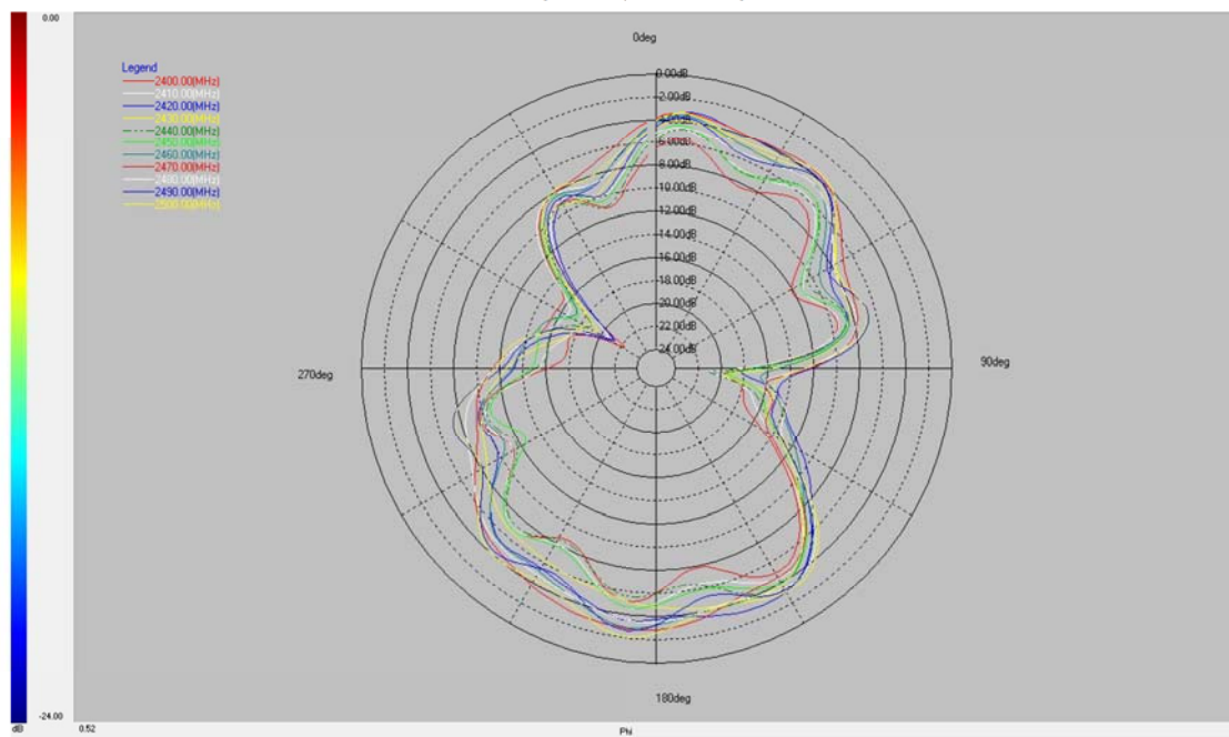
XY plane ( \Theta = 90^\circ )
