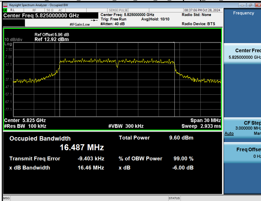
-6dB_Emission_Bandwidth_NVNT_ANT2_802_11n(HT20)_5825_20M
