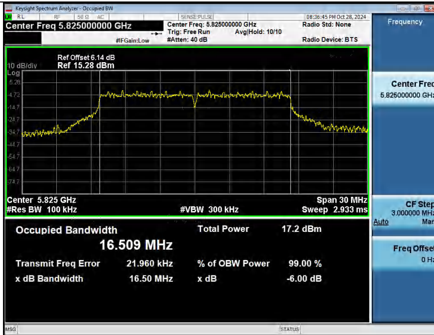
-6dB_Emission_Bandwidth_NVNT_ANT2_802_11n(HT20)_5825_20M
