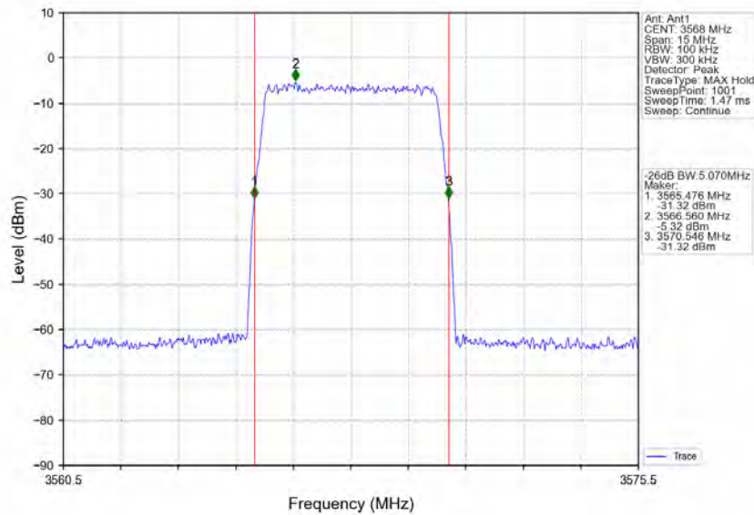
Band48_3568MHz_AWGN_SISO_Ant1_NTNV_Input_AGC+3
