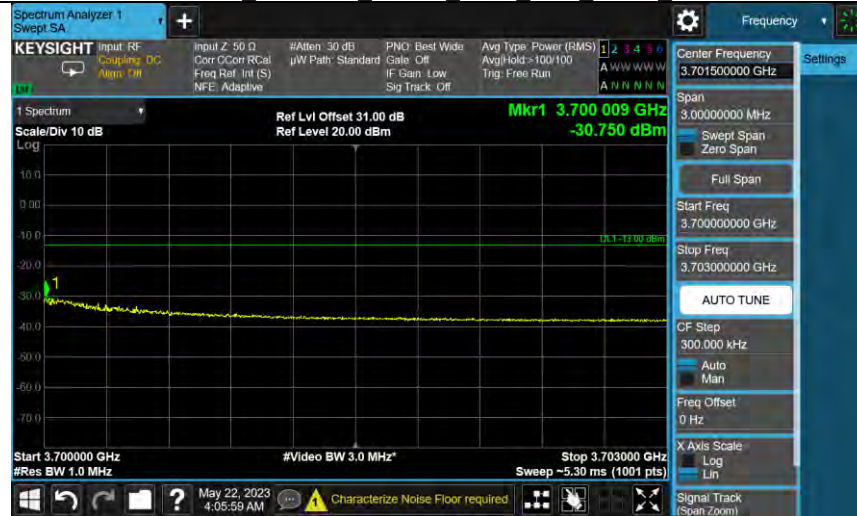
Band48_3650MHz_AWGN_SISO_Ant1_NTNV_AGC+3
