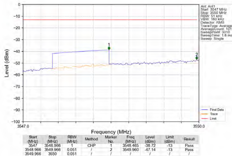
Band48_3552.5MHz_AWGN_SISO_Ant1_NTNV_AGC+3
