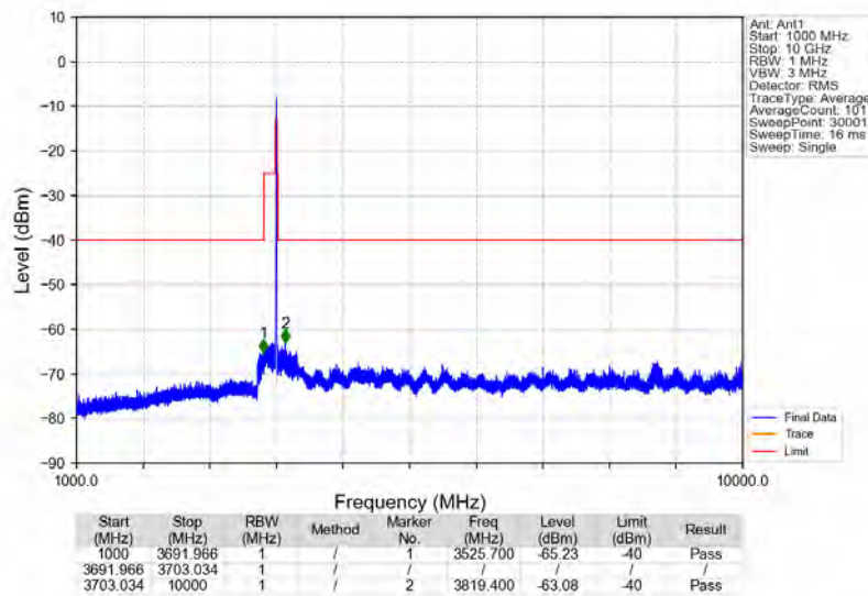
Band48_3697.5MHz_AWGN_SISO_Ant1_NTNV
