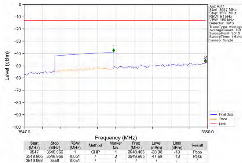
Band48_3552.5MHz_AWGN_SISO_Ant1_NTNV_AGC
