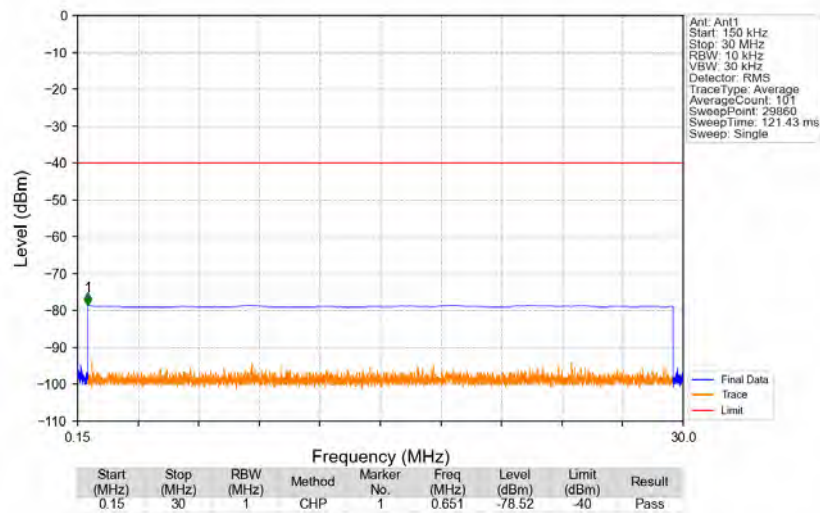
Band48_3697.5MHz_AWGN_SISO_Ant1_NTNV
