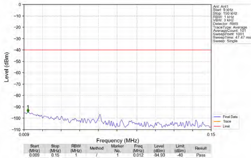
Band48_3697.5MHz_AWGN_SISO_Ant1_NTNV
