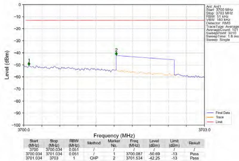
Band48_3697.5MHz_AWGN_SISO_Ant1_NTNV_AGC+3
