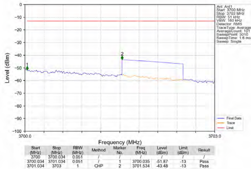
Band48_3697.5MHz_AWGN_SISO_Ant1_NTNV_AGC
