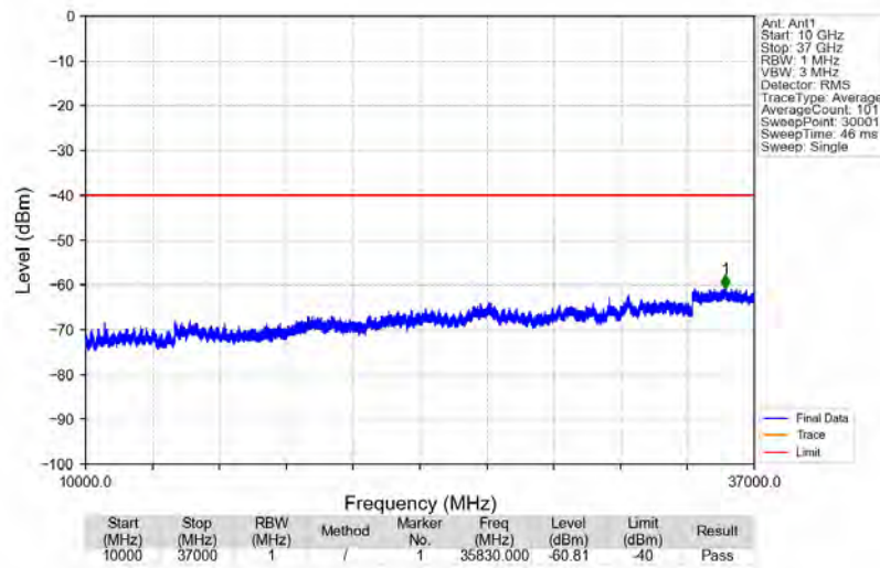
Band48_3697.5MHz_AWGN_SISO_Ant1_NTNV
