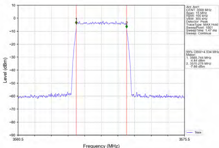
Band48_3568MHz_AWGN_SISO_Ant1_NTNV_Input_AGC+3
