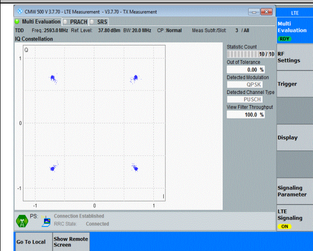
Band41-20MHz-QPSK-40620-100RB#0-PASS
