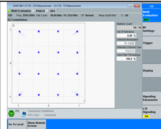
Band38-20MHz-16QAM-38000-100RB#0-PASS
