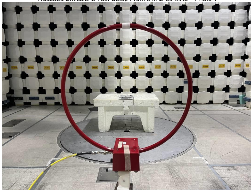
Radiated Emissions Test Setup From 9 kHz-30 MHz – Photo 1
