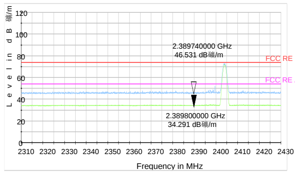
Bluetooth LE Channel 0 Peak &amp; Average
