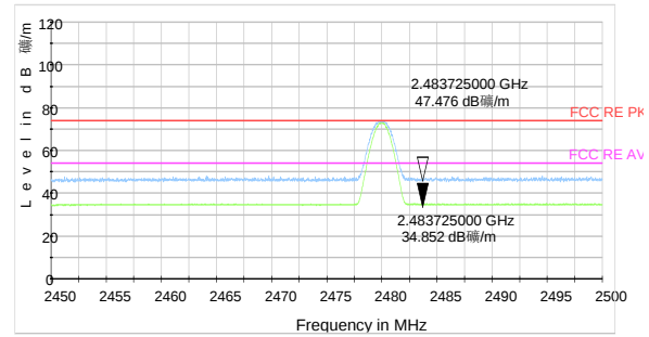
Bluetooth LE Channel 39 Peak &amp; Average
