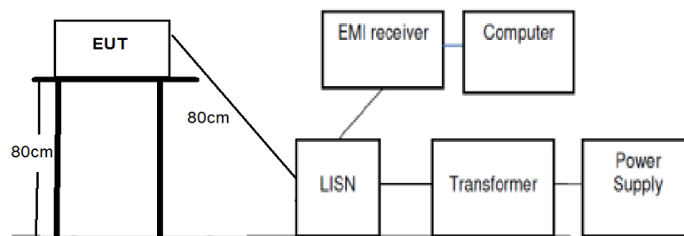
(Conducted emission)
