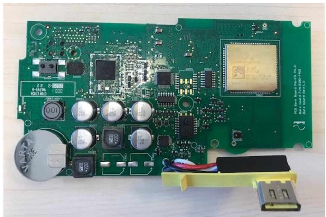
PCBA Bottom View
