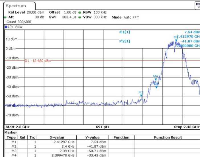
11B_Low bandedge
