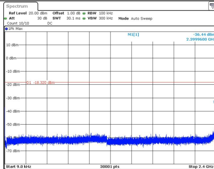
11G_2412_0.009~2400
