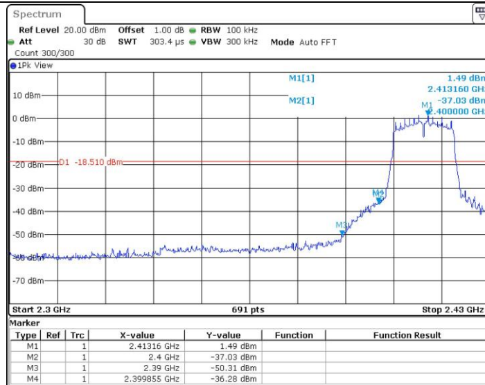
11G_low bandedge
