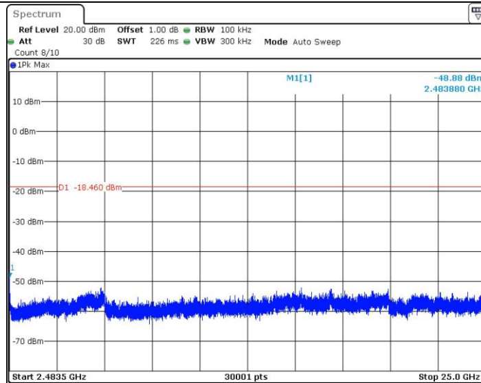
11N20_2462_2483.5~25000
