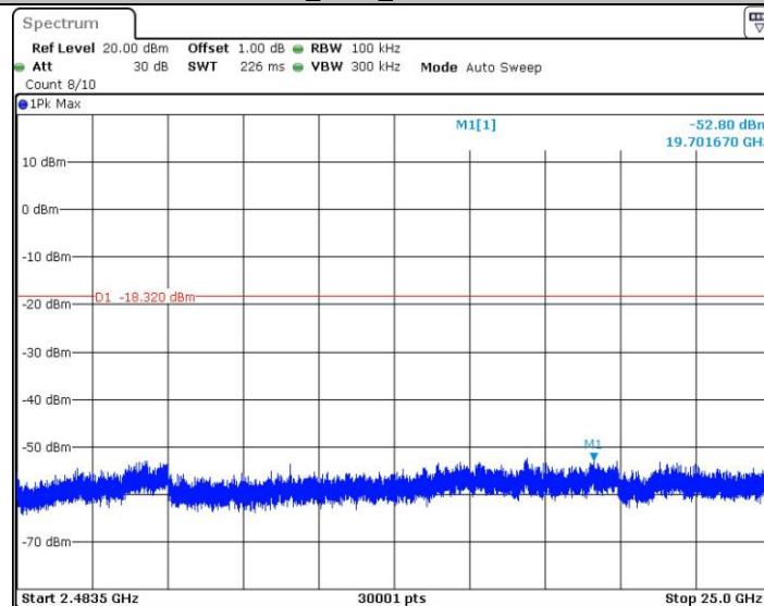
11G_2412_2483.5~25000
