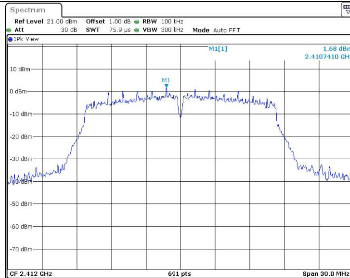
11G_2412_0~Reference
