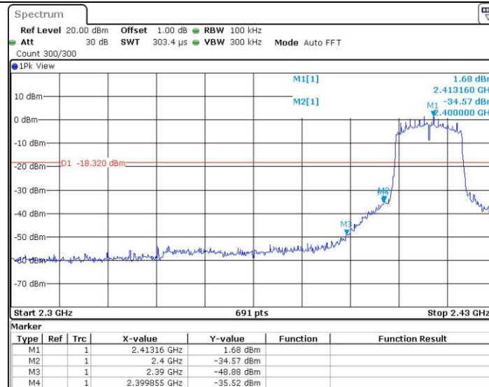
11N20_low bandedge
