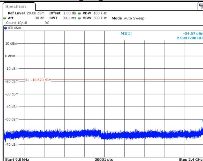
11G_2437_0.009~2400
