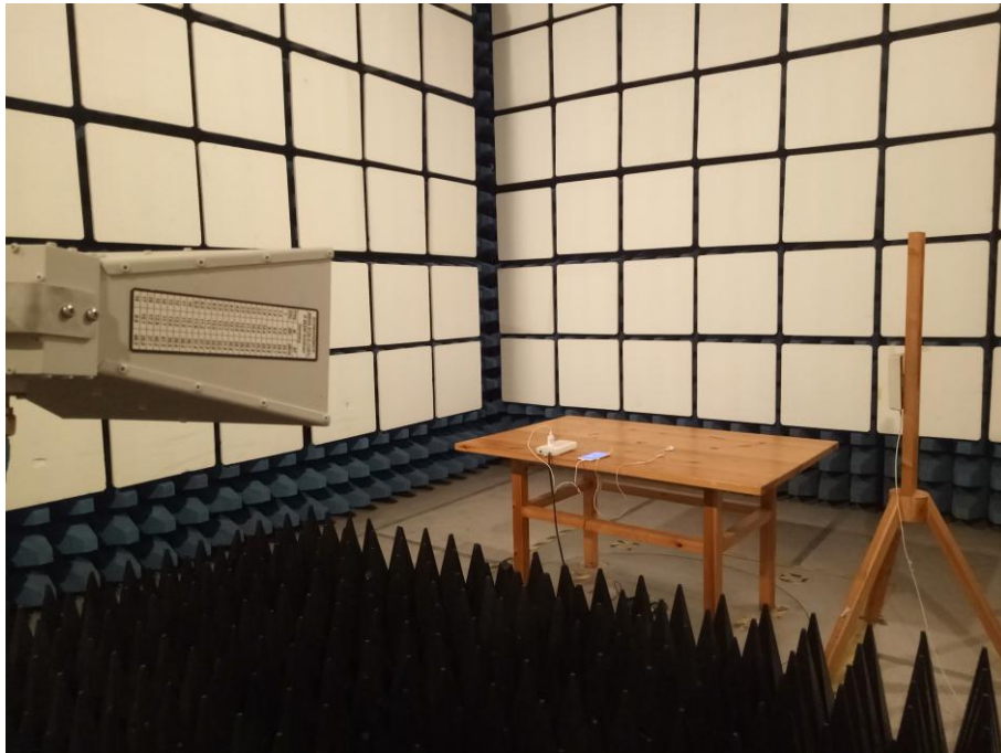
Above 1 GHz (The GSM 850 Test Mode)
