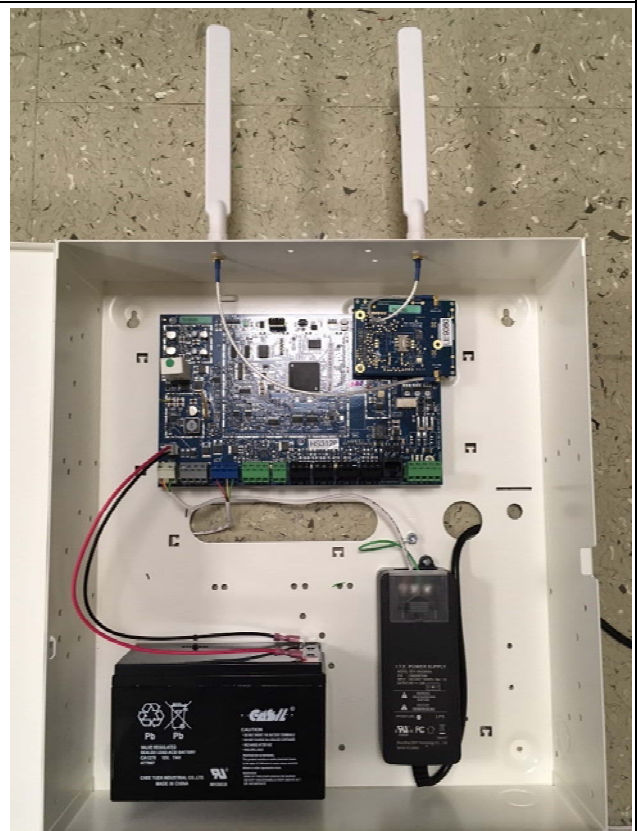
Host – With Battery
