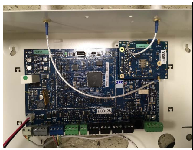
Host - Cover-off View 2
